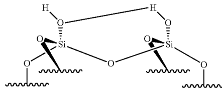
Chemical Structure #10
