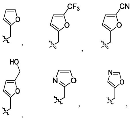
Ring A
