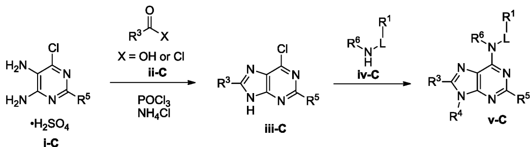
Scheme III.
