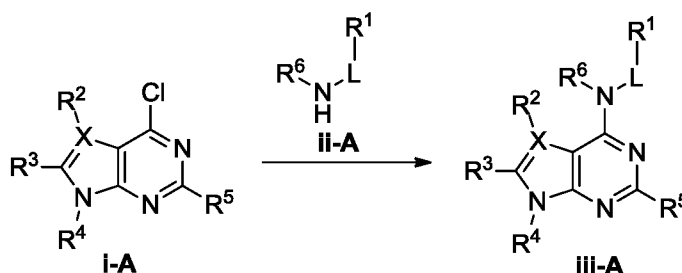
Scheme I
