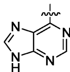
Ring A
