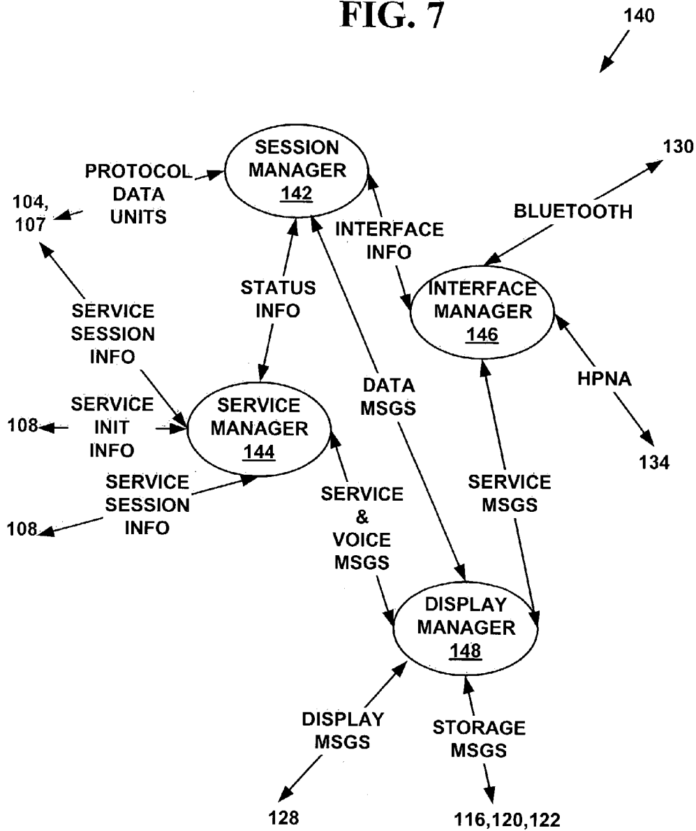
INTEGRATED PHONE-BASED HOME GATEWAY INTERFACE SOFTWARE ARCHITECTURE
