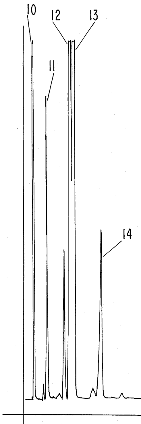
GLC PROFILE FOR EXAMPLE I(A).
