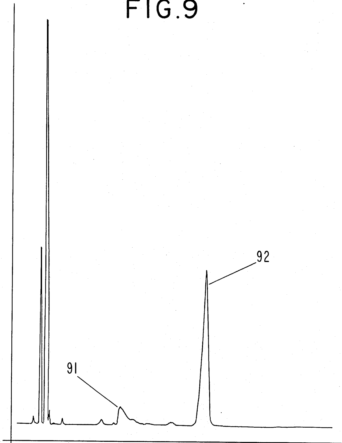
GLC PROFILE FOR EXAMPLE III.
