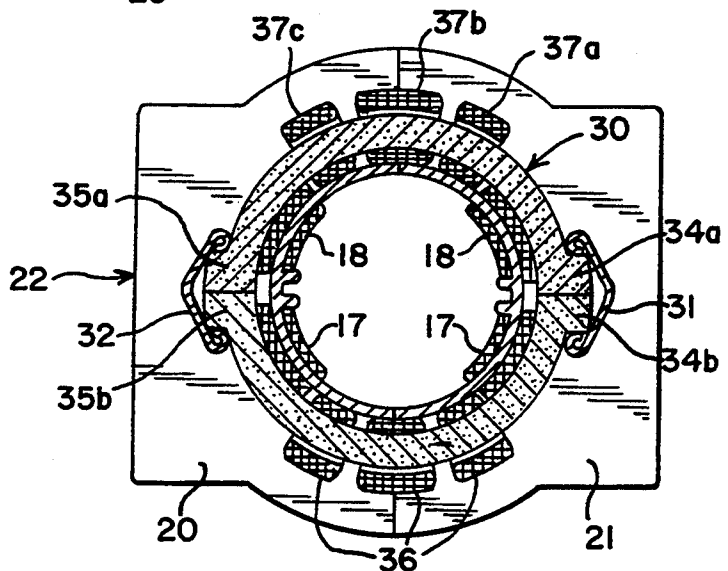
FIG. 3 PRIOR ART
