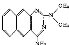
2-dimethylamino-4-amino-6,7-benzoquinazoline
