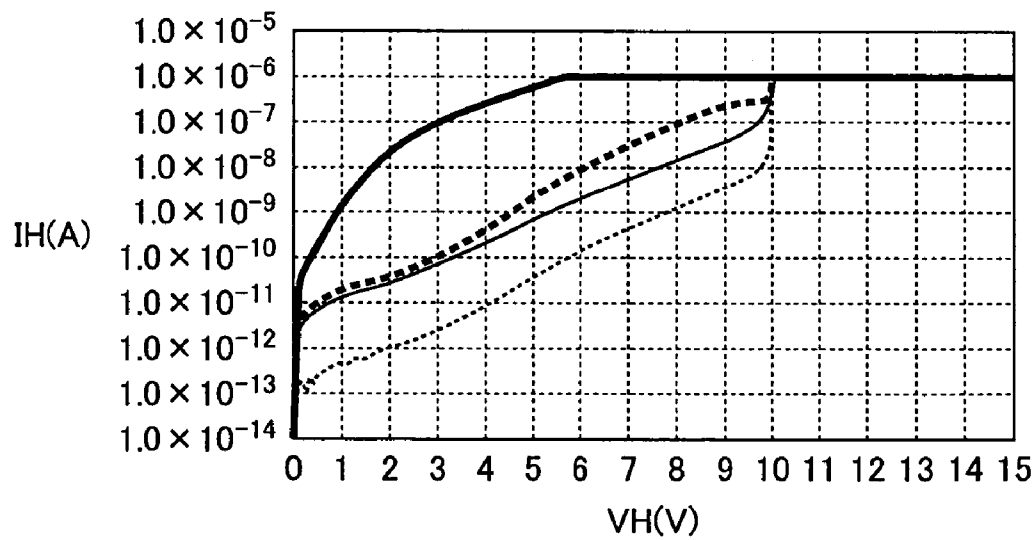
FIG.11 PRIOR ART
