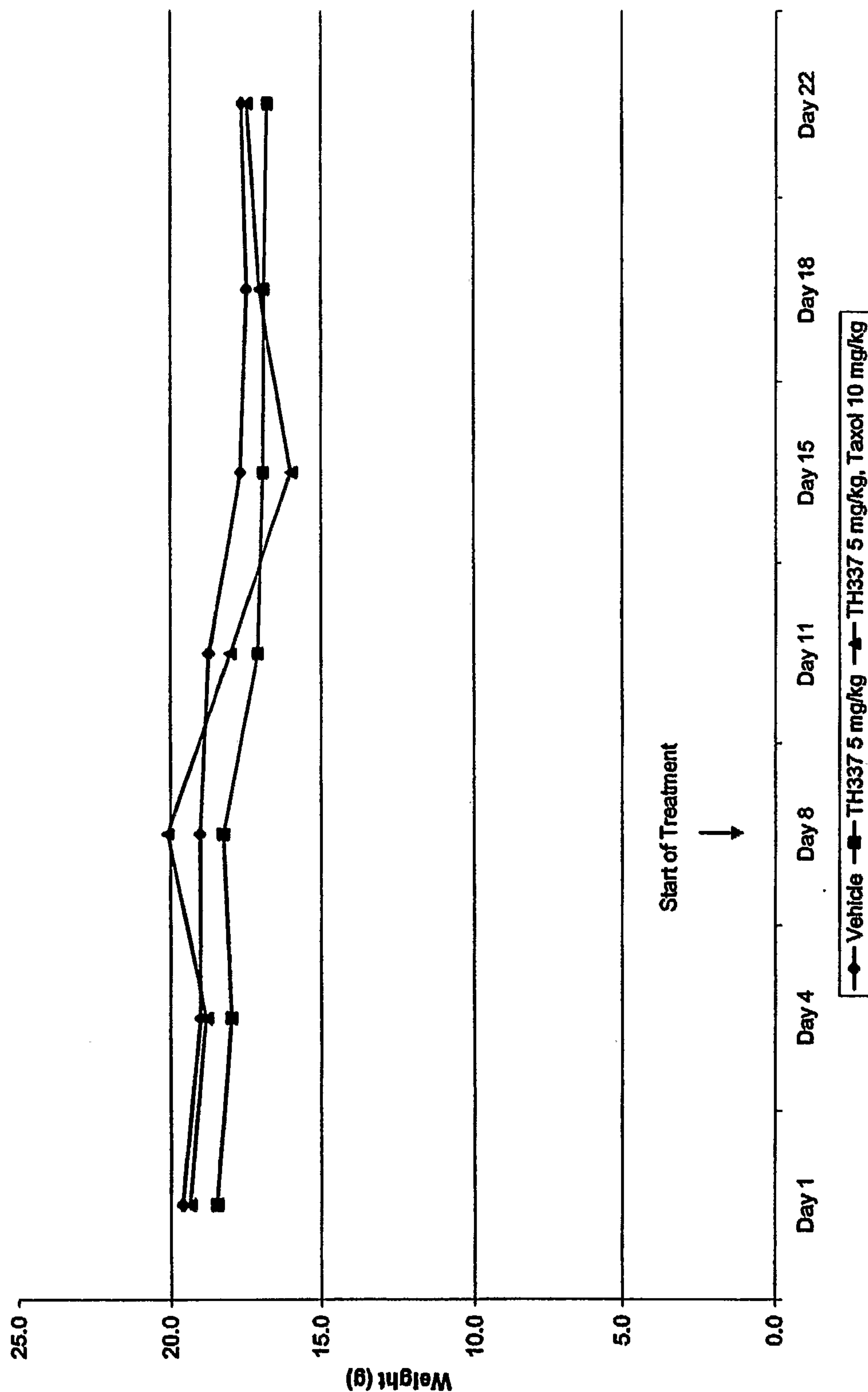
Figure 1 Body Weights, Day 1-14
