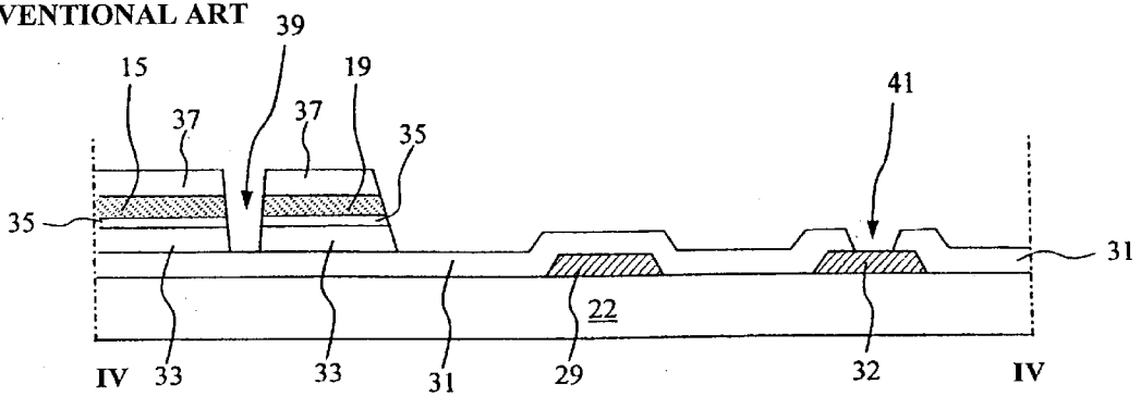
FIG. 4C CONVENTIONAL ART
