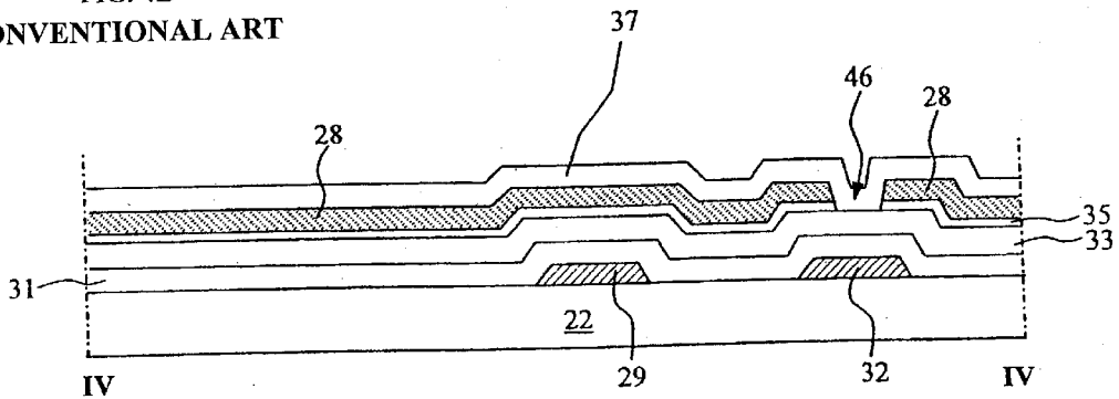
FIG. 4C CONVENTIONAL ART
