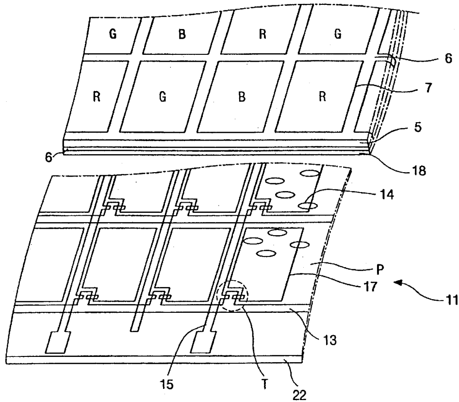
FIG.1 CONVENTIONAL ART
