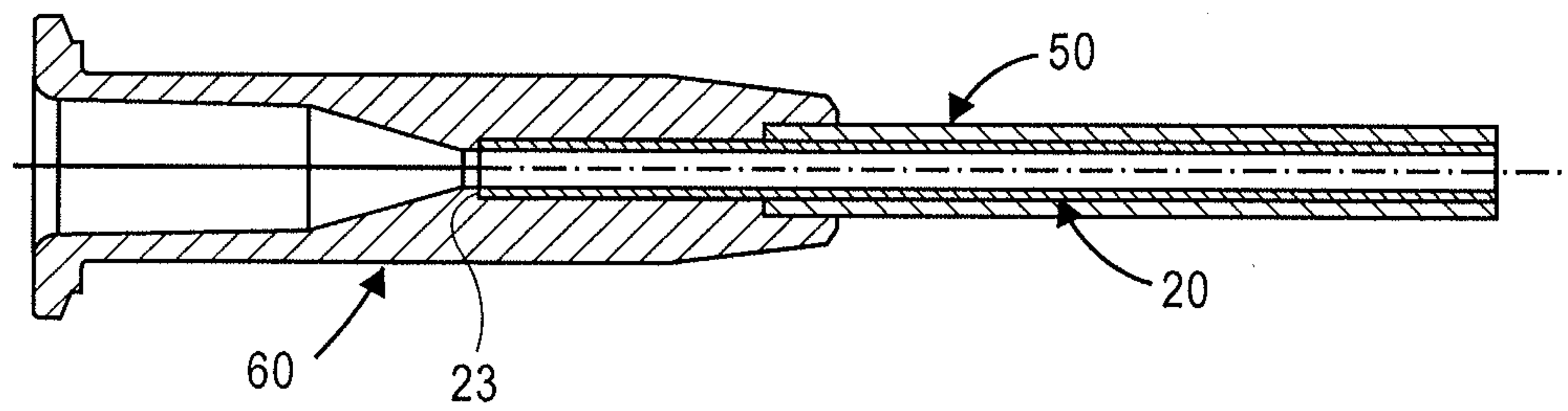
SECTION A - A
