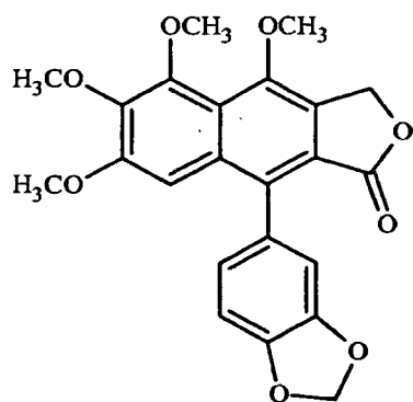
3: 5-Methoxyjusticidin A
