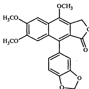
4: Justicidin A
