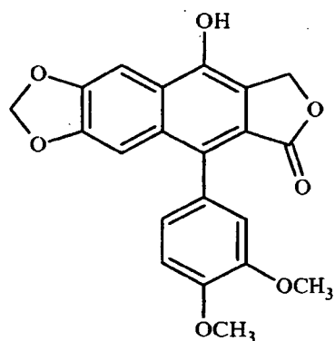
5: Chinensinaphthol
