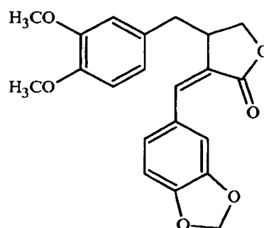
6: Suchilactone
