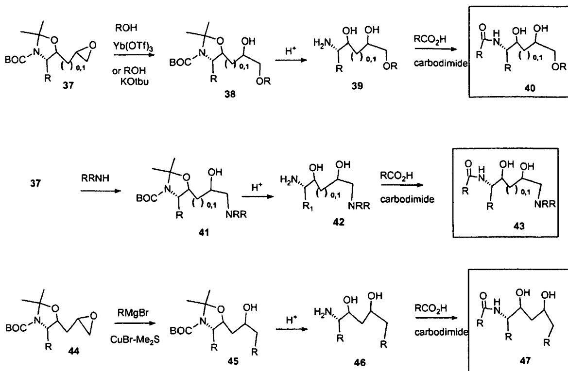
Scheme 6.
