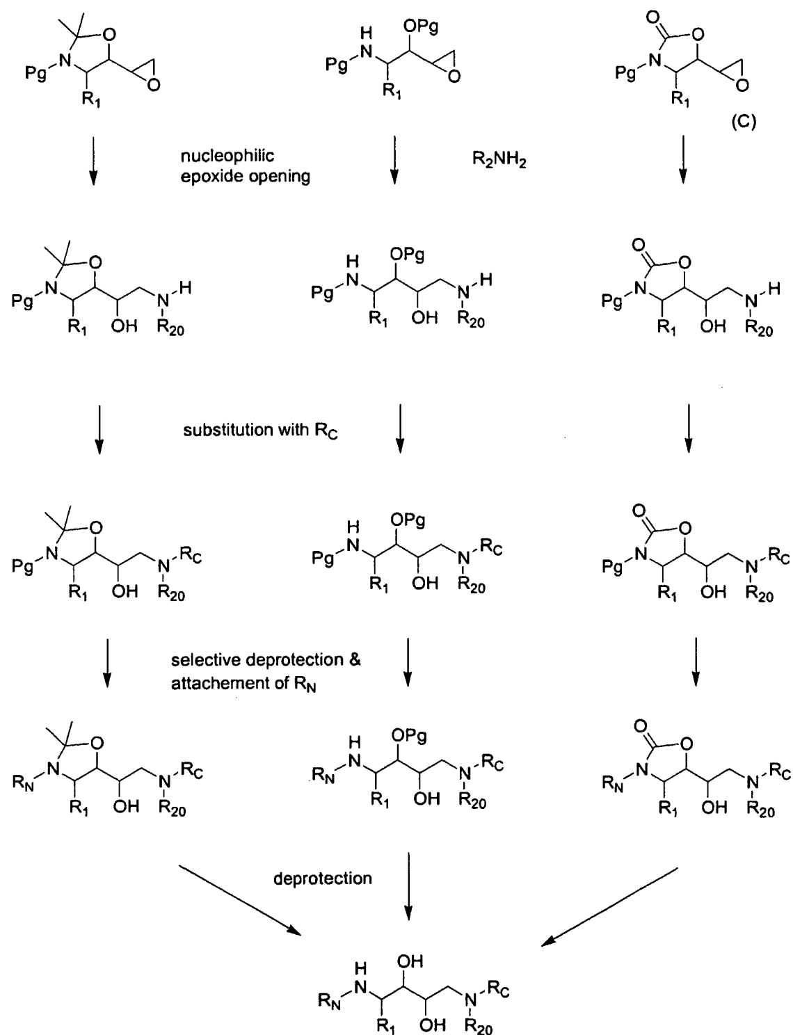
Scheme V
