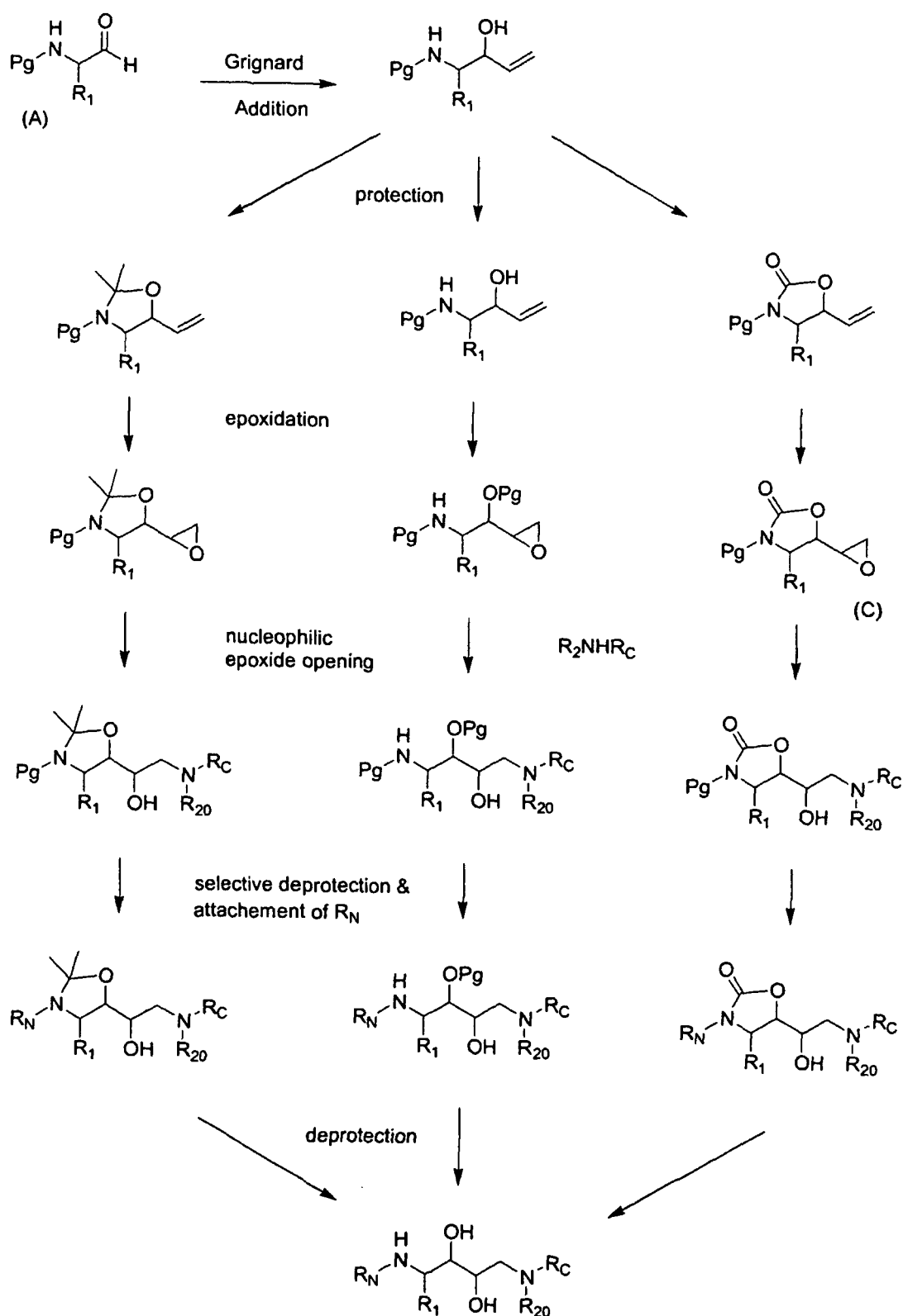
Scheme III
