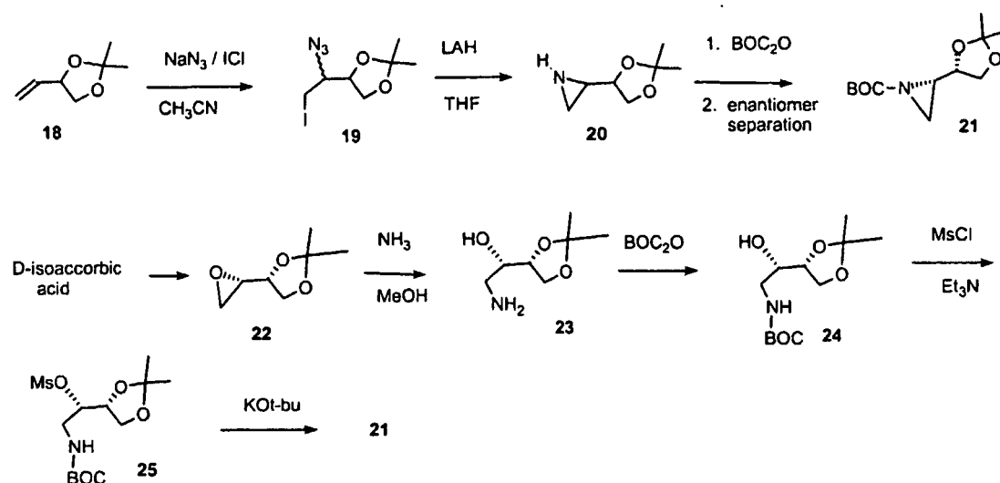
Scheme 4: Preparation of enantiomerically pure aziridine intermediate
