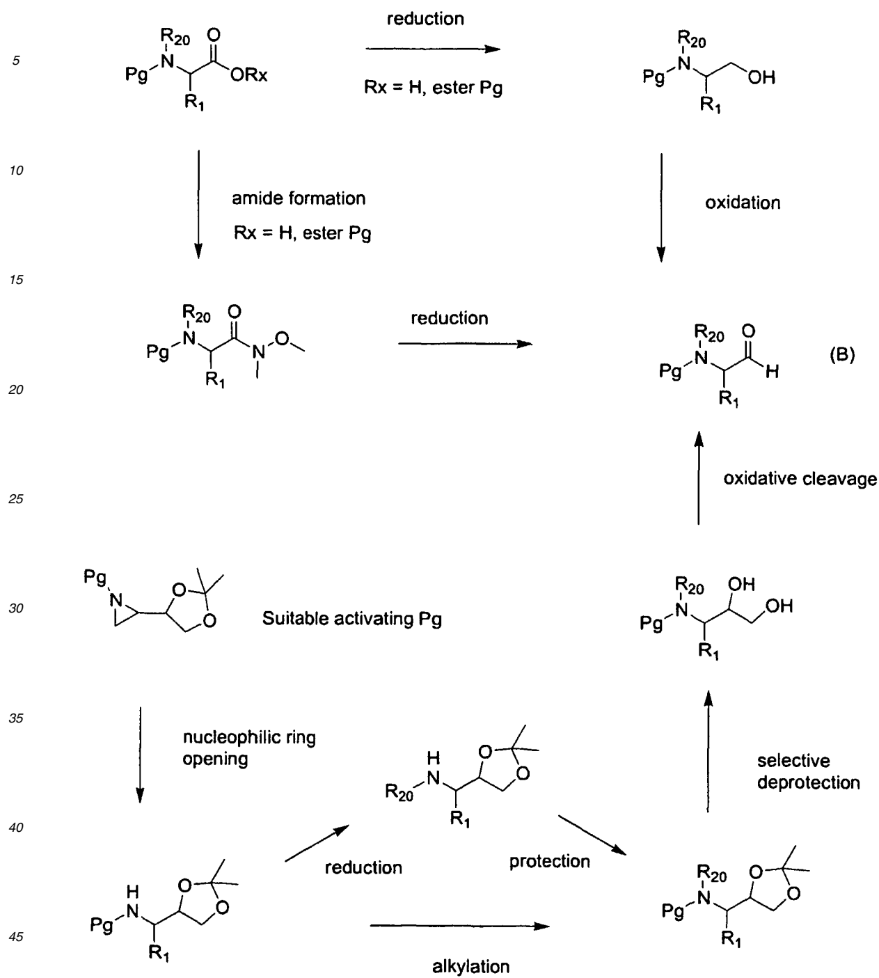
Scheme II
