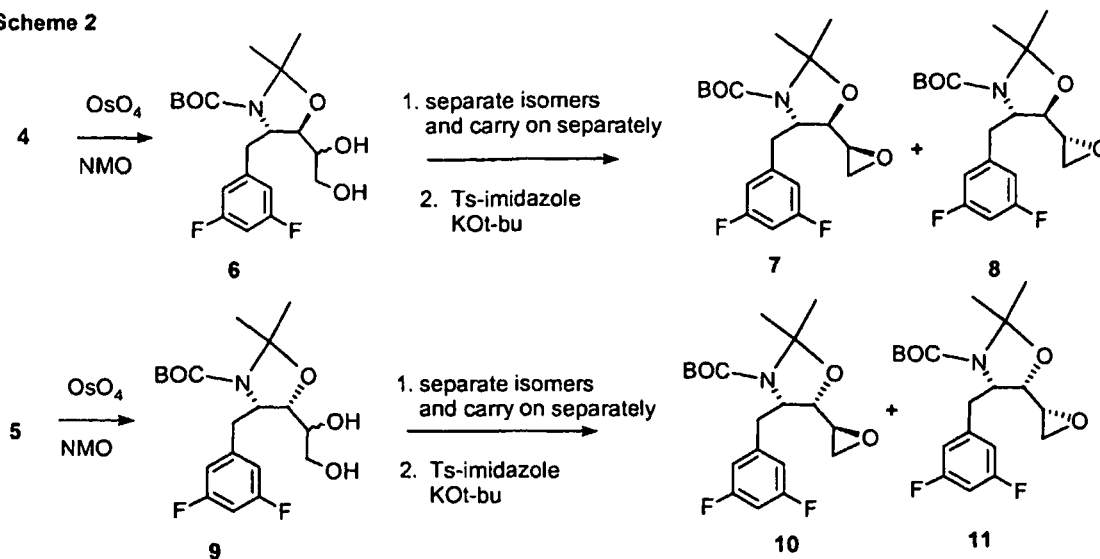
Scheme 2
