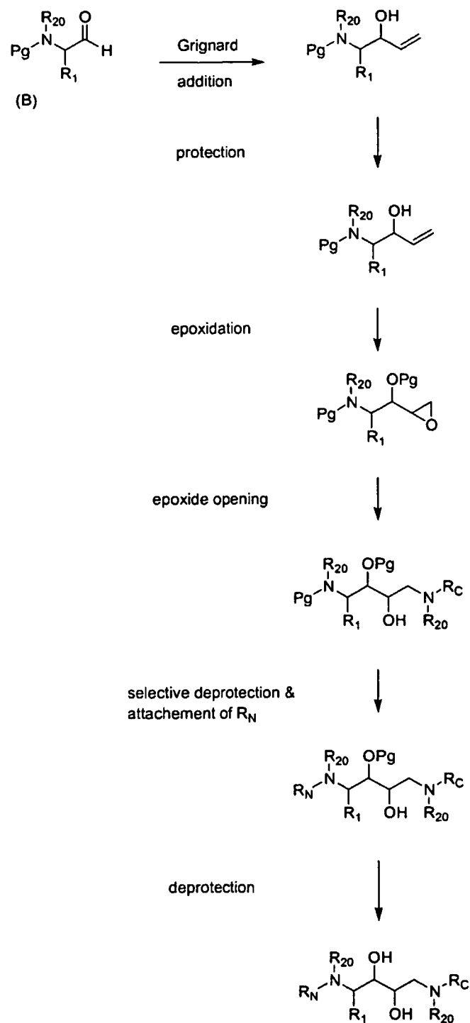
Scheme IV
