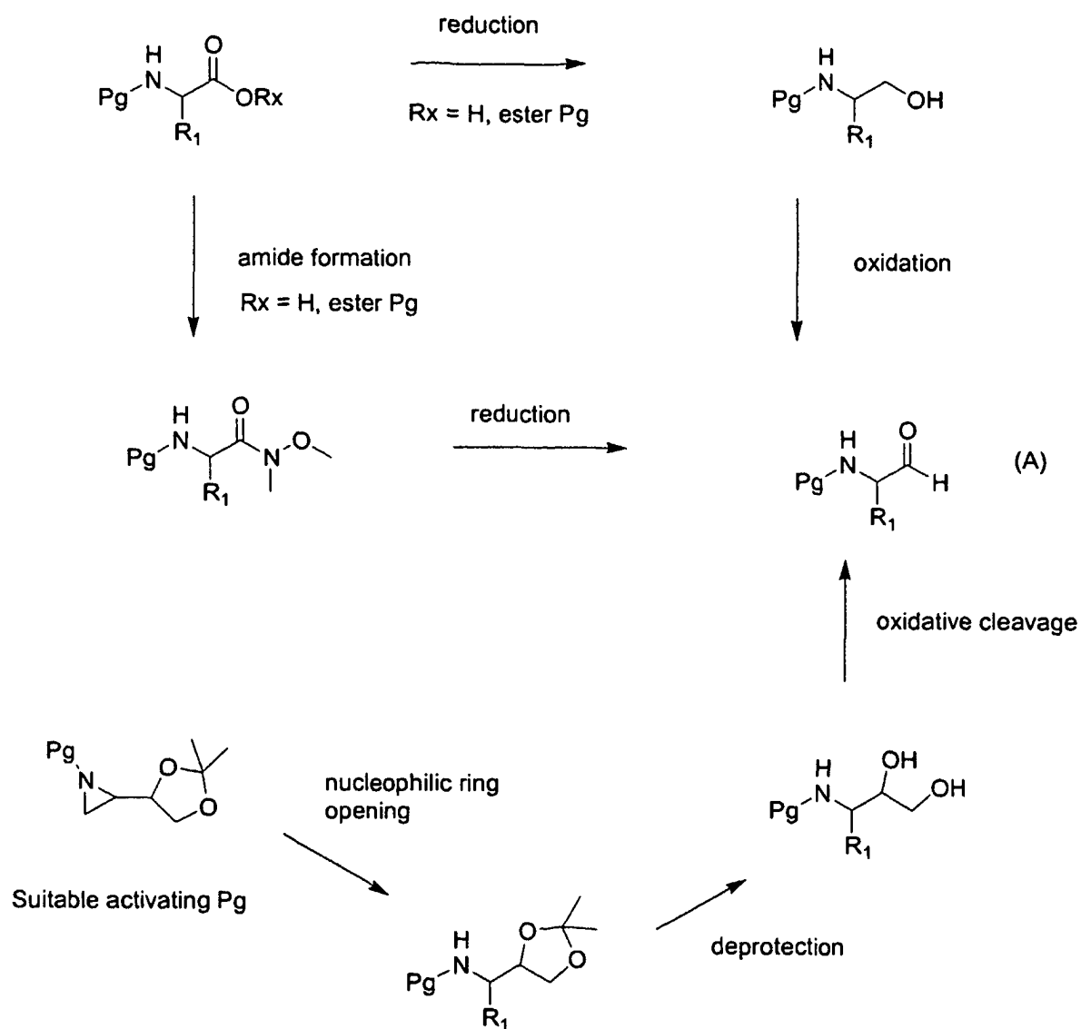
Scheme I
