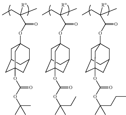
(Chemical formula 26)
