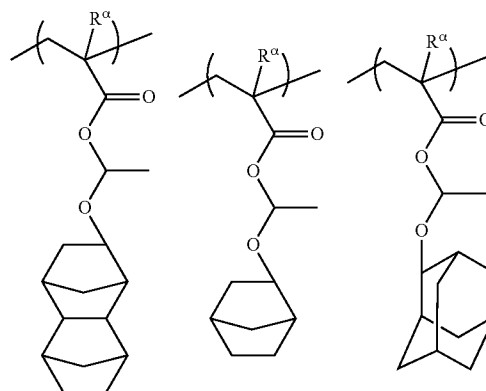
(Chemical formula 22)
