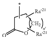
(Chemical formula 4)
