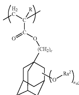
(Chemical formula 21)
