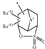
(Chemical formula 6)
