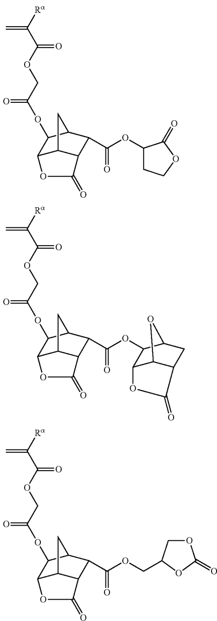
(Chemical formula 13)
