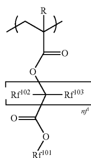
(Chemical formula 47)
