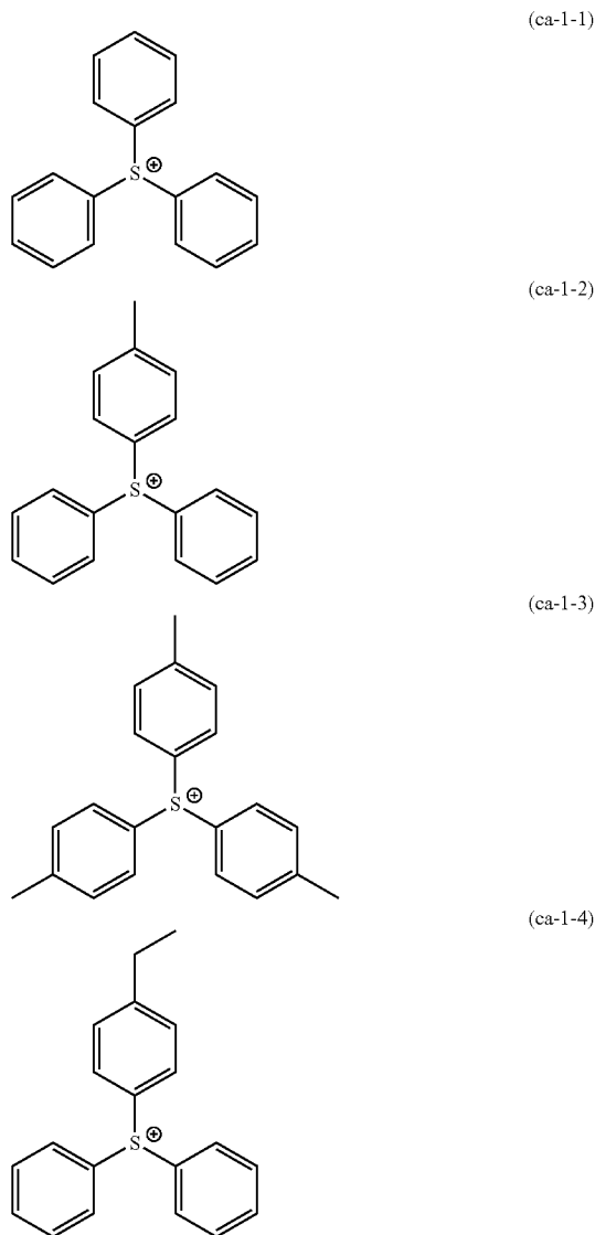
(Chemical formula 36)
