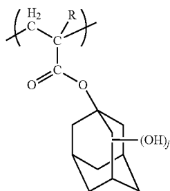
(Chemical formula 28)
