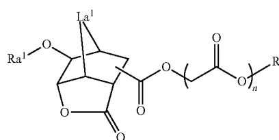
(Chemical formula 3)
