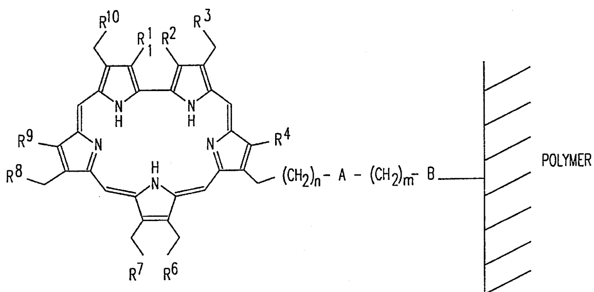
GENERAL STRUCTURE VI
