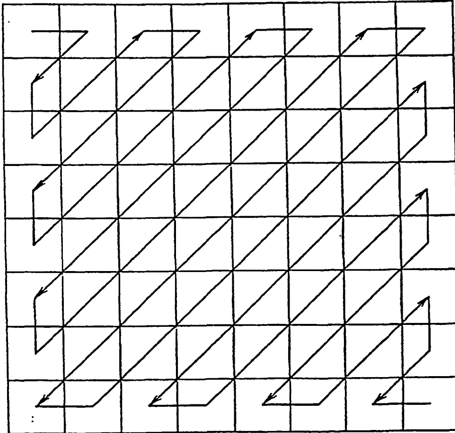
8 × 8 DCT COEFFICIENTS
