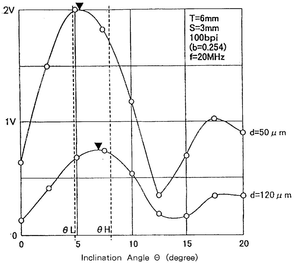
Terminal Voltage of MI Element
