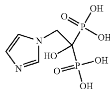
Zoledronic acid
