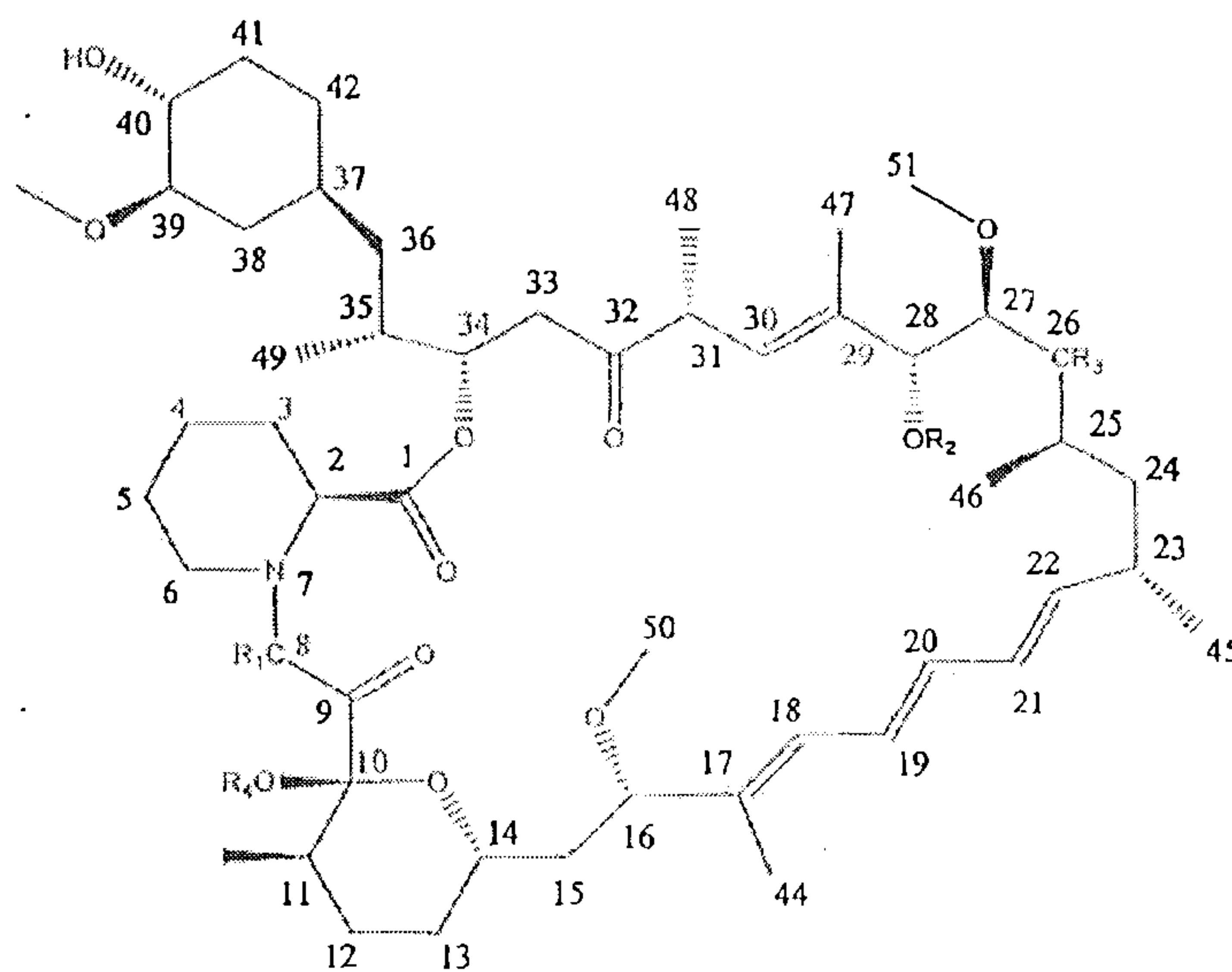
Formula II
