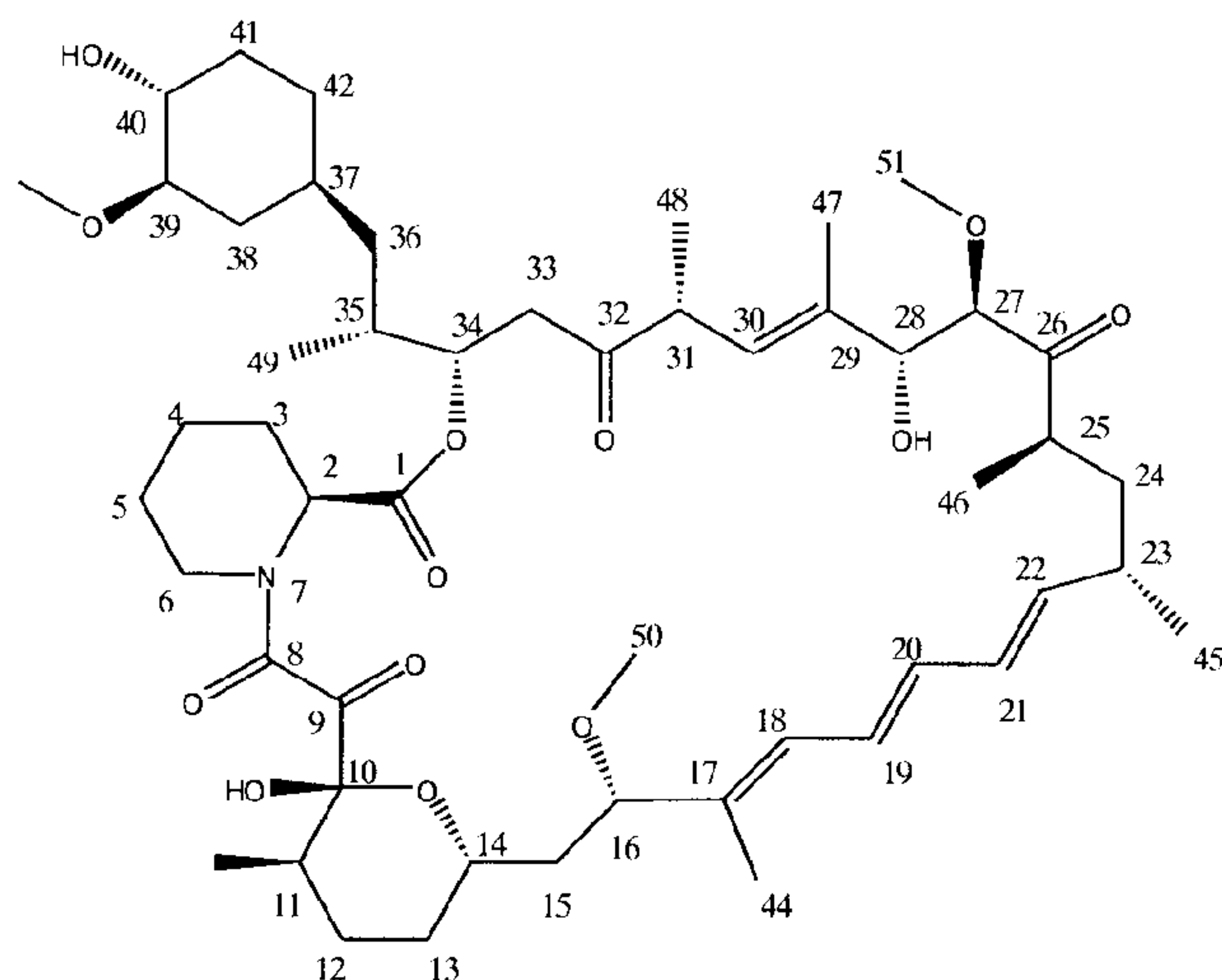
(Formula VI)
