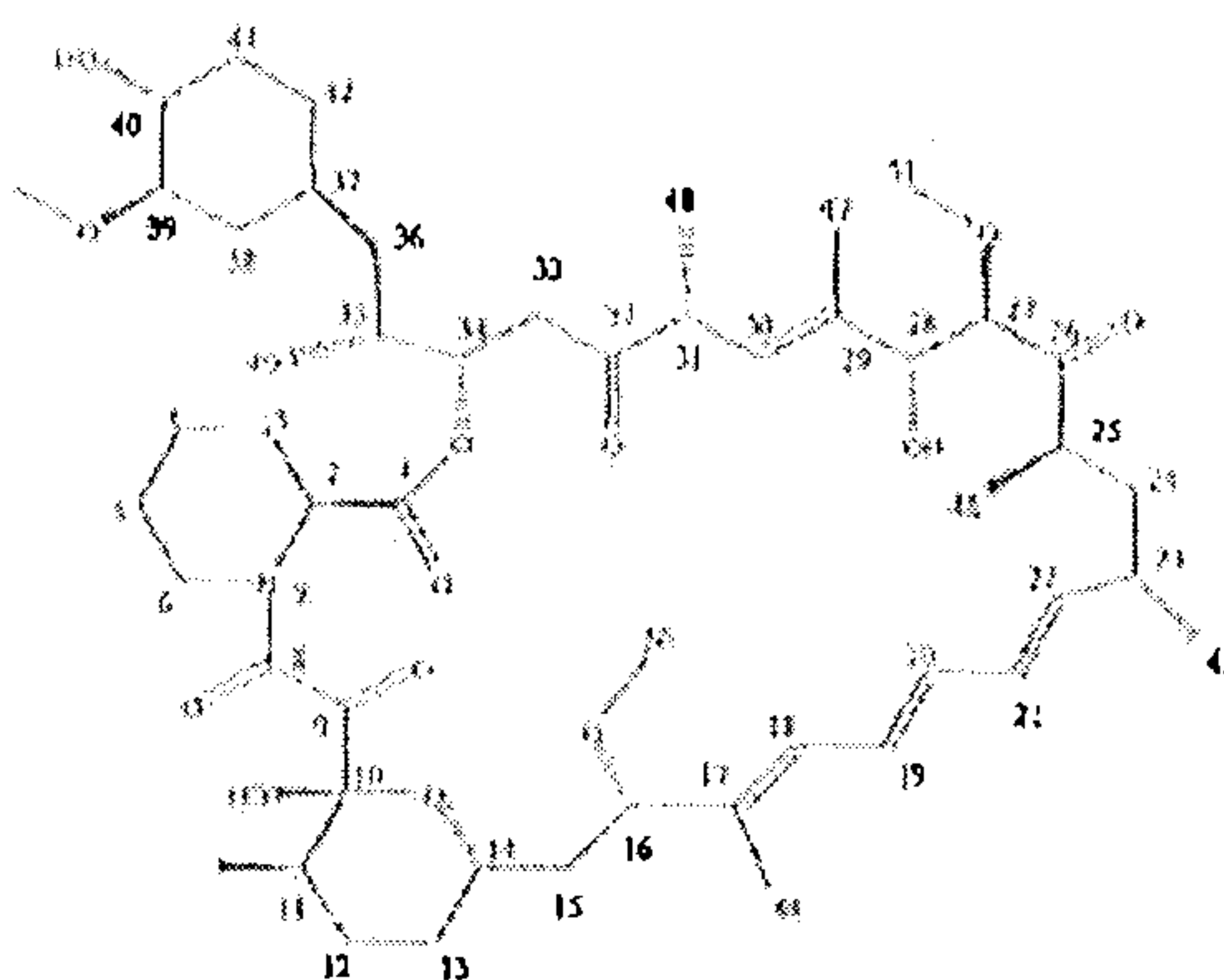
Formula VI
