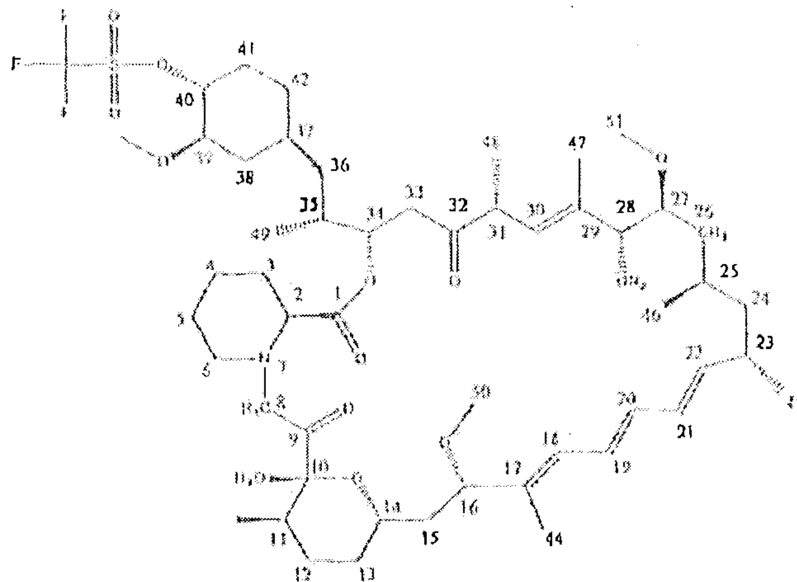
Formula III
