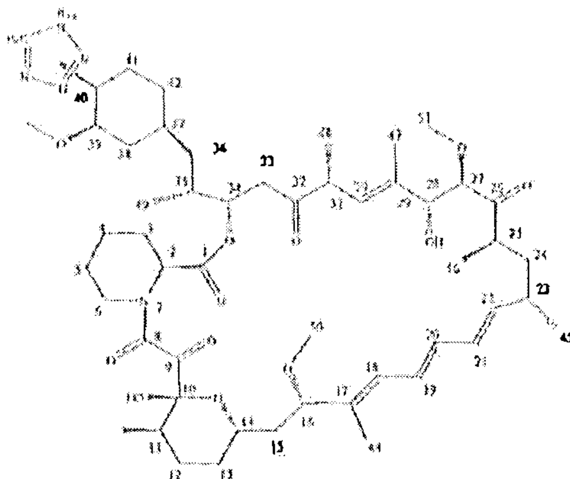
Formula V
