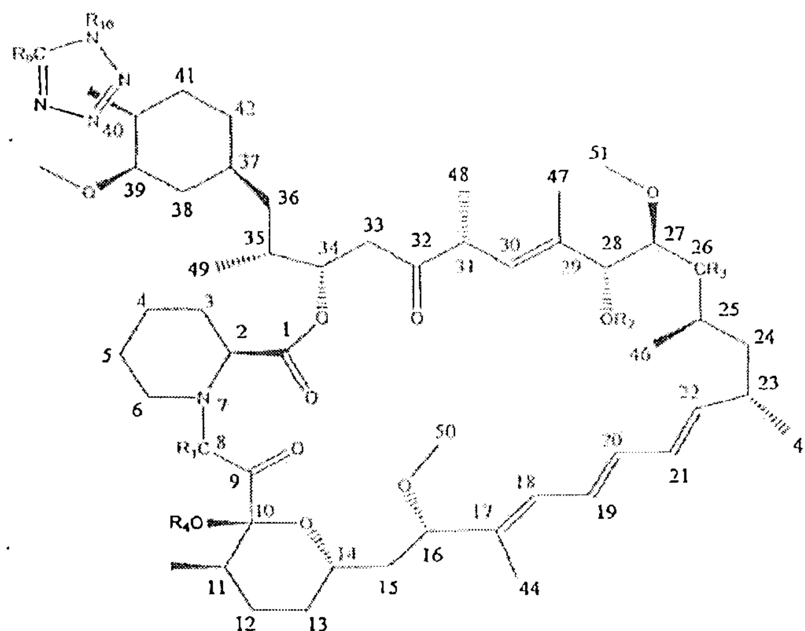
Formula I
