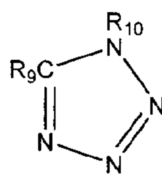
(Formula IV)
