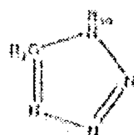
Formula IV
