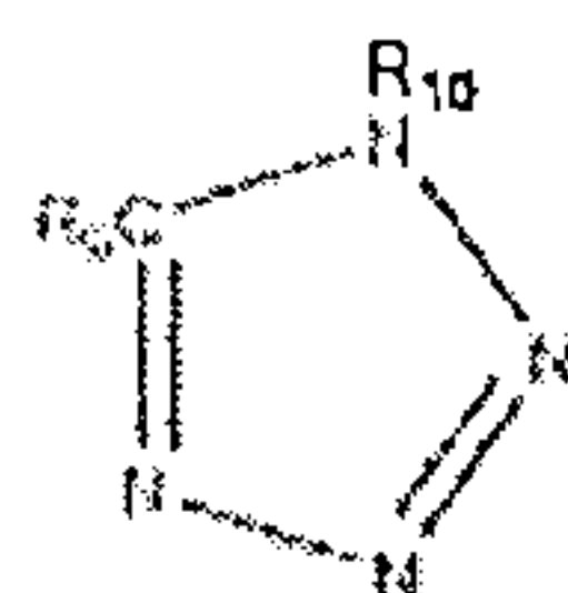
Formula IV
