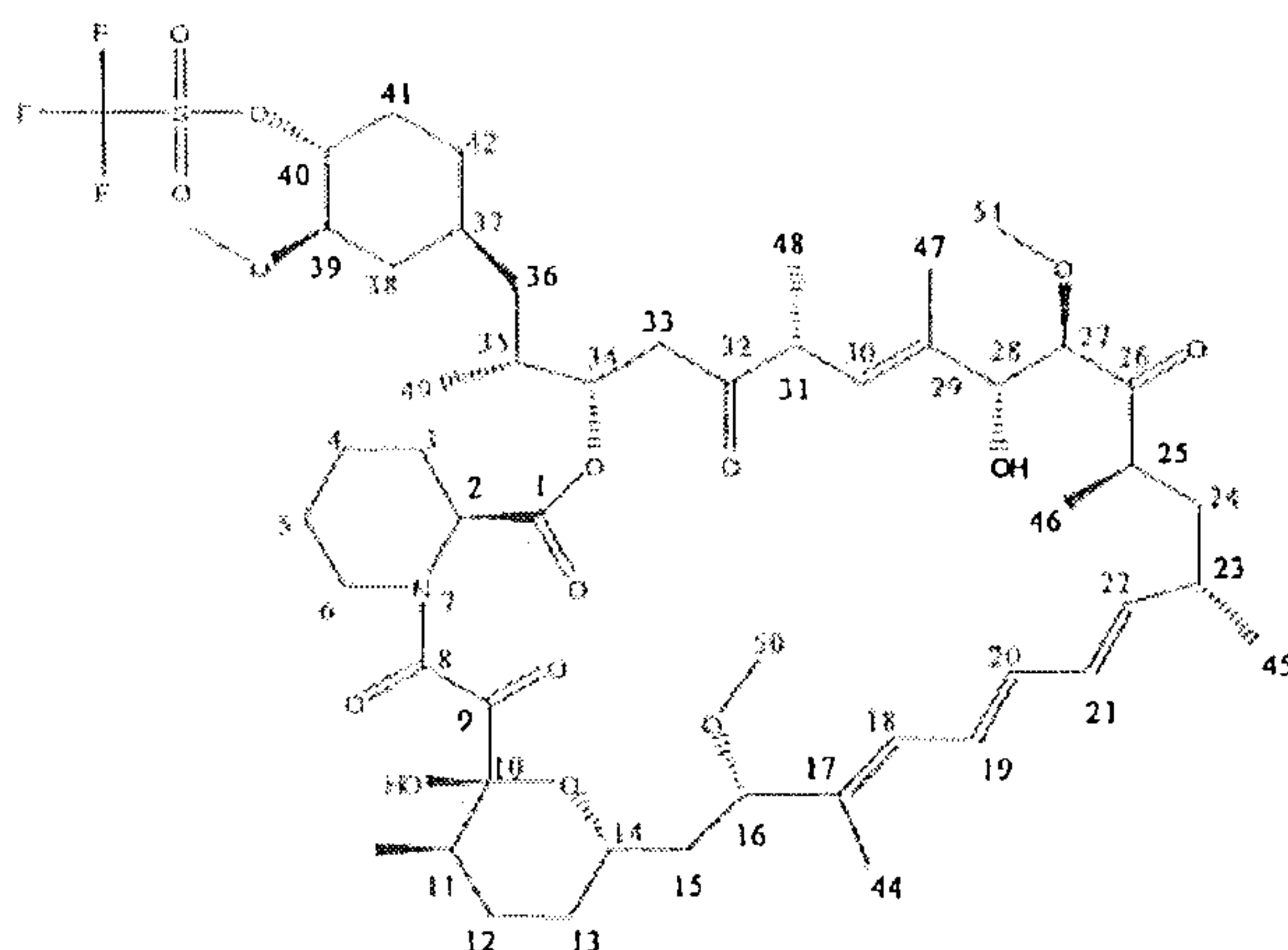
Formula VII
