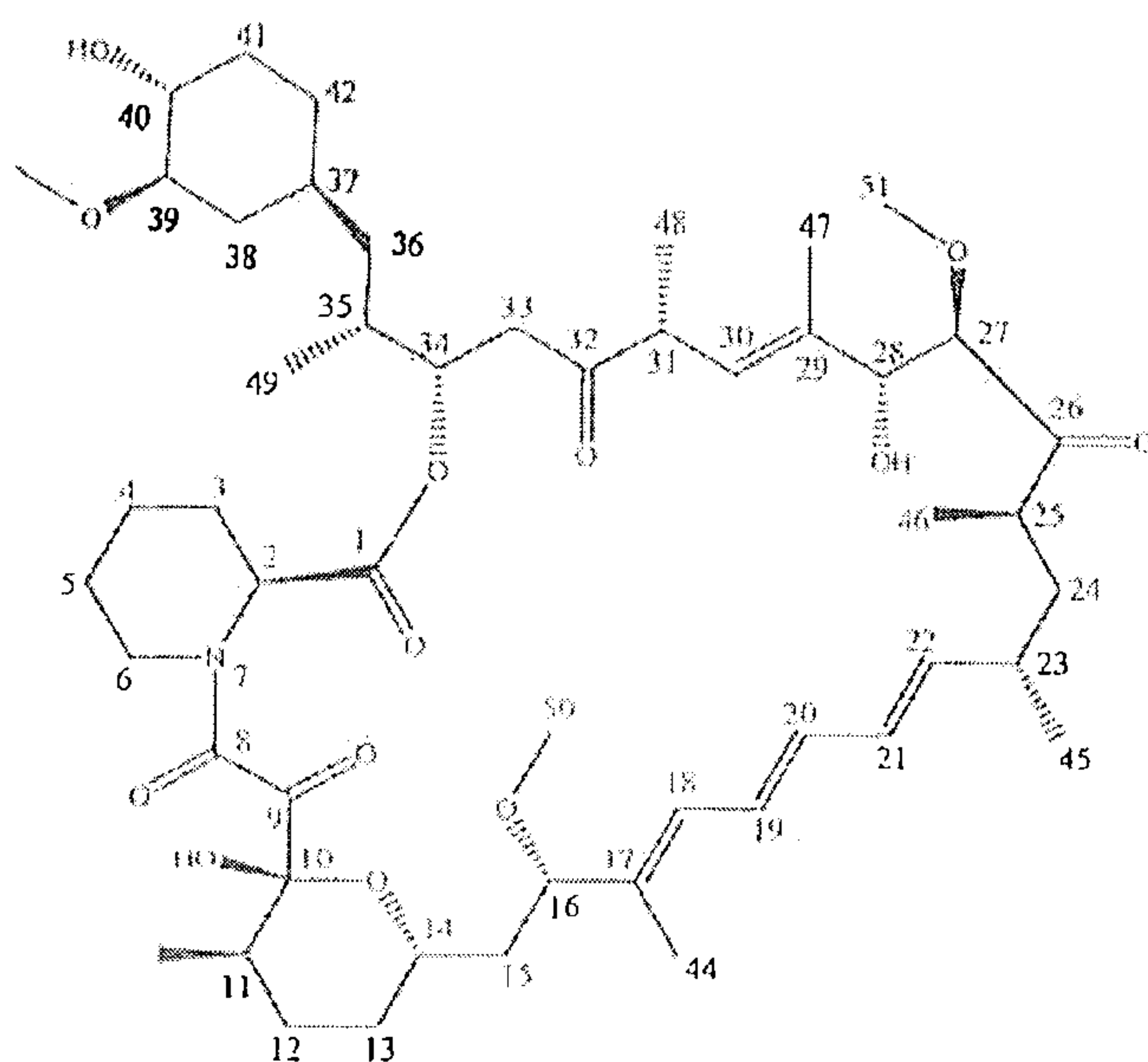
Sirolimus (rapamycin)
