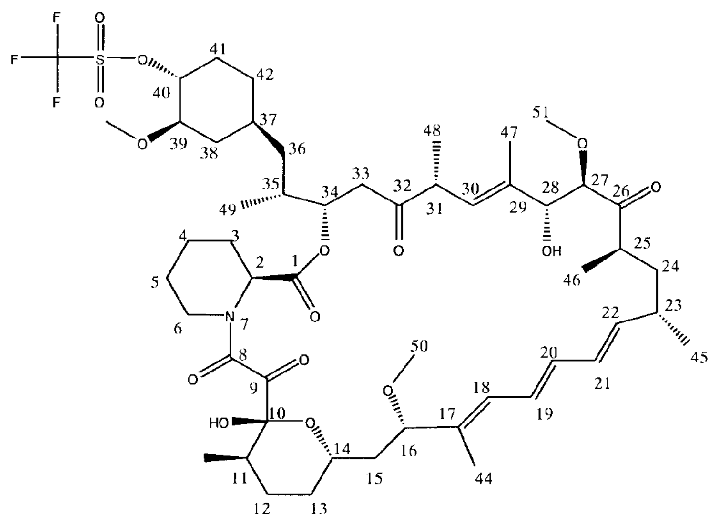
(Formula VII)
