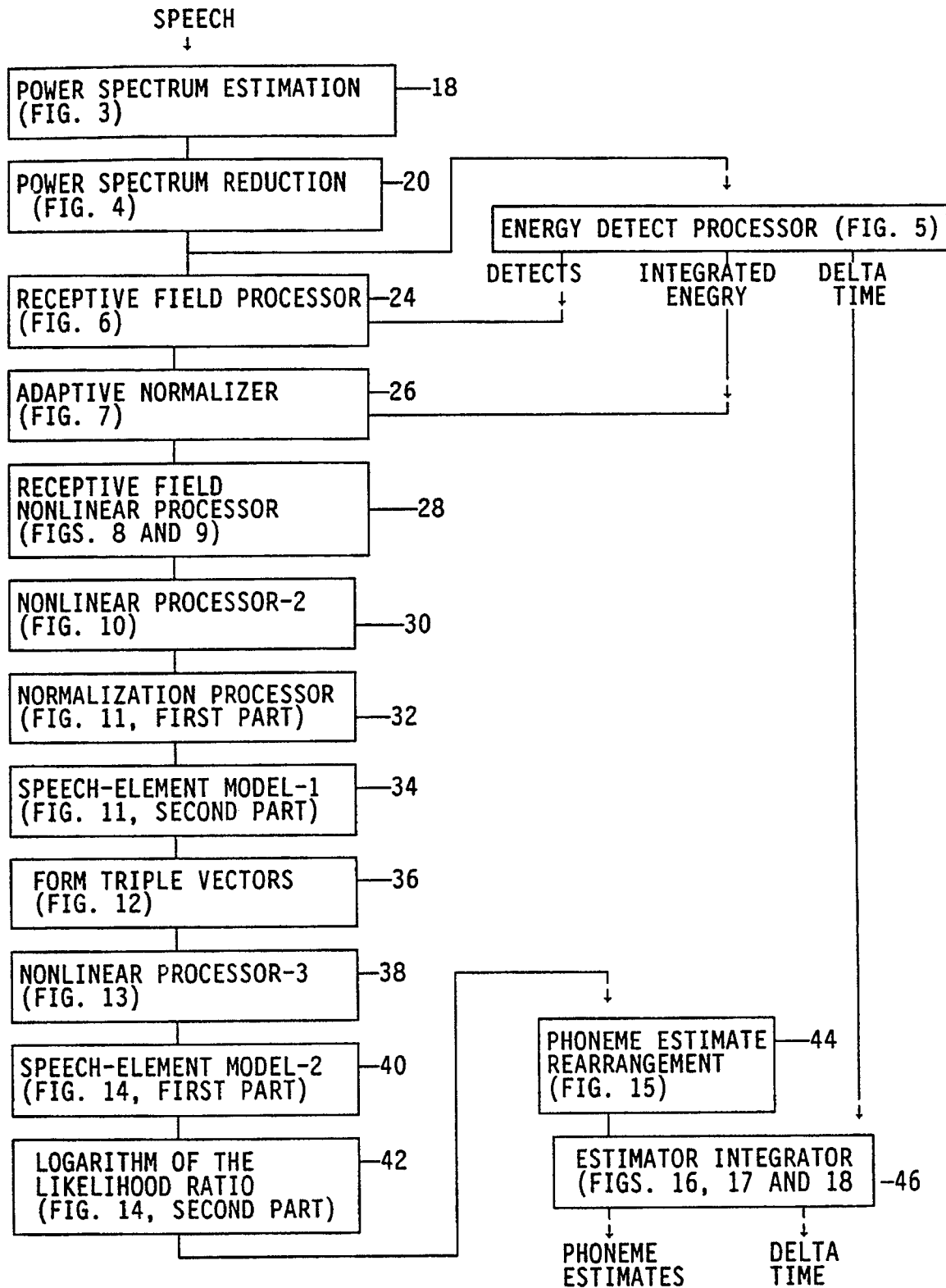
FIG. 2 OVERVIEW OF THE PHONEME ESTIMATOR
