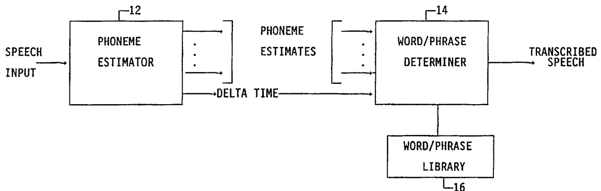
FIG. 1 OVERVIEW OF SPEECH RECOGNITION SYSTEM
