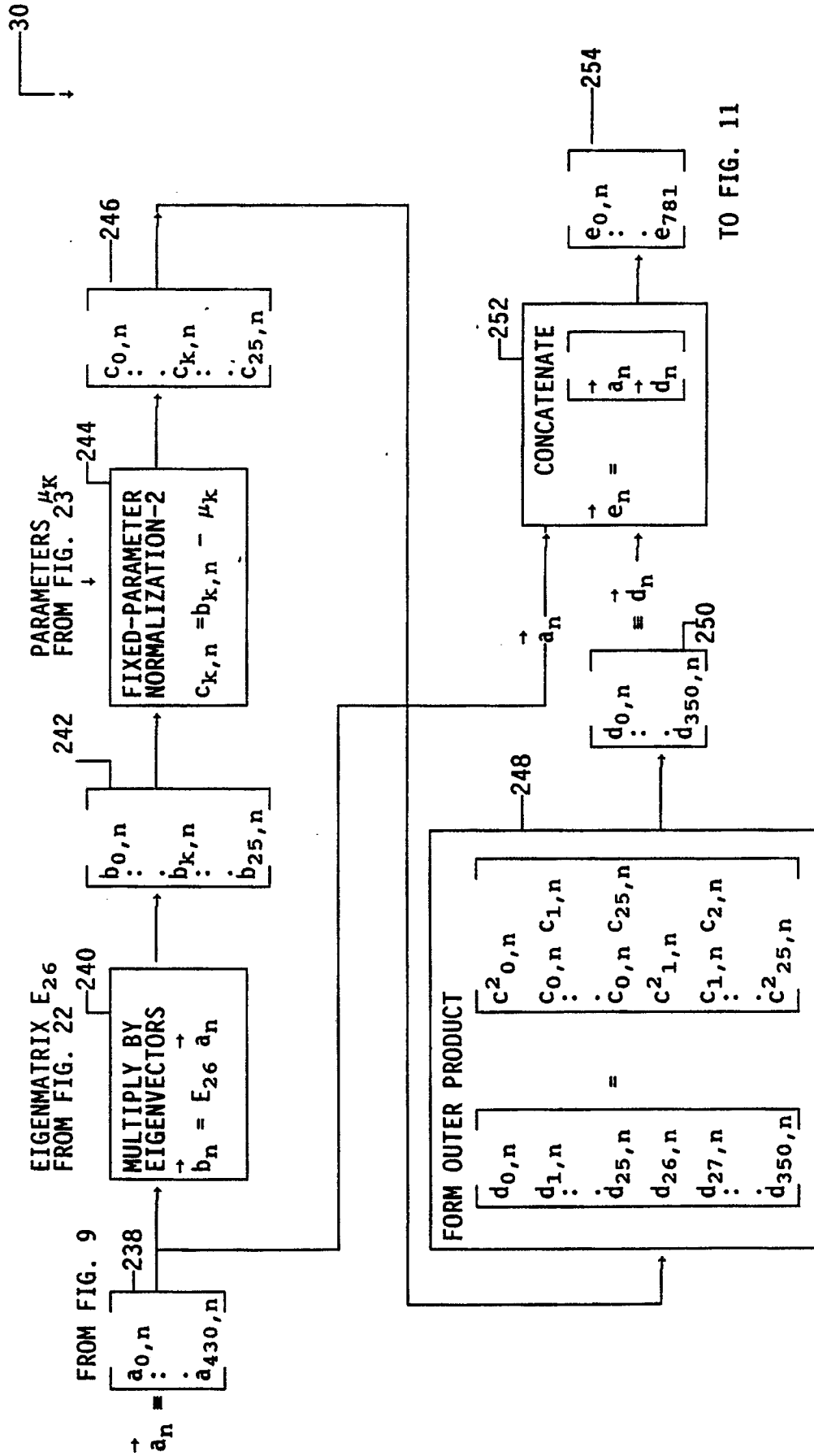
FIG. 10 NONLINEAR PROCESSOR-2
