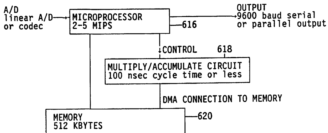
FIG. 47 PHONEME ESTIMATOR HARDWARE CONFIGURATION-3.
