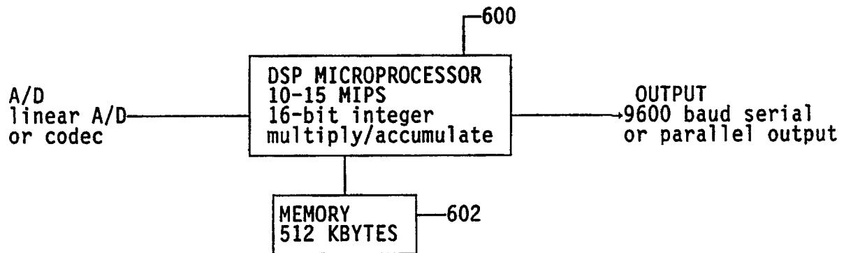
FIG. 45 PHONEME ESTIMATOR HARDWARE CONFIGURATION-1.
