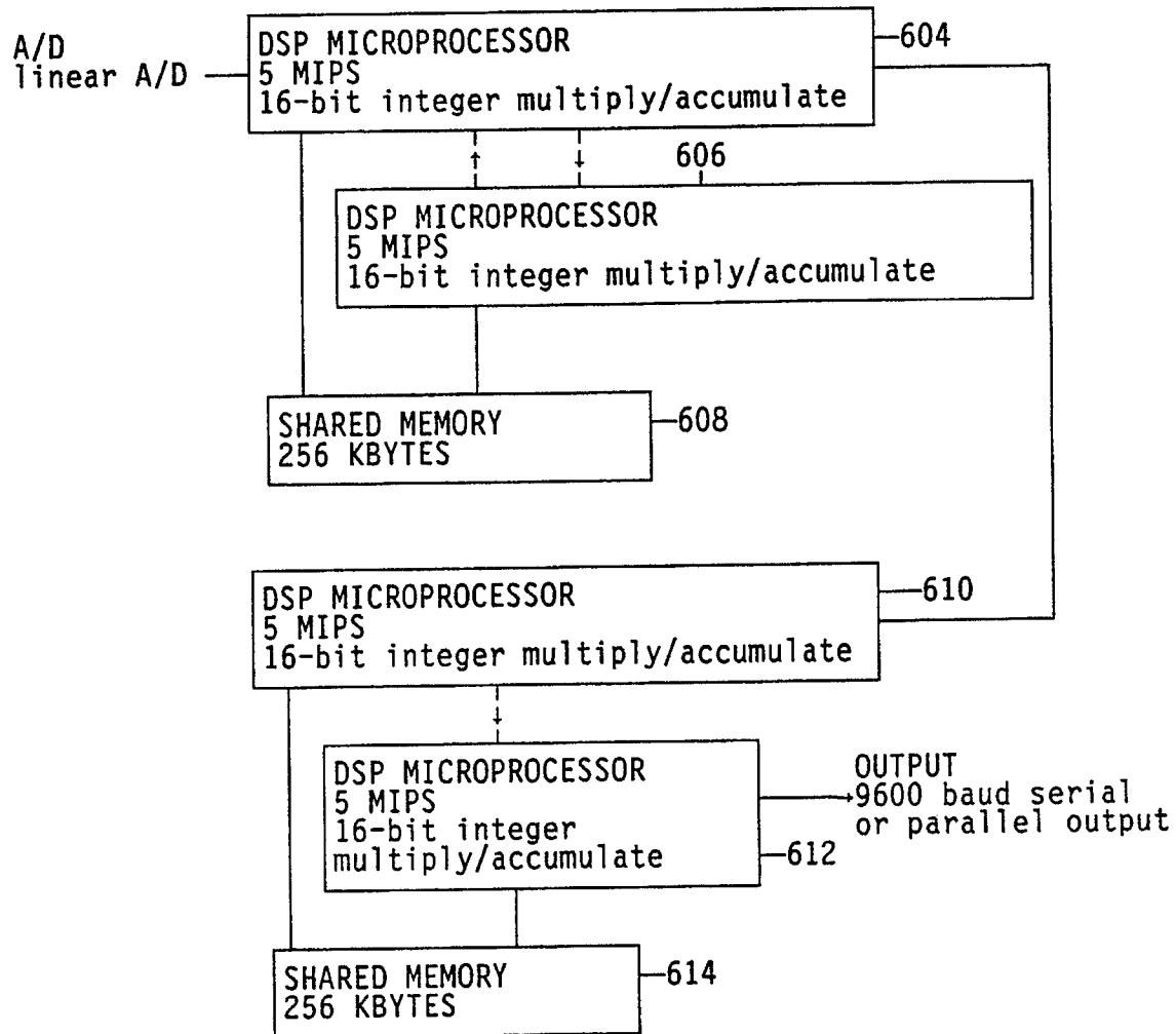
FIG. 46 PHONENE ESTIMATOR HARDWARE CONFIGURATION-2.
