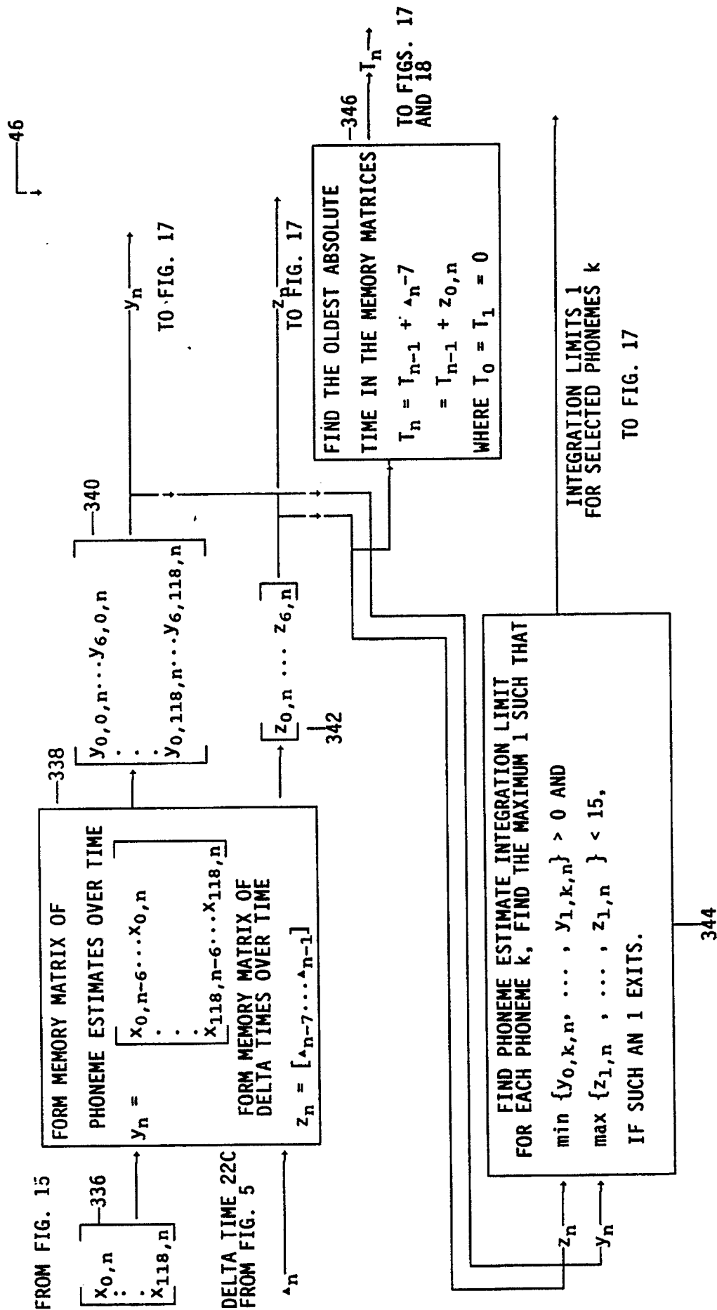
FIG. 16 ESTIMATOR INTEGRATOR, PART 1
