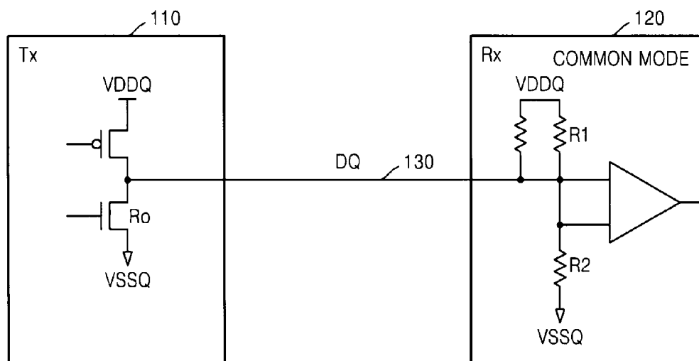
FIG. 2 (CONVENTIONAL ART)
