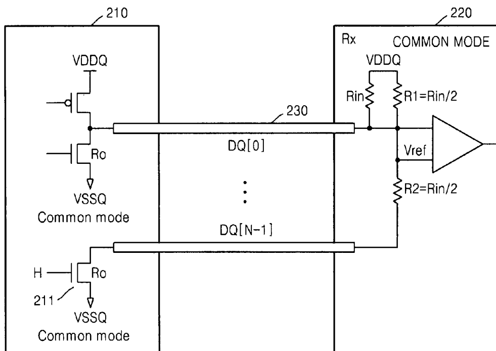
FIG. 2 (CONVENTIONAL ART)
