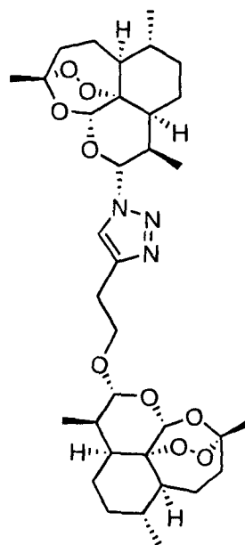
Compound 15
