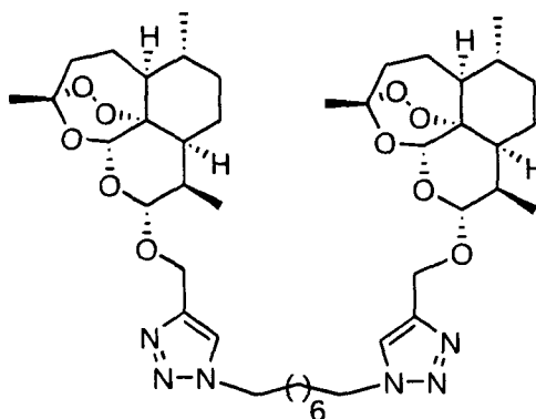
Compound 9b
