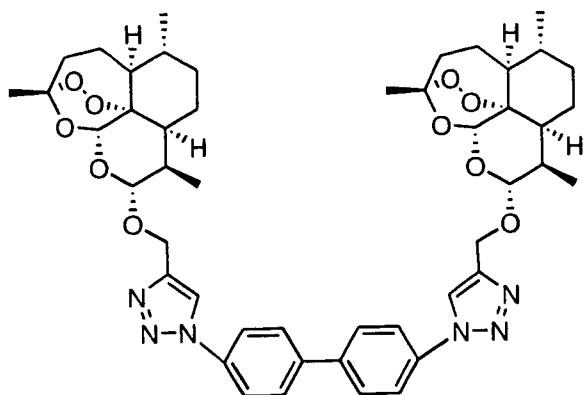
Compound 12
