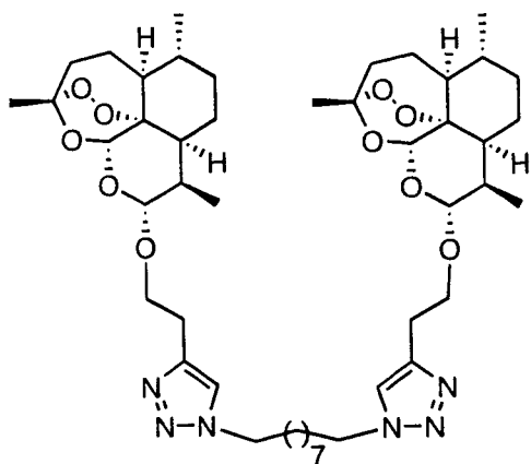
Compound 10b
