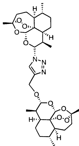
Compound 14
