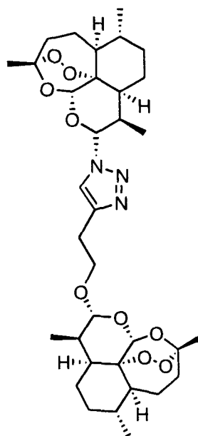
Compound 15
