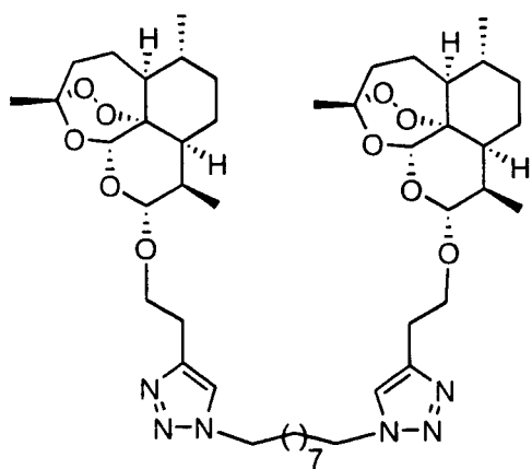
Compound 10b
