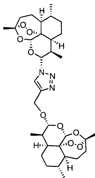
Compound 14
