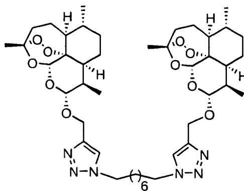
Compound 9b
