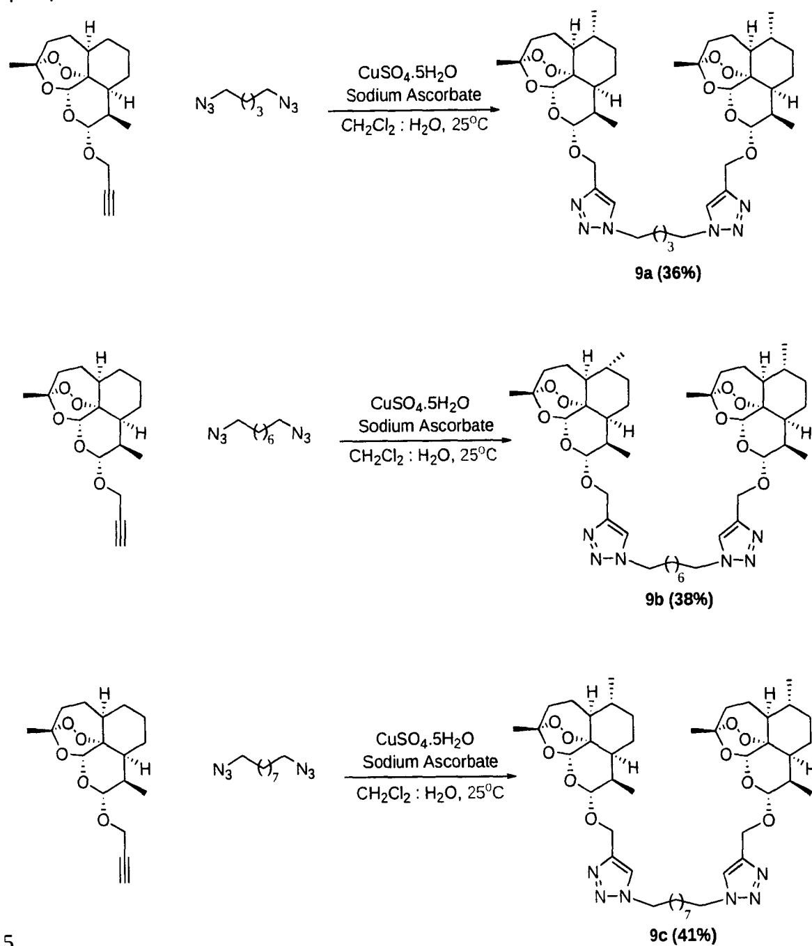
Scheme 3
