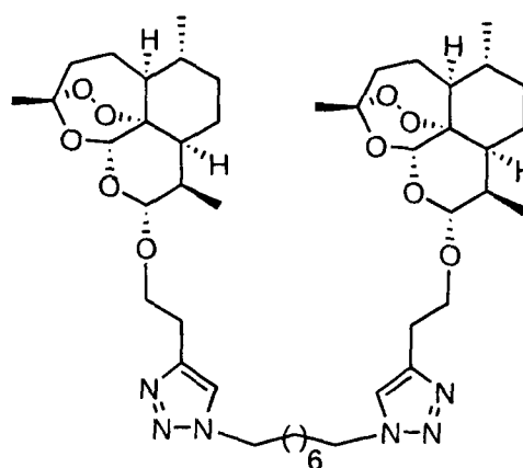
Compound 10a
