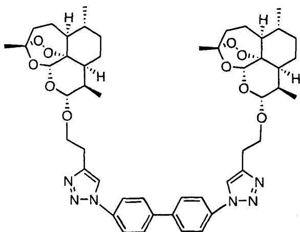
Compound 13
