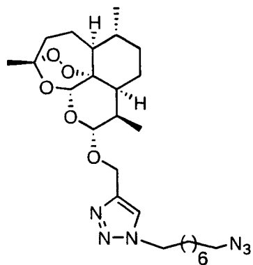
Compound 11
