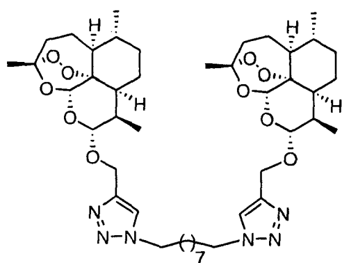
Compound 9c
