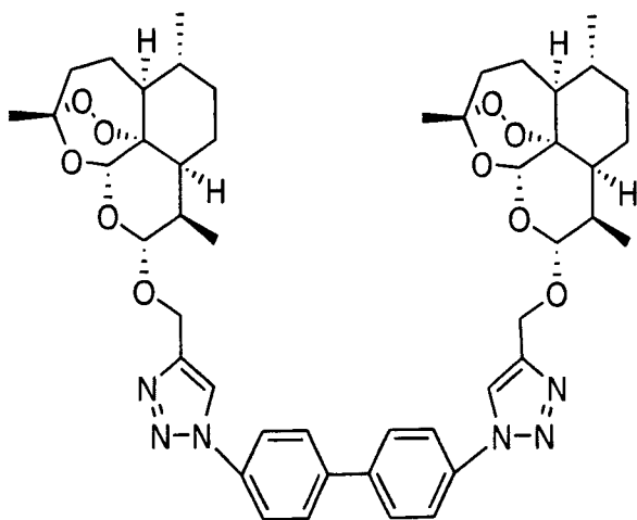
Compound 12
