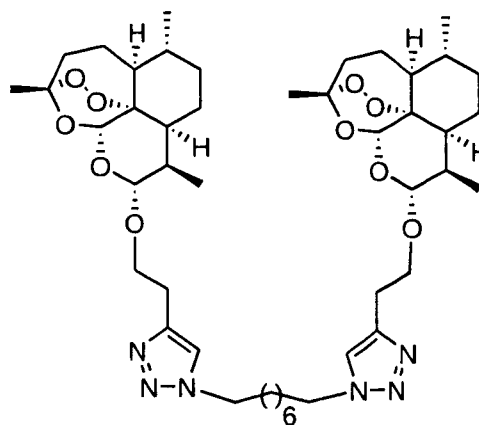
Compound 10a
