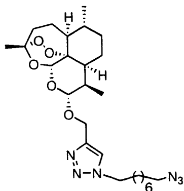
Compound 11
