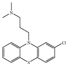
Chlorpromazine
