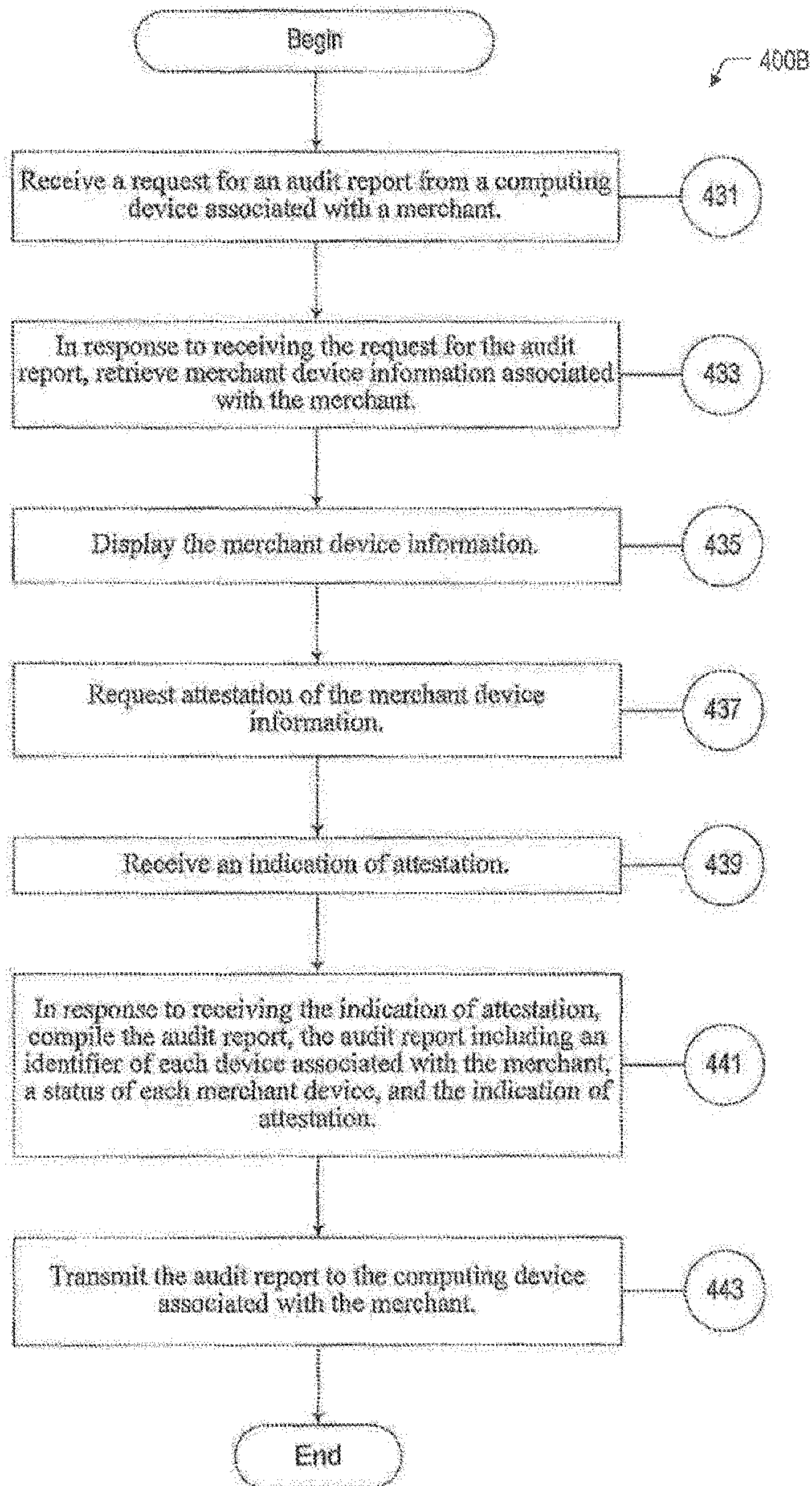
FIG. 4B P2PE REPORT PROCESS
