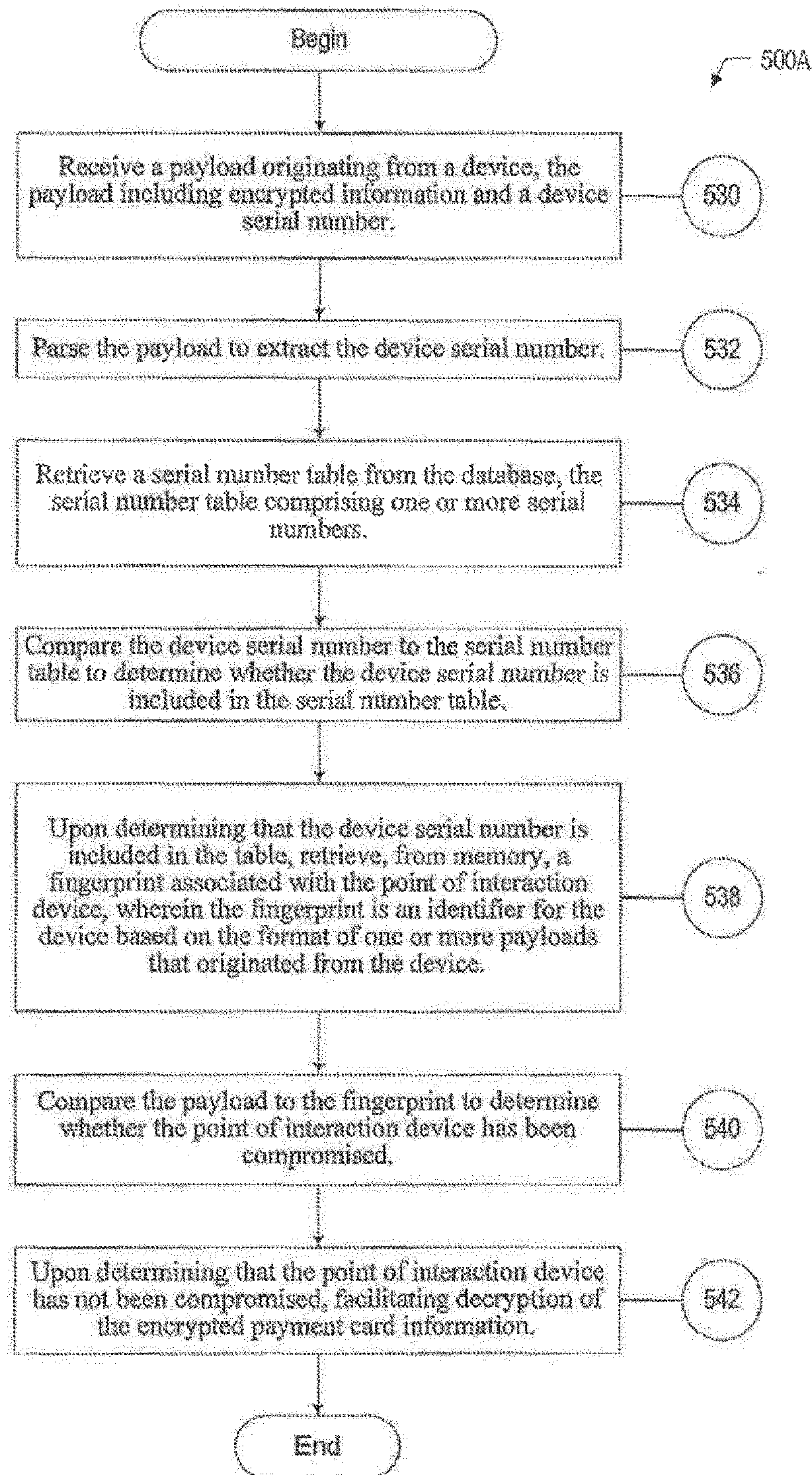
FIG. 5A EXEMPLARY DECRYPTION PROCESS
