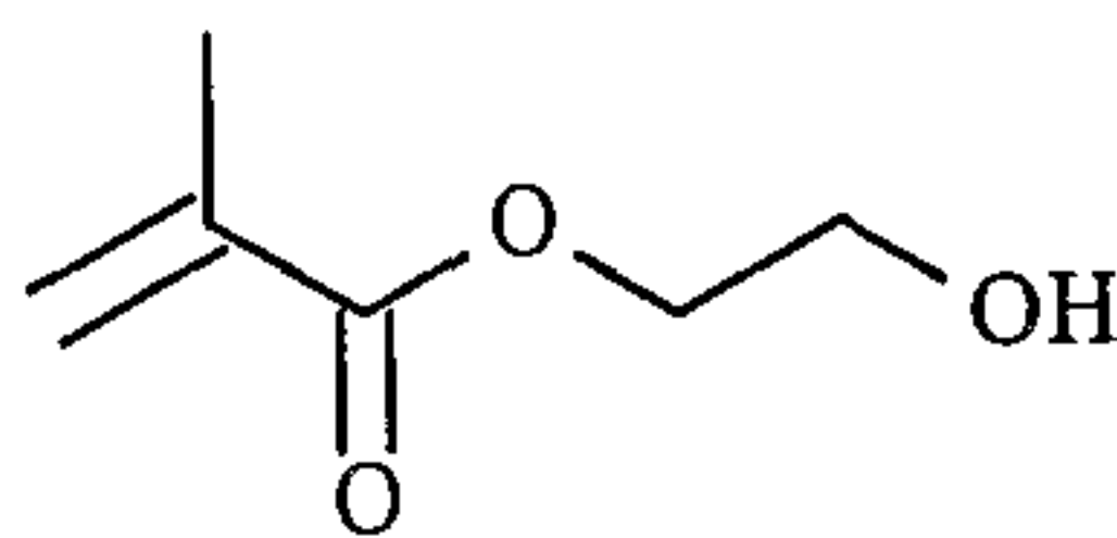
Compound E
