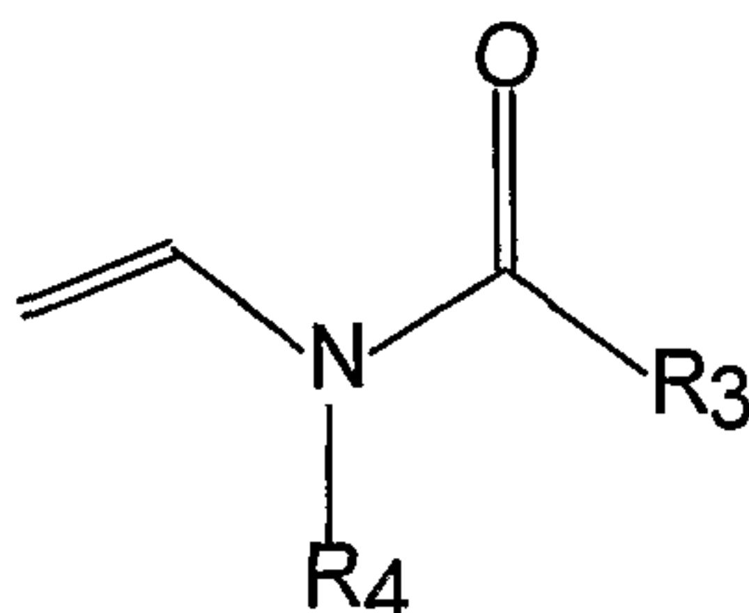
Formula II
