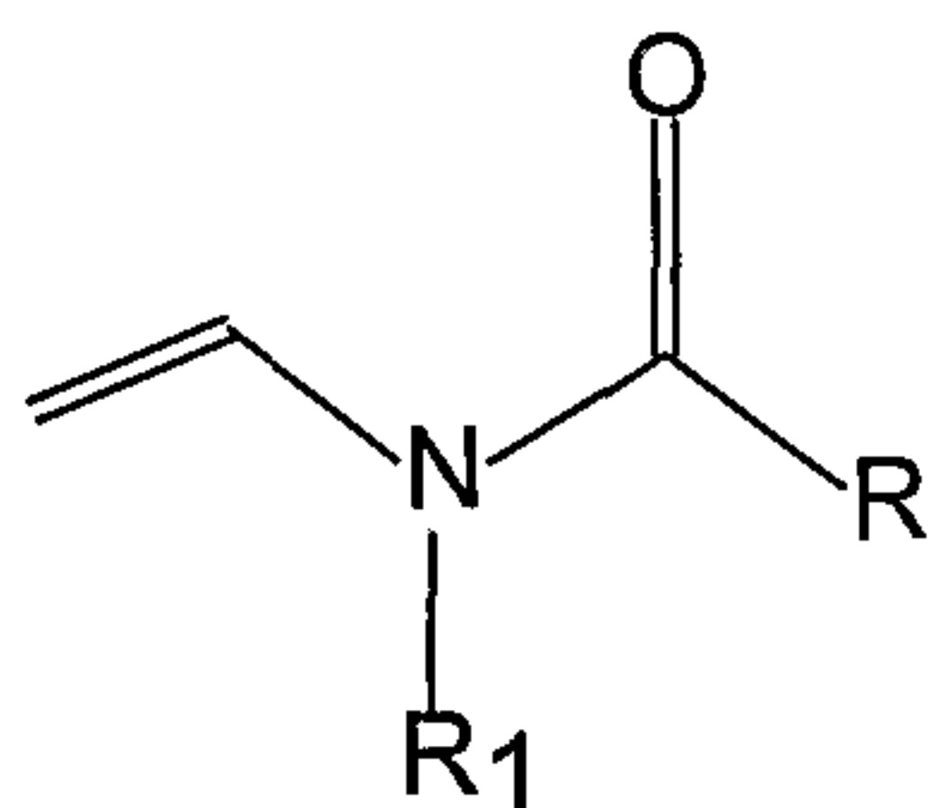
Formula I
