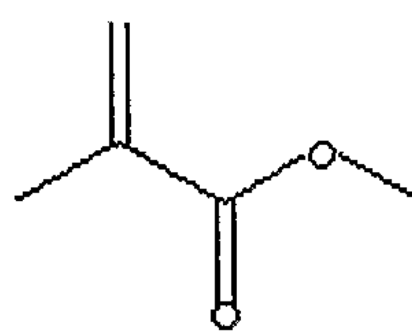
Compound L
