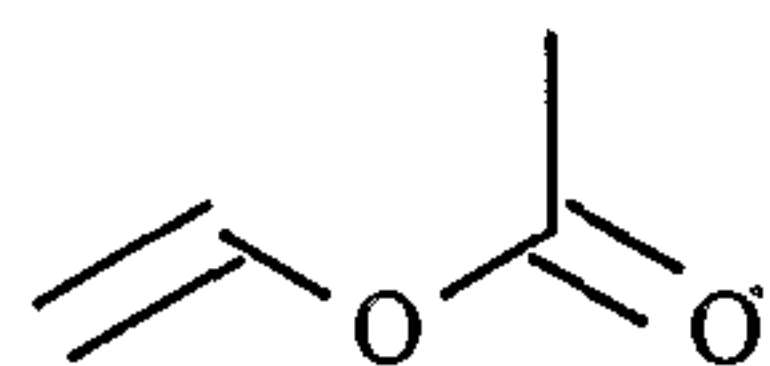
Compound J
