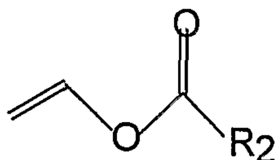
Formula IV
