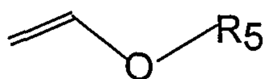
Formula III
