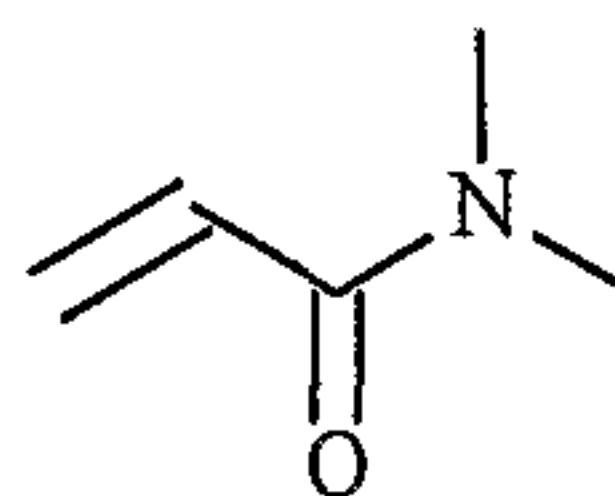
Compound G
