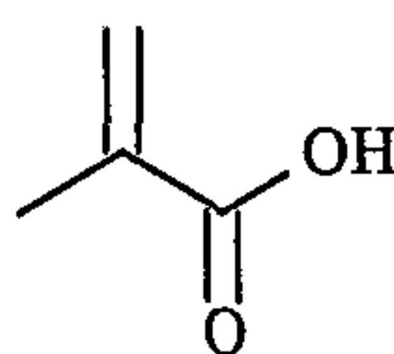
Compound H
