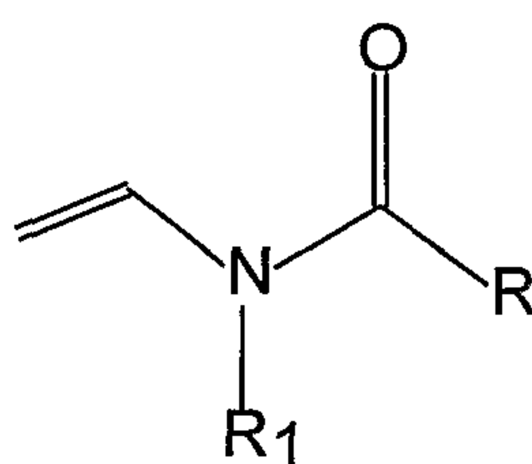
Formula I
