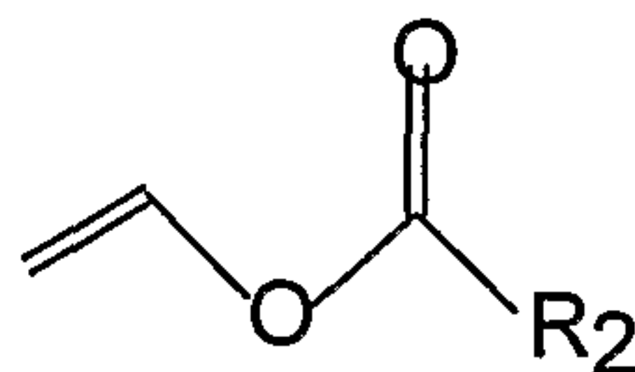
Formula IV
