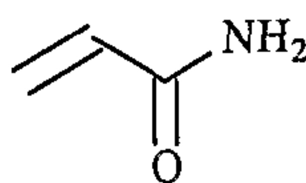
Compound F
