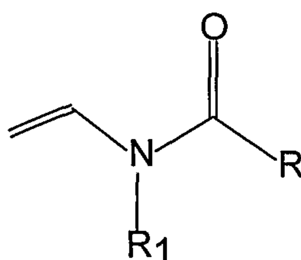
Formula I
