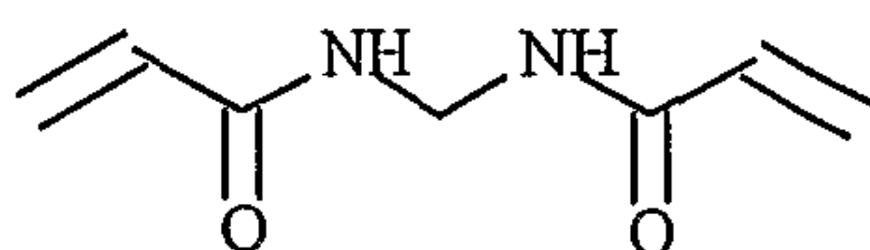
Compound D
