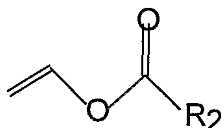
Formula IV
