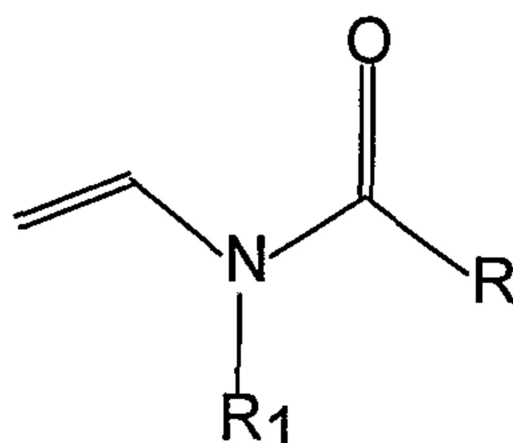
Formula I
