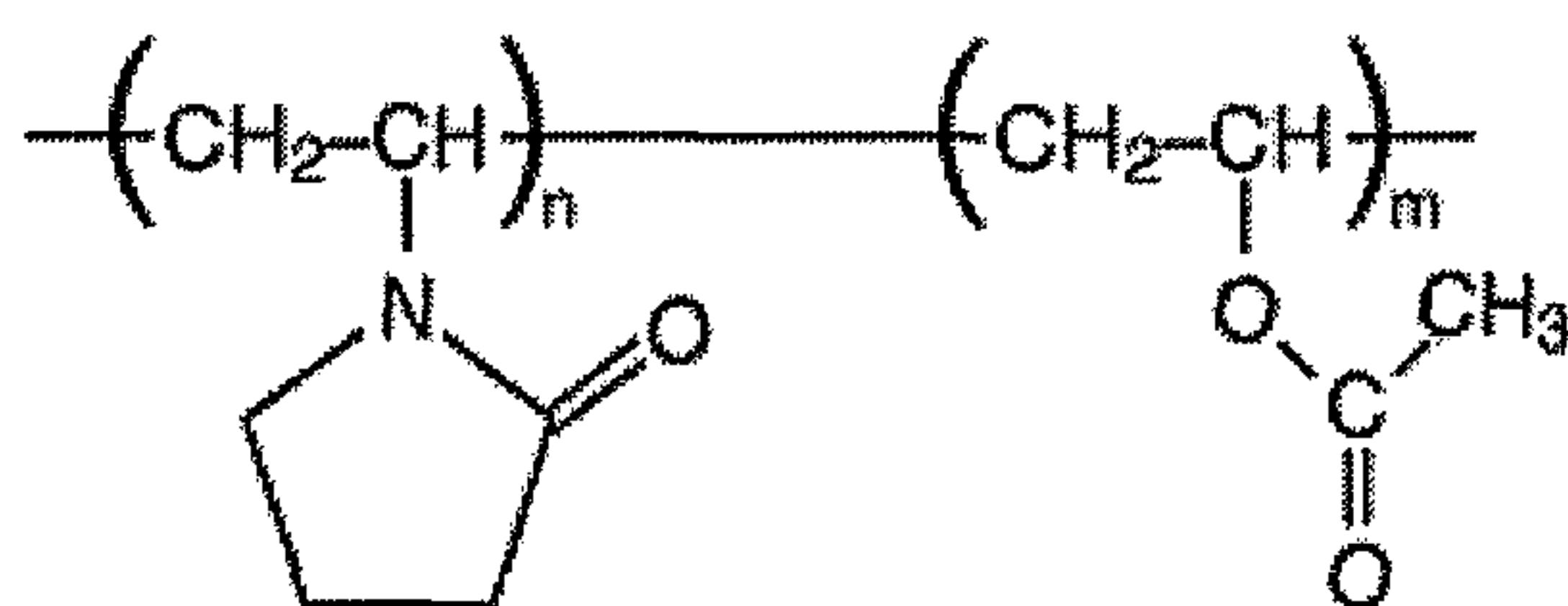
Formula M
