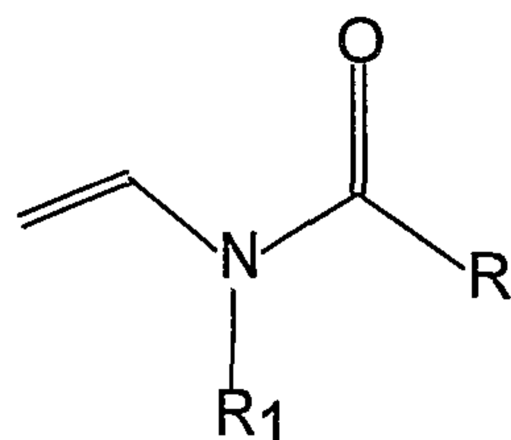
Formula I
