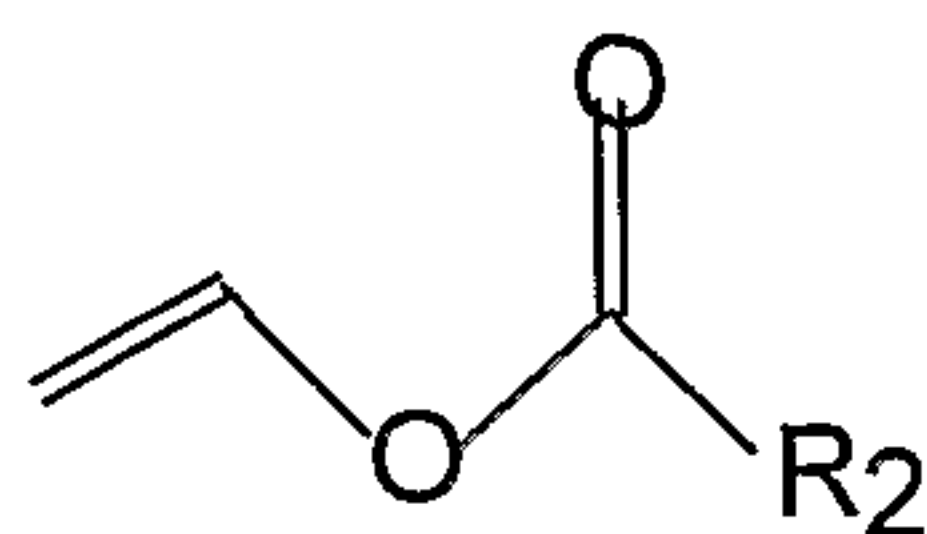
Formula IV
