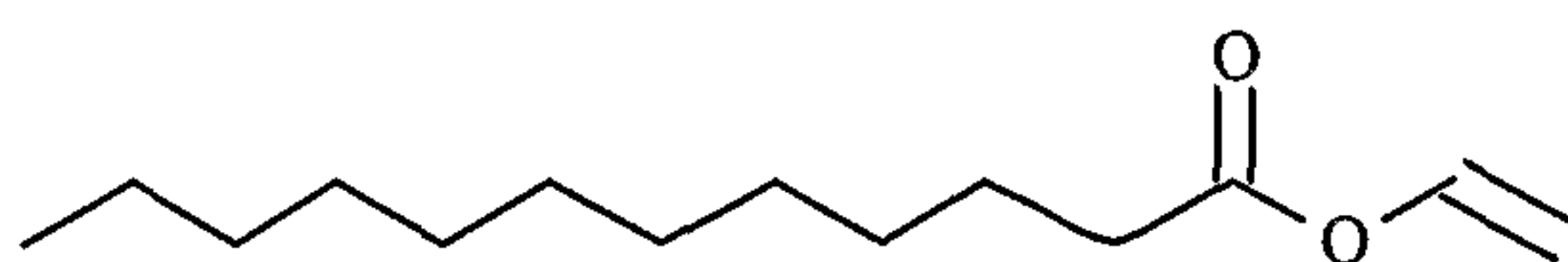
Compound K
