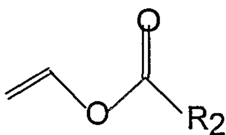
Formula IV
