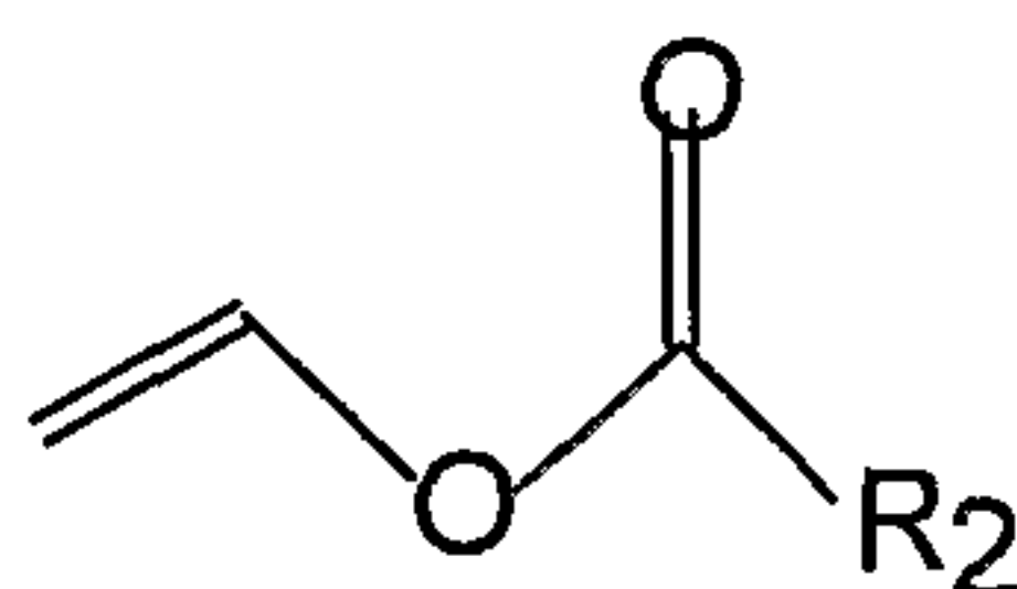
Formula IV
