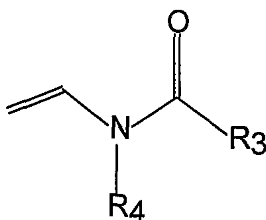
Formula II
