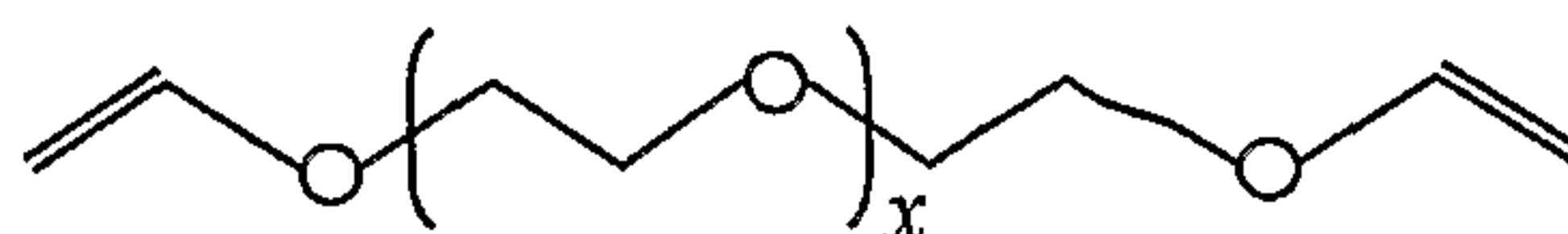
Formula V
