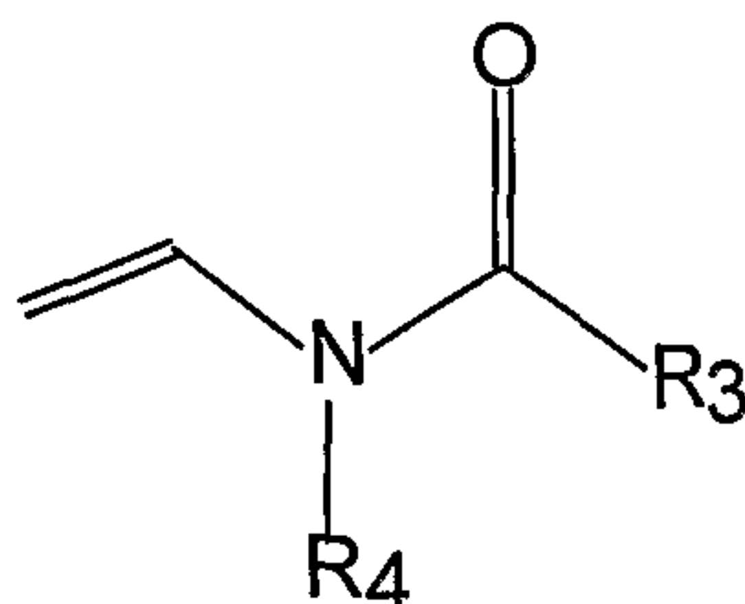
Formula II
