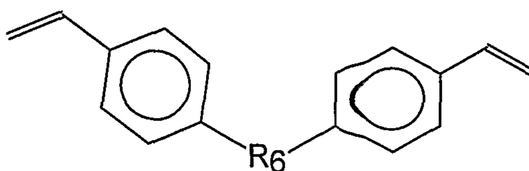
Formula VI
