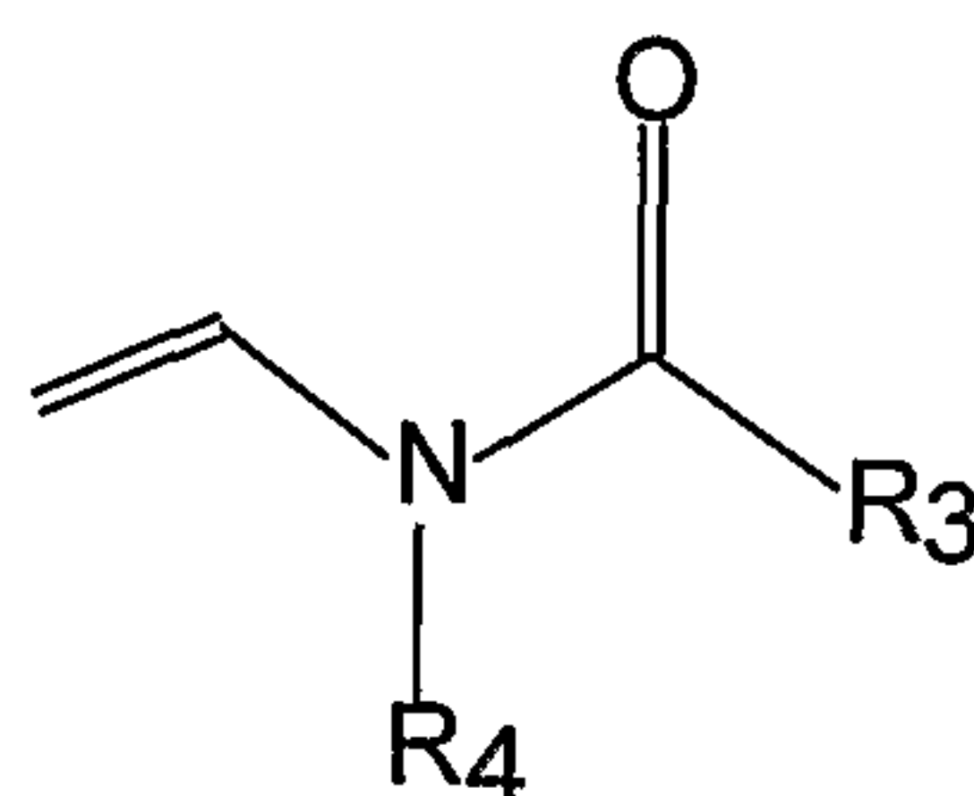
Formula II
