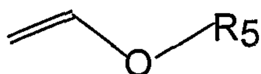
Formula III
