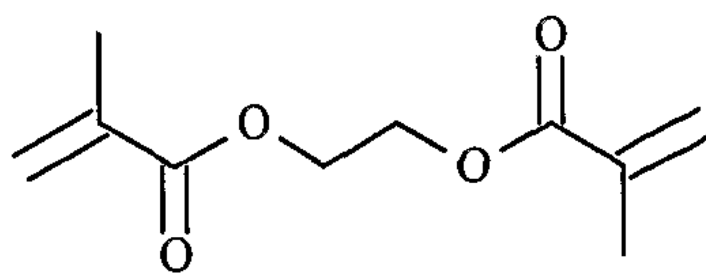
Compound C
