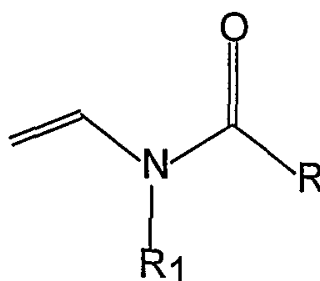
Formula I
