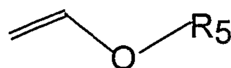
Formula III
