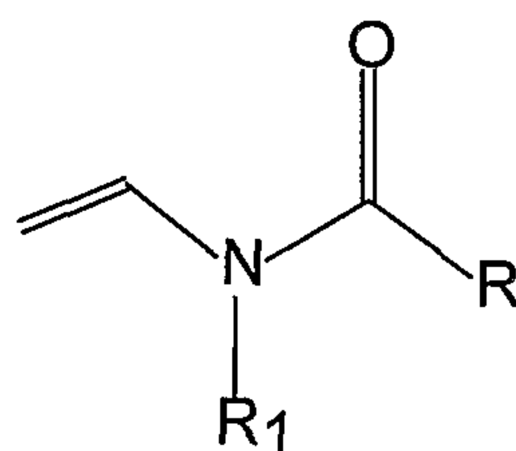
Formula I
