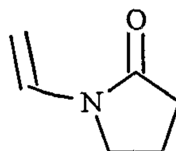
Compound A
