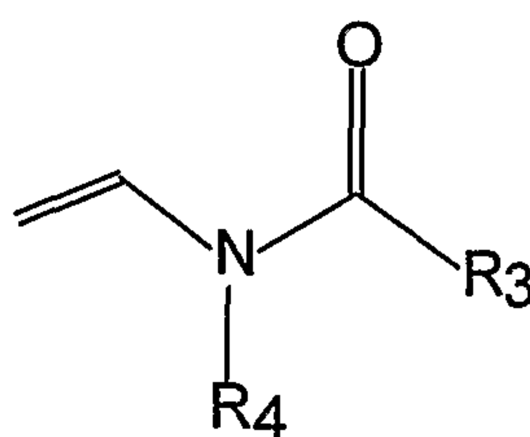
Formula II
