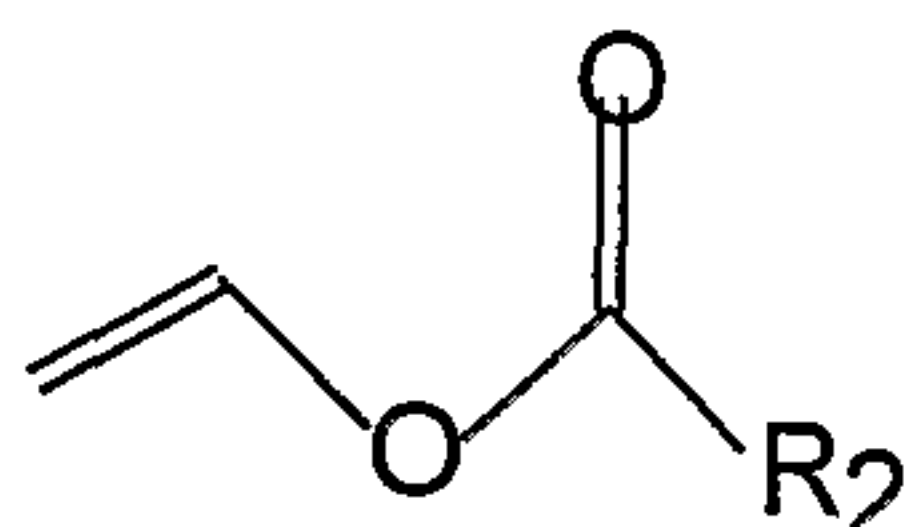
Formula IV
