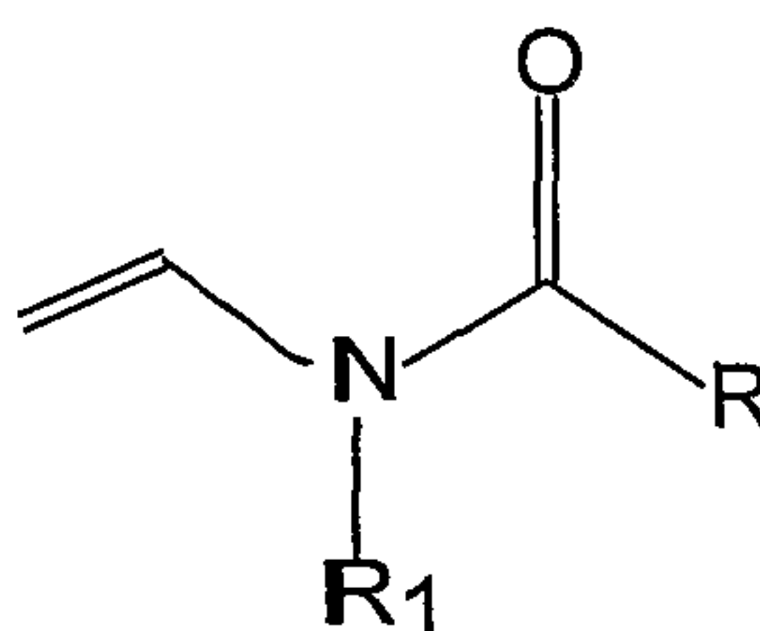
Formula I
