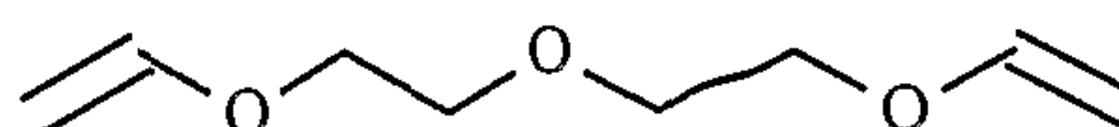
Compound B
