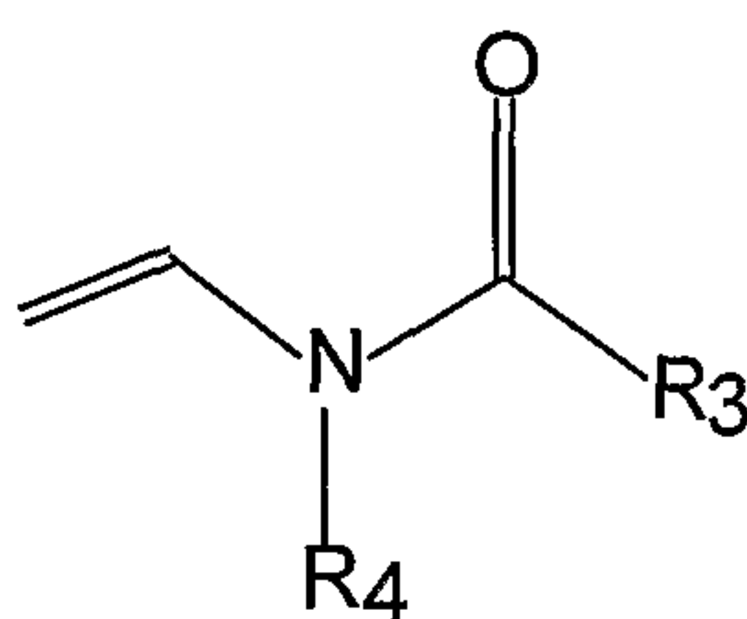
Formula II
