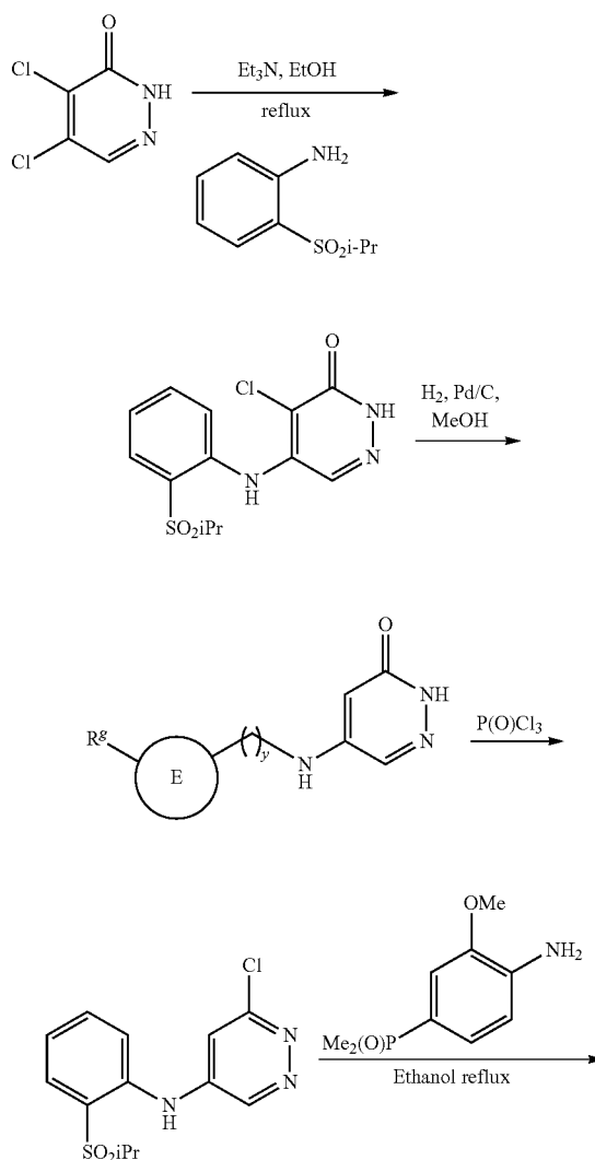
Scheme 33A
