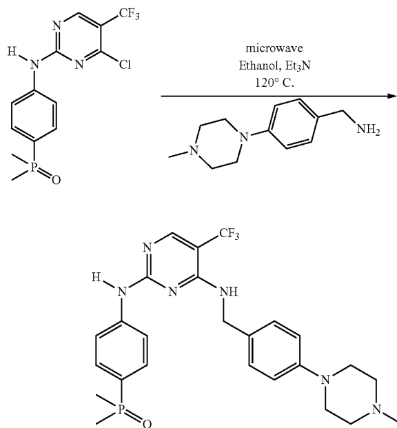
Scheme 4B
