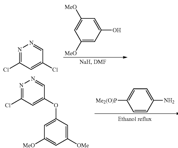
Scheme 32A
