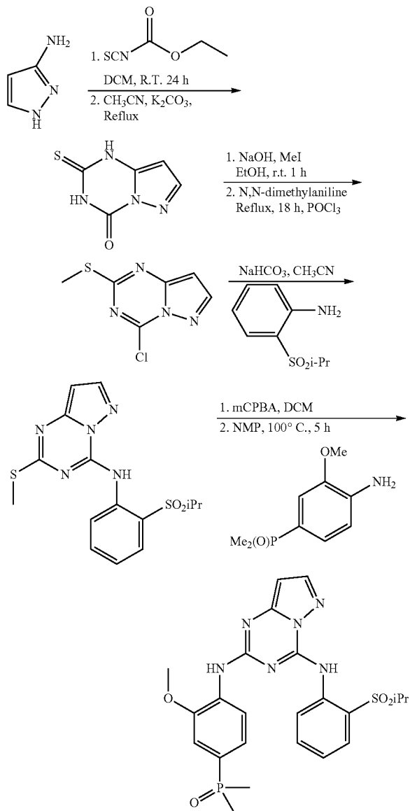
Scheme 52A
