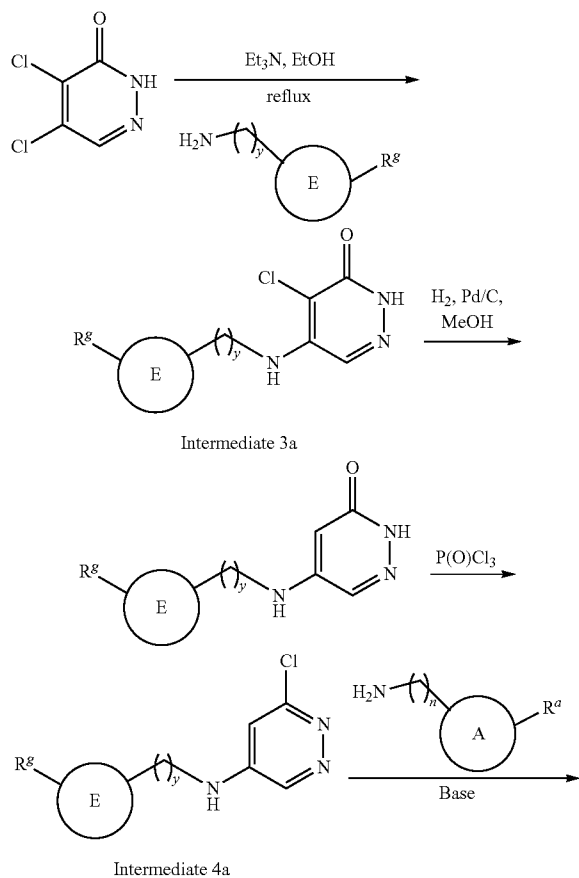
Scheme 33
