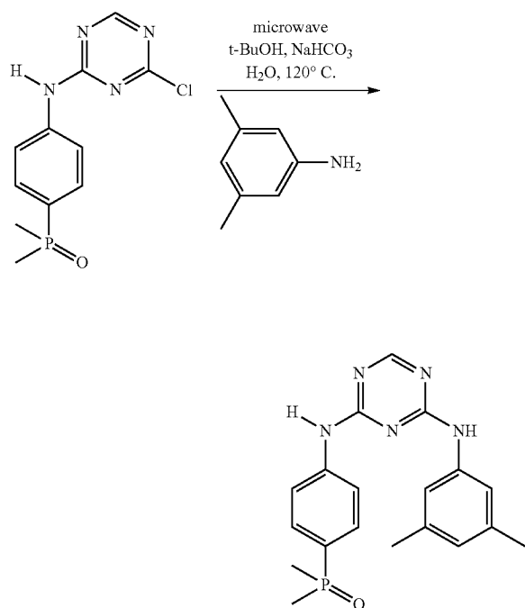
Scheme 44A
