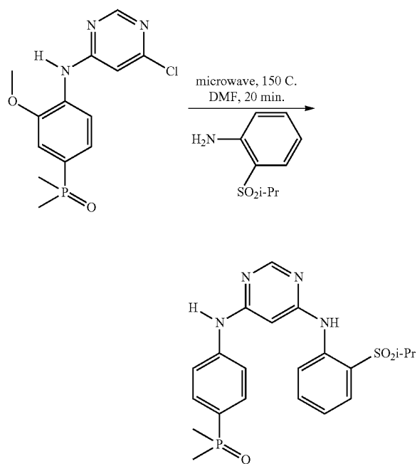
Scheme 26A
