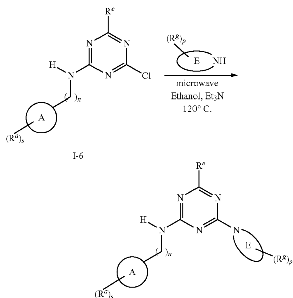
Scheme 49
