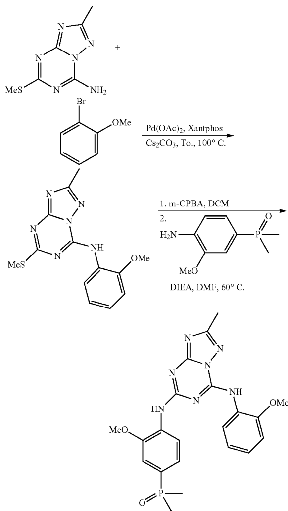
Scheme 51A
