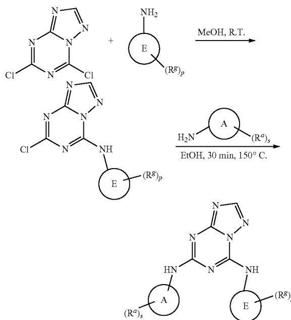
Scheme 50
