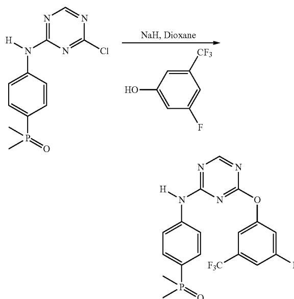
Scheme 43A
