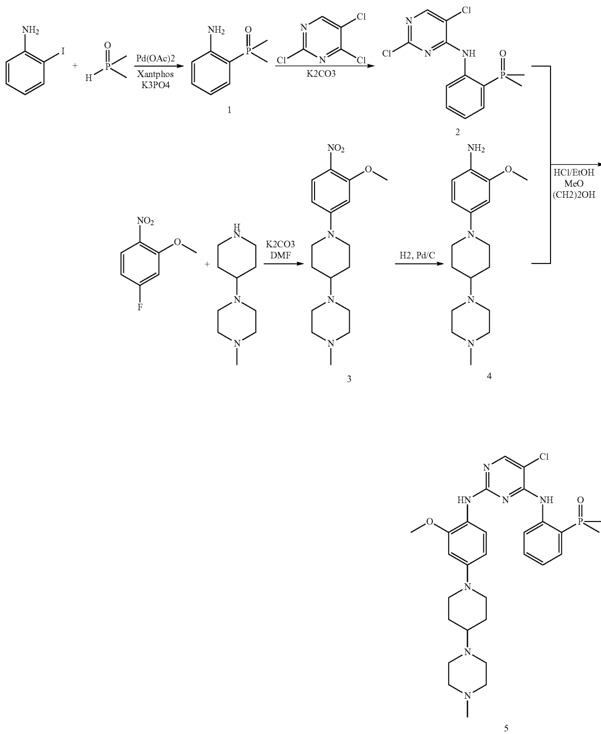
Scheme 122
