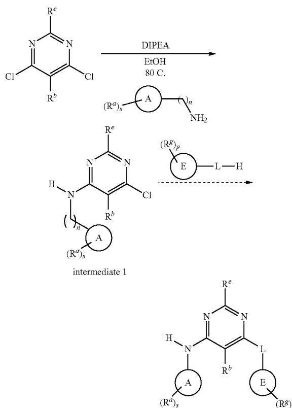
Scheme 25
