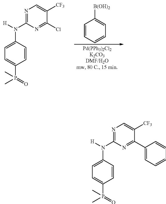
Scheme 6A
