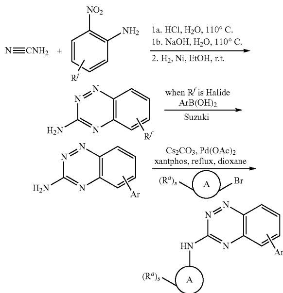
Scheme 57
