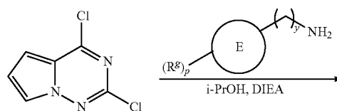
Scheme 53
