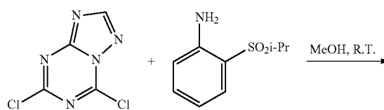
Scheme 50A
