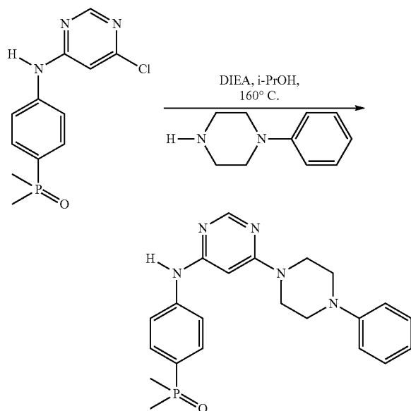
Scheme 27A
