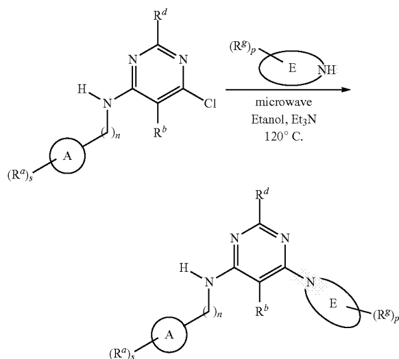
Scheme 27
