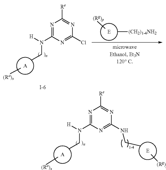
Scheme 45
