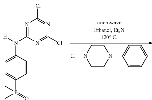
Scheme 49A
