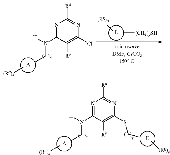
Scheme 30
