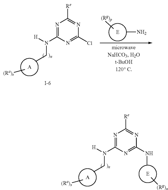
Scheme 44
