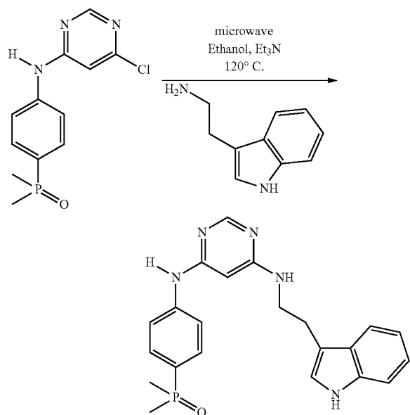
Scheme 29B
