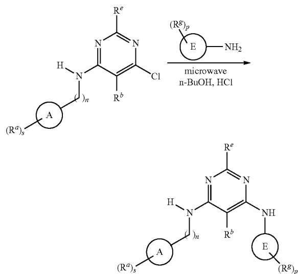
Scheme 26
