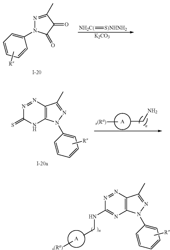
Scheme 56
