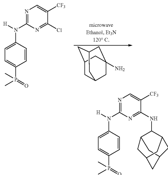
Scheme 3B
