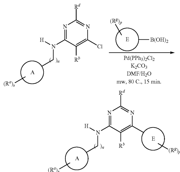
Scheme 31
