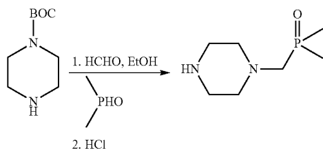
Scheme 24
