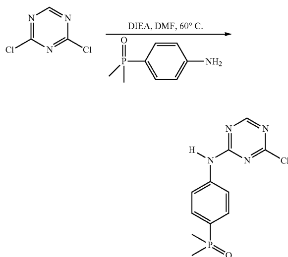
Scheme 42B
