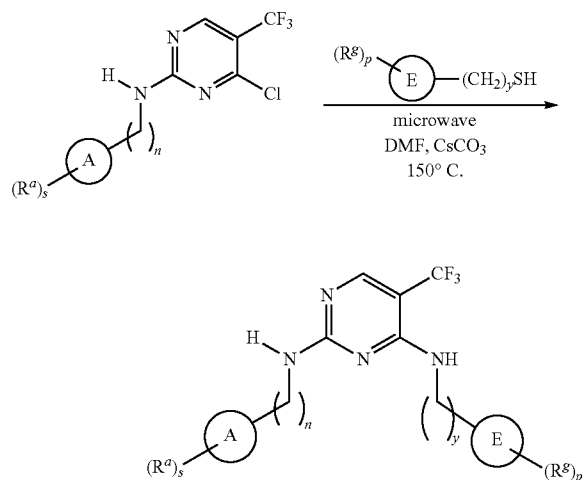
Scheme 5
