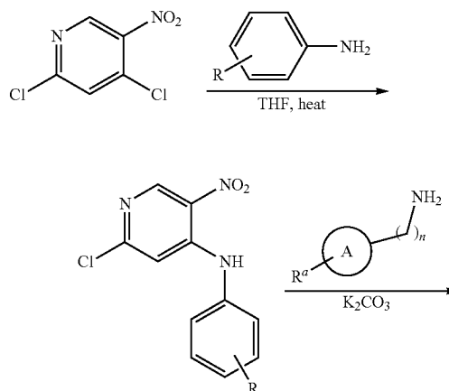
Scheme 36
