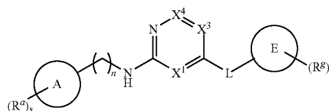
Formula VI
