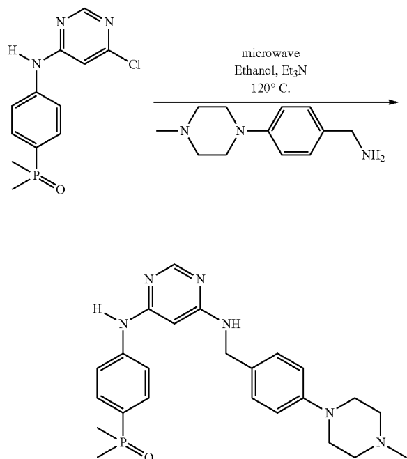
Scheme 29A
