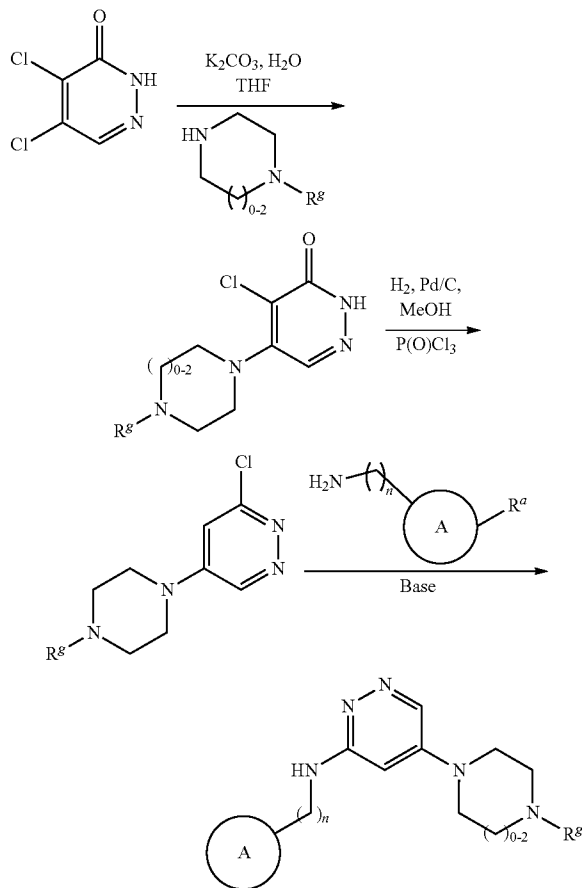
Scheme 35
