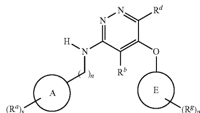
Intermediate 2a
