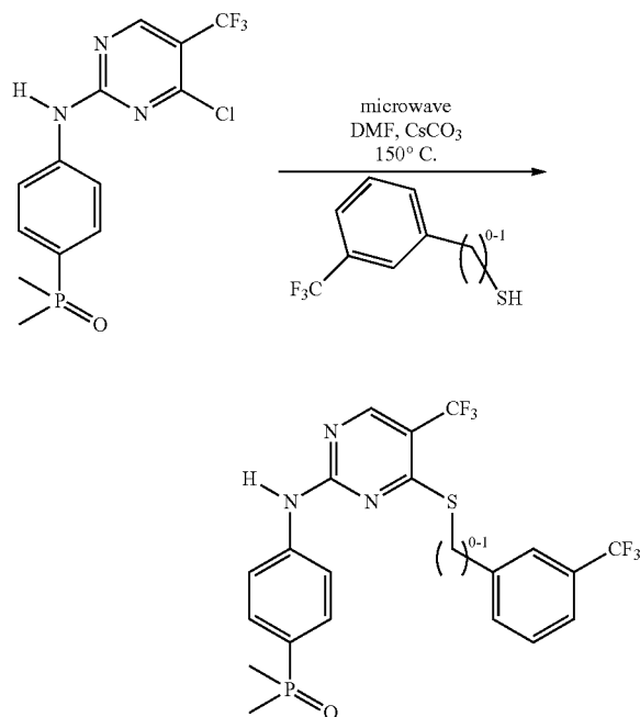
Scheme 5A
