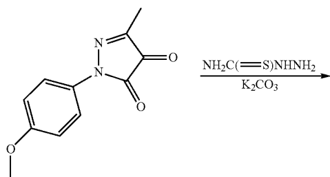
Scheme 56A
