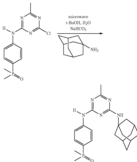
Scheme 44B
