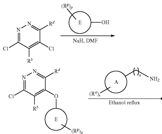
Intermediate 2a
