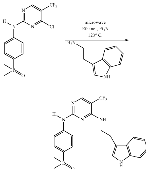
Scheme 4A
