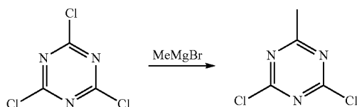
Scheme 42A
