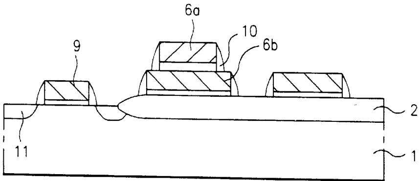
FIG. 2g Prior Art
