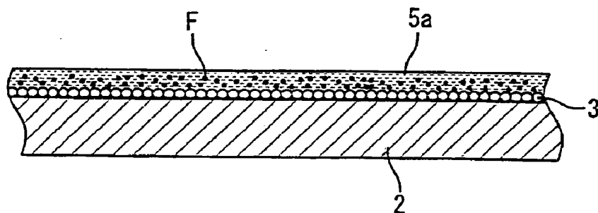
(b) Drying of the dielectric filler containing resin film
