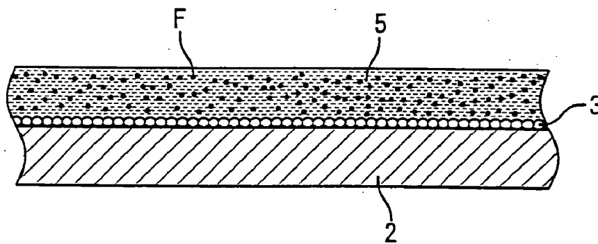
(d) Drying of the re-formed dielectric filler containing resin film
