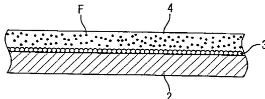
(a) Formation of a dielectric filler containing resin film
