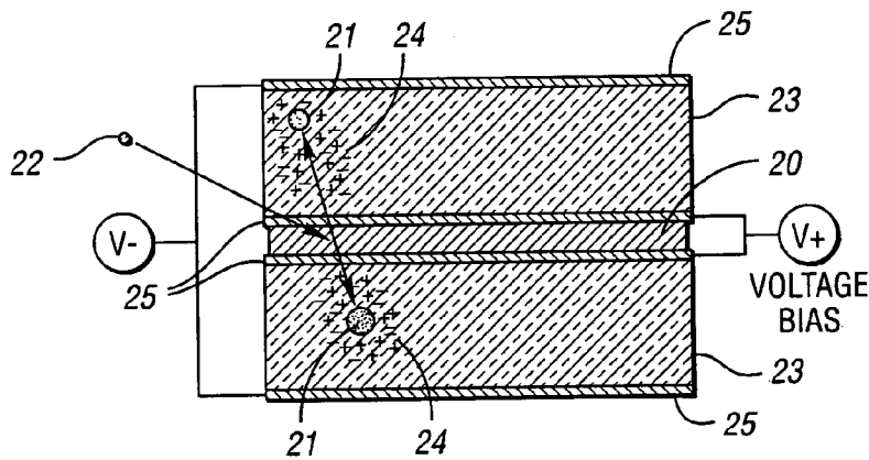
Fig. 2 (PRIOR ART)
