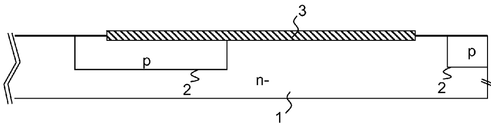
FIG. 2B A-A' SECTIONAL VIEW
