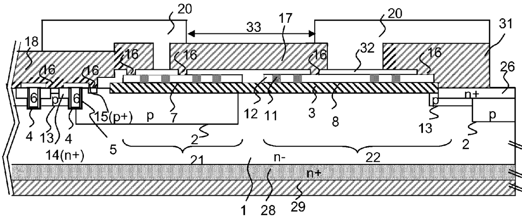
FIG. 17B A-A' SECTIONAL VIEW
