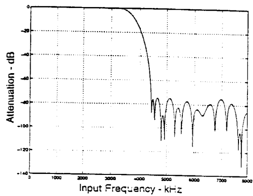
Figure 4. Decimation Filter Response
