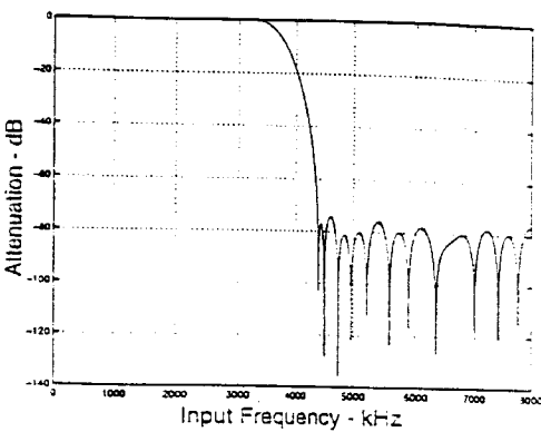
Figure 6. Interpolation Filter Response
