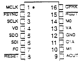
Figure 16. Si3032A Pin Configuration
