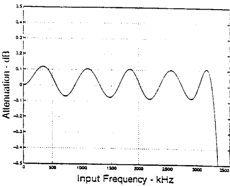
Figure 7. Interpolation Filter Passband Ripple
