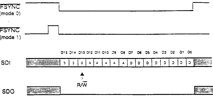
Figure 15. Secondary Communication Data Format—Write Cycle
