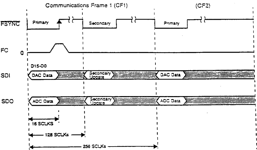
Figure 13. Hardware FC Secondary Request
