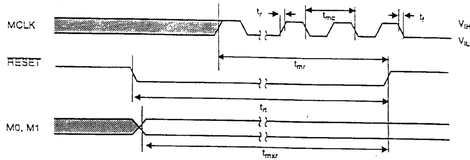
Figure 1. General Inputs Timing Diagram
