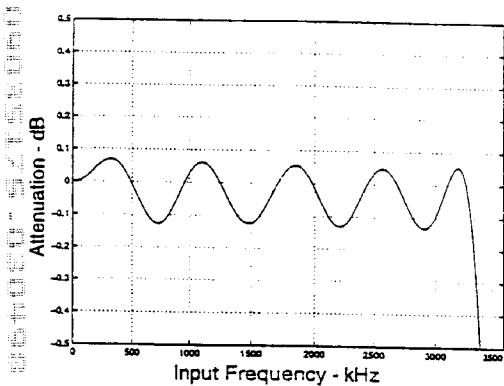
Figure 5. Decimation Filter Passband Ripple
