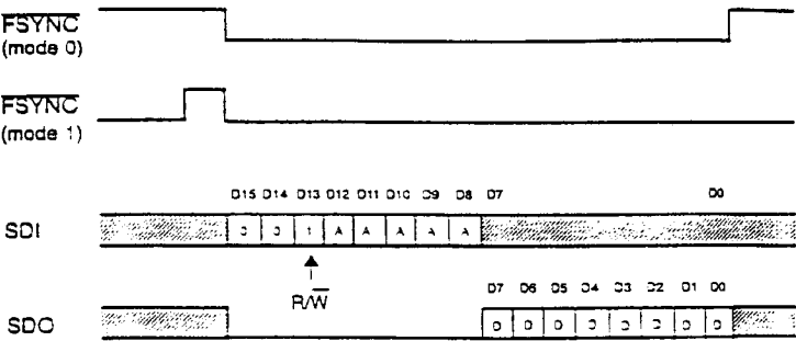
Figure 14. Secondary Communication Data Format—Read Cycle
