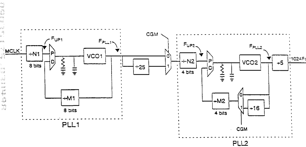
Figure 11. Clock Generation Subsystem
