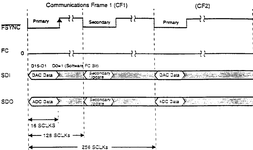
Figure 12. Software FC Secondary Request
