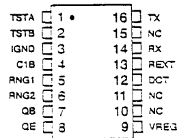
Figure 17. Si3032B Pin Configuration
