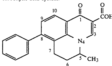
6,7-dihydro-5-methyl-1-oxo-8-phenyl-1H,5H-benzo[ ij ]quinolizine-2-carboxylic acid system:
