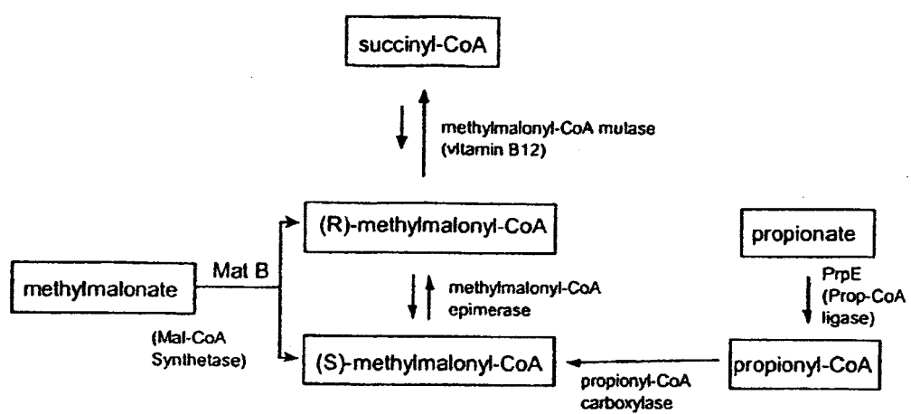
Biosynthetic pathways to (S)-methymalonyl-CoA
