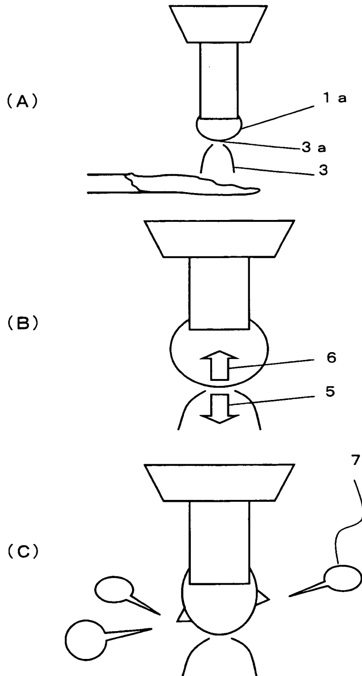
FIG. 13 PRIOR ART
