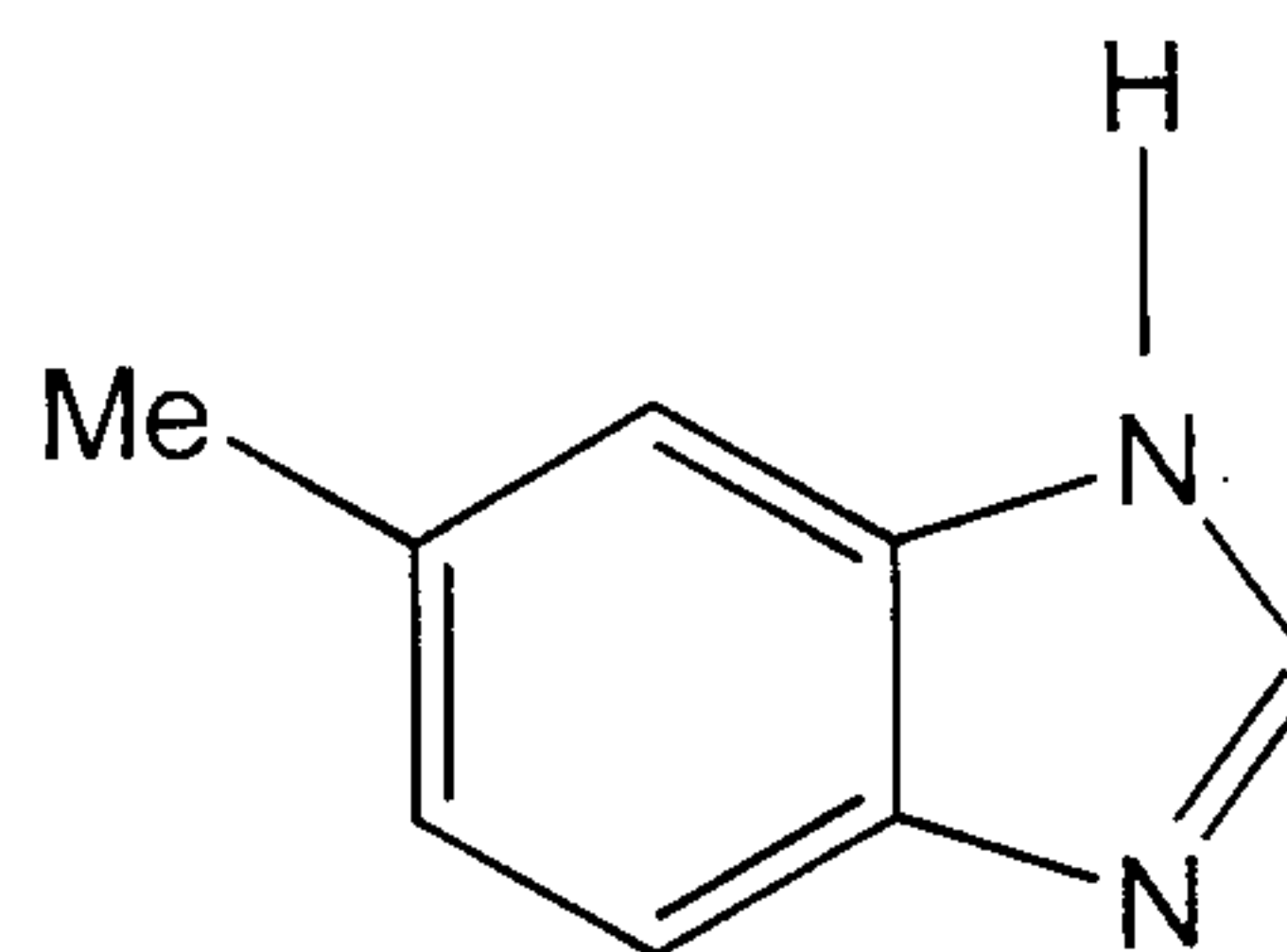
5-Methyl benzimidazole
