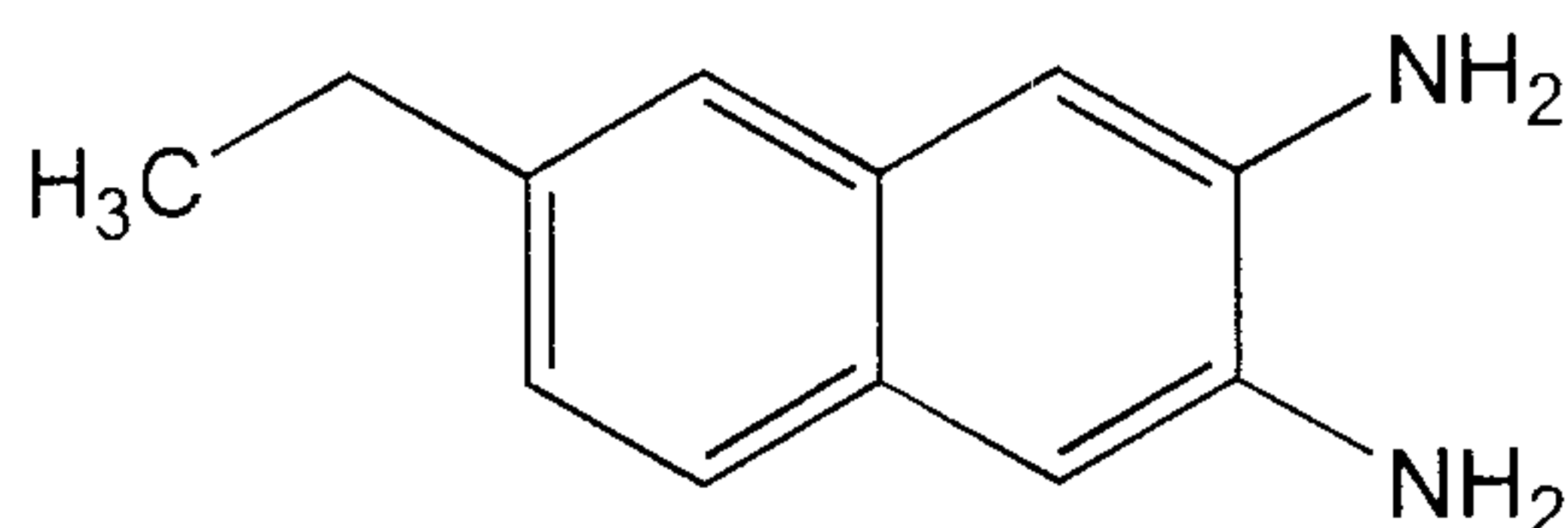
6-Ethyl-2,3-diamino naphthalene
