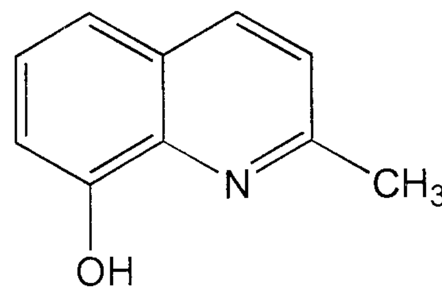
8-hydroxy quinaldine
