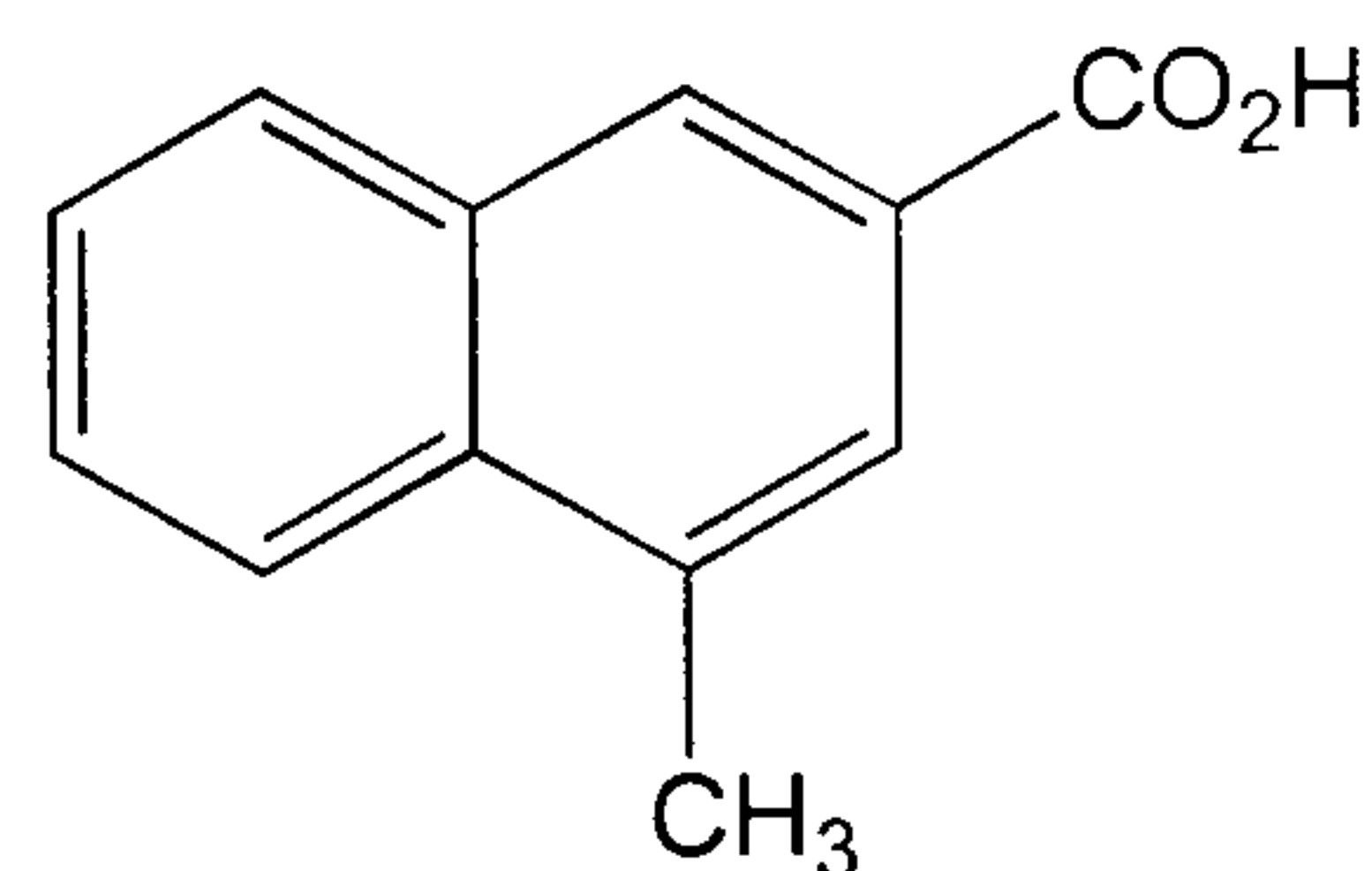
4-Methyl-2-naphthoic acid
