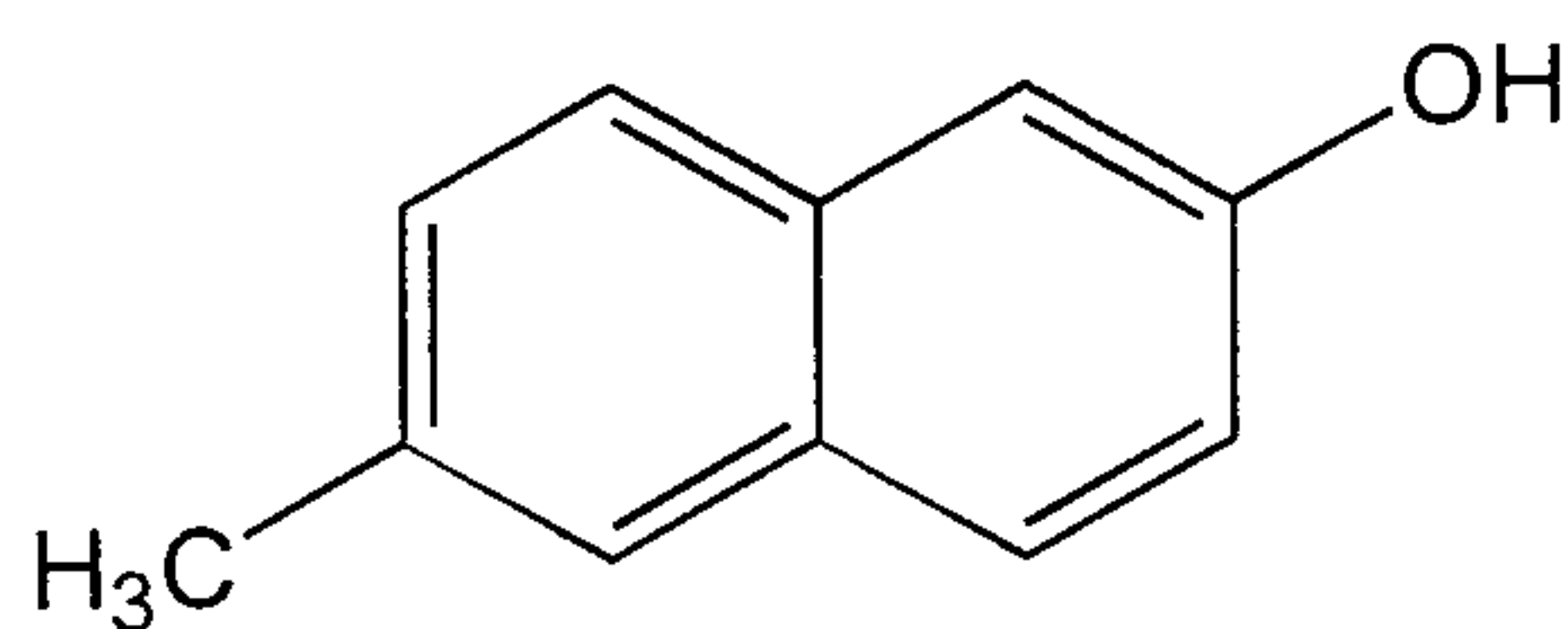
6-Methyl naphth-2-ol
