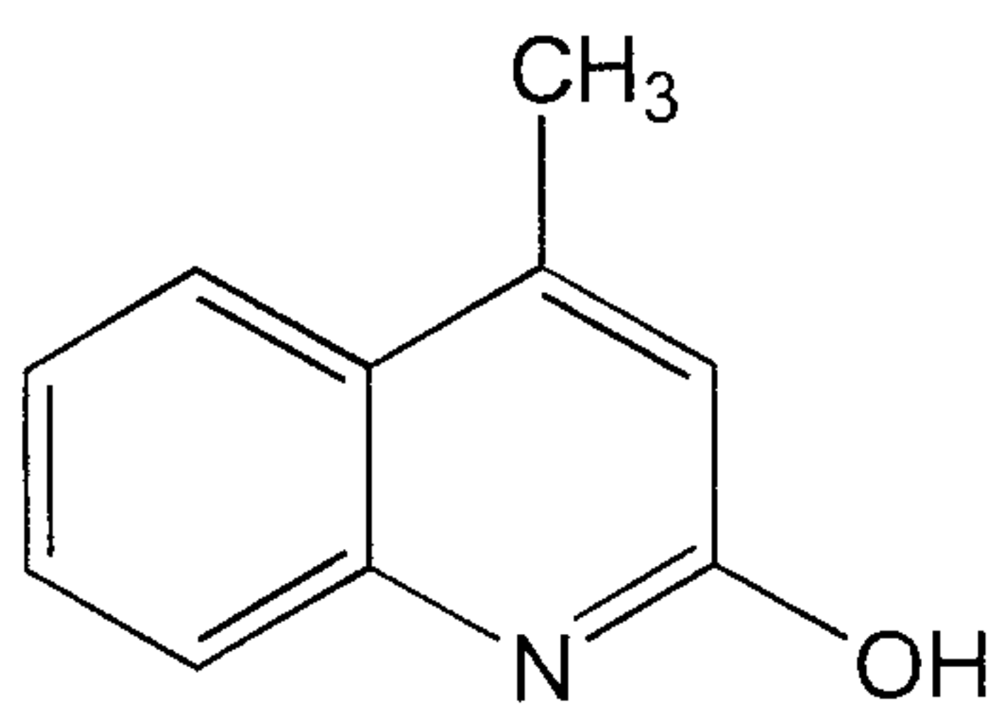
2-hydroxy-4-methyl quinoline
