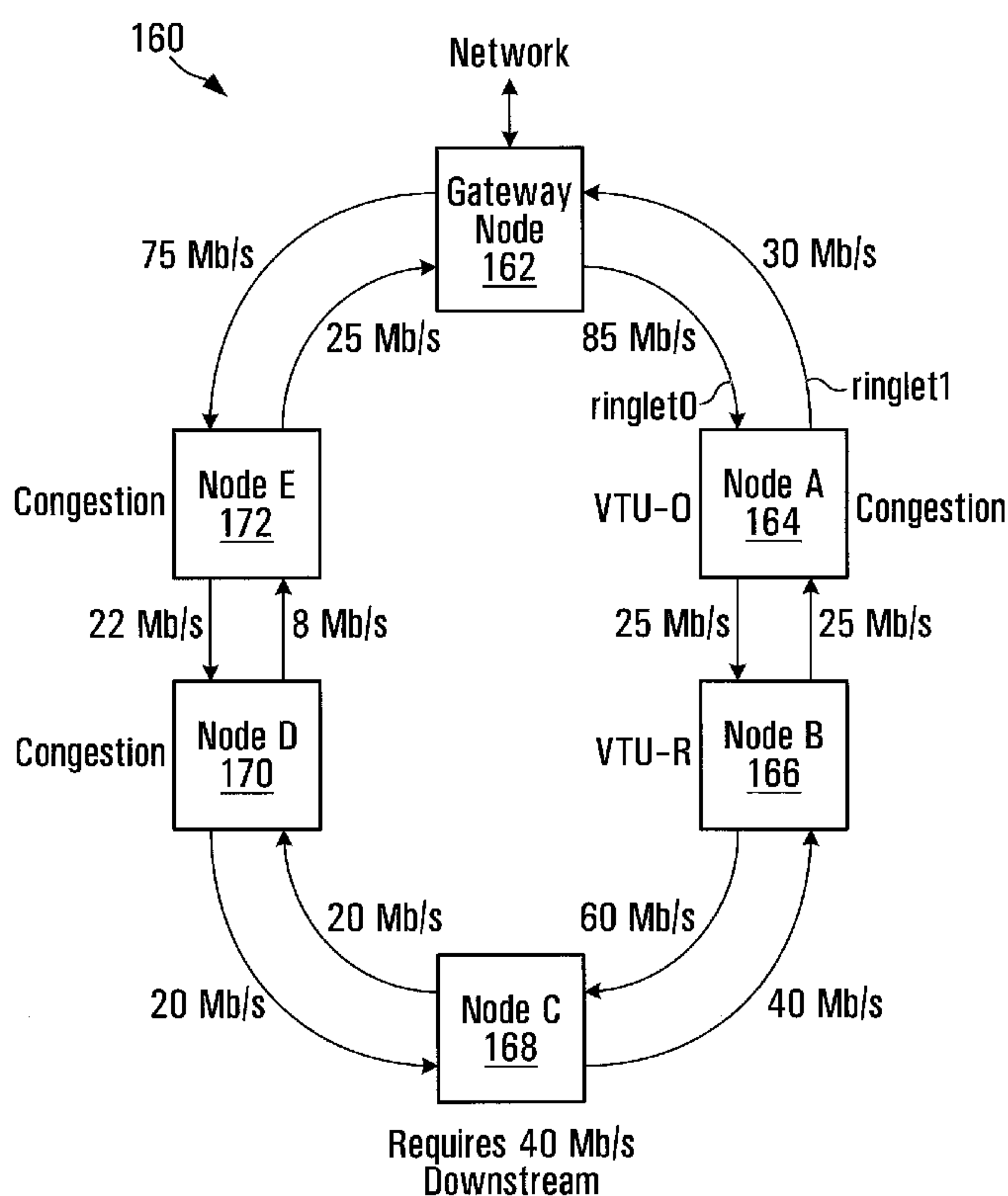
Asymmetric DSL Rings Dynamically Optimized Ring
