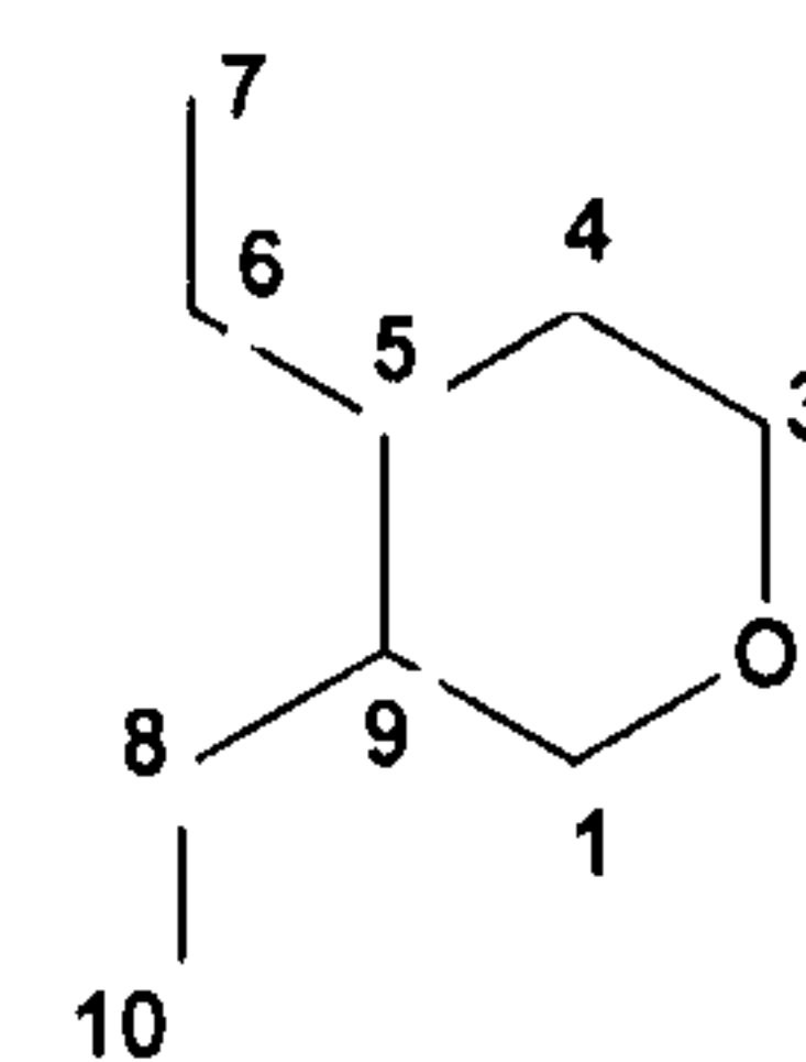
simple secoiridoid
