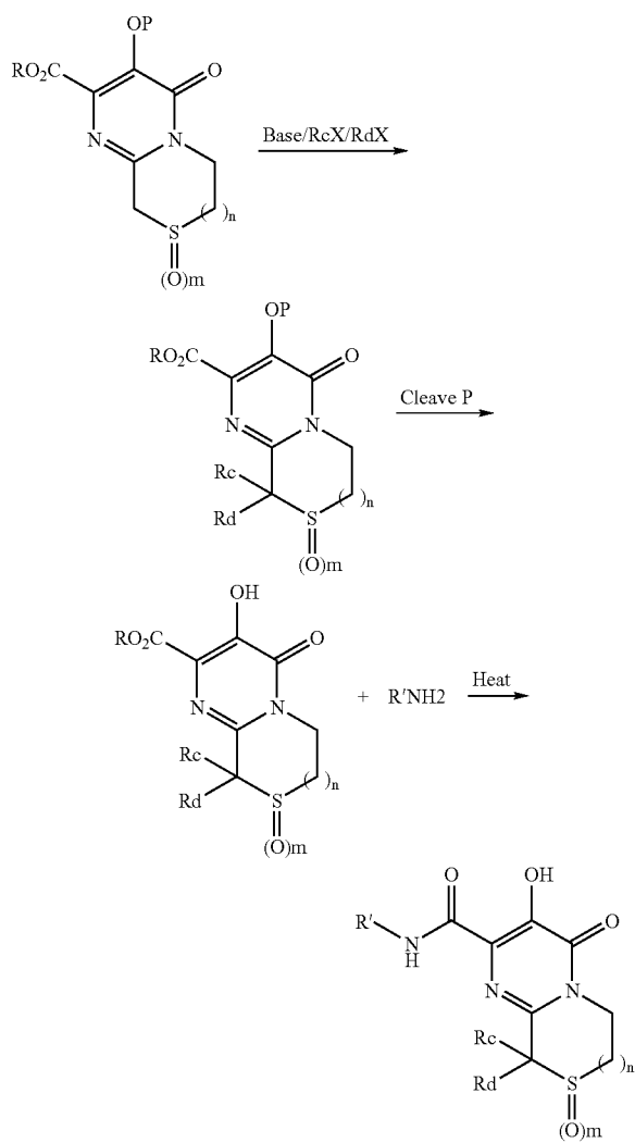
Scheme XIX.
