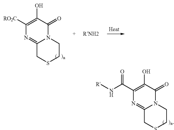
Scheme XVI
