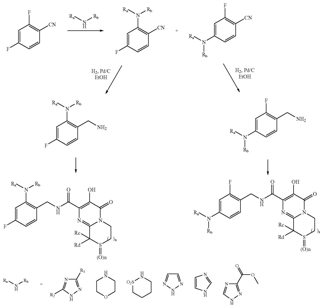
Scheme X
