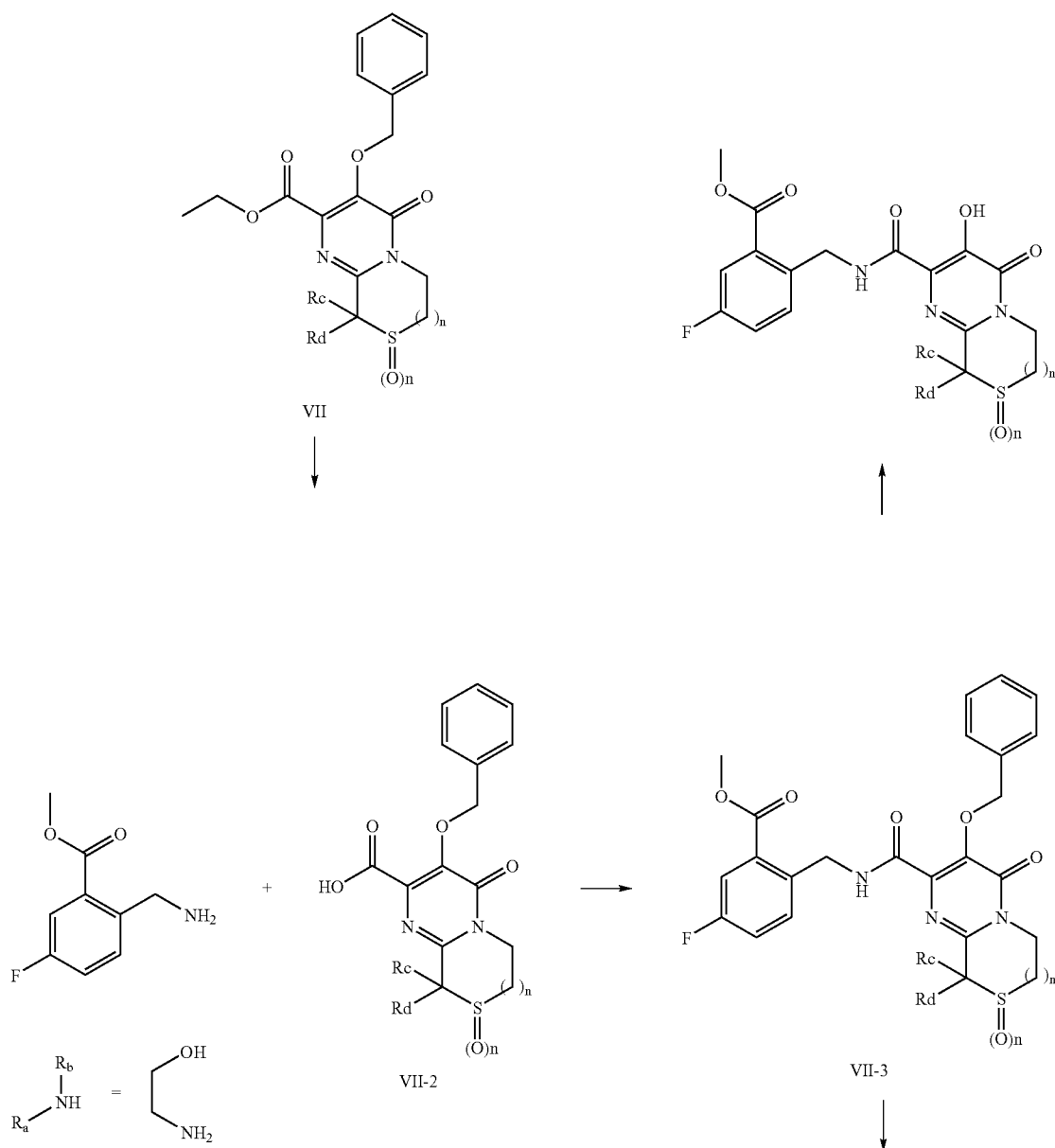
Scheme VII
