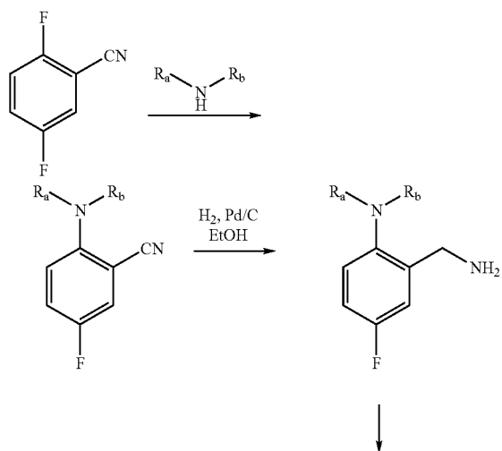
Scheme XII
