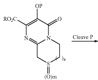
Scheme XVIII.
