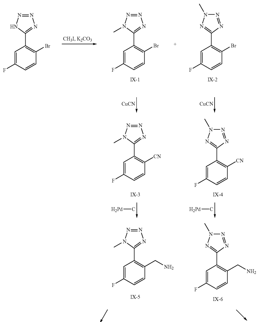
Scheme IX
