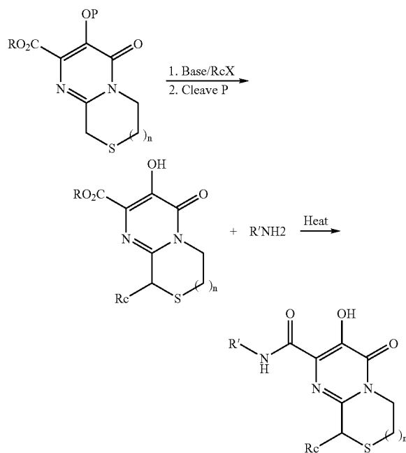
Scheme XVII.
