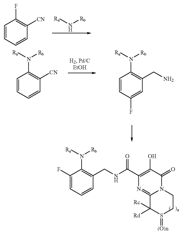
Scheme XIII
