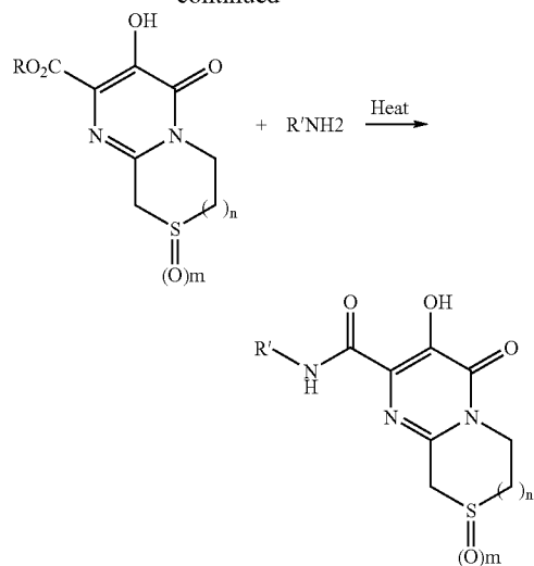
Scheme XIX.
