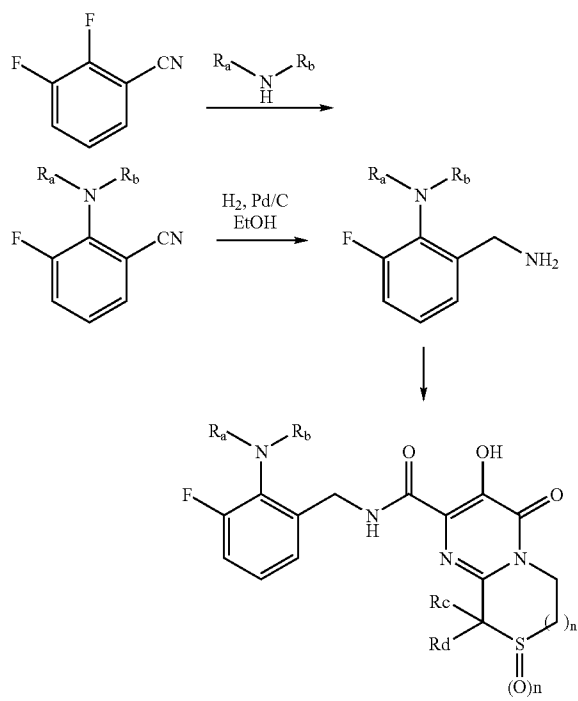
Scheme XI
