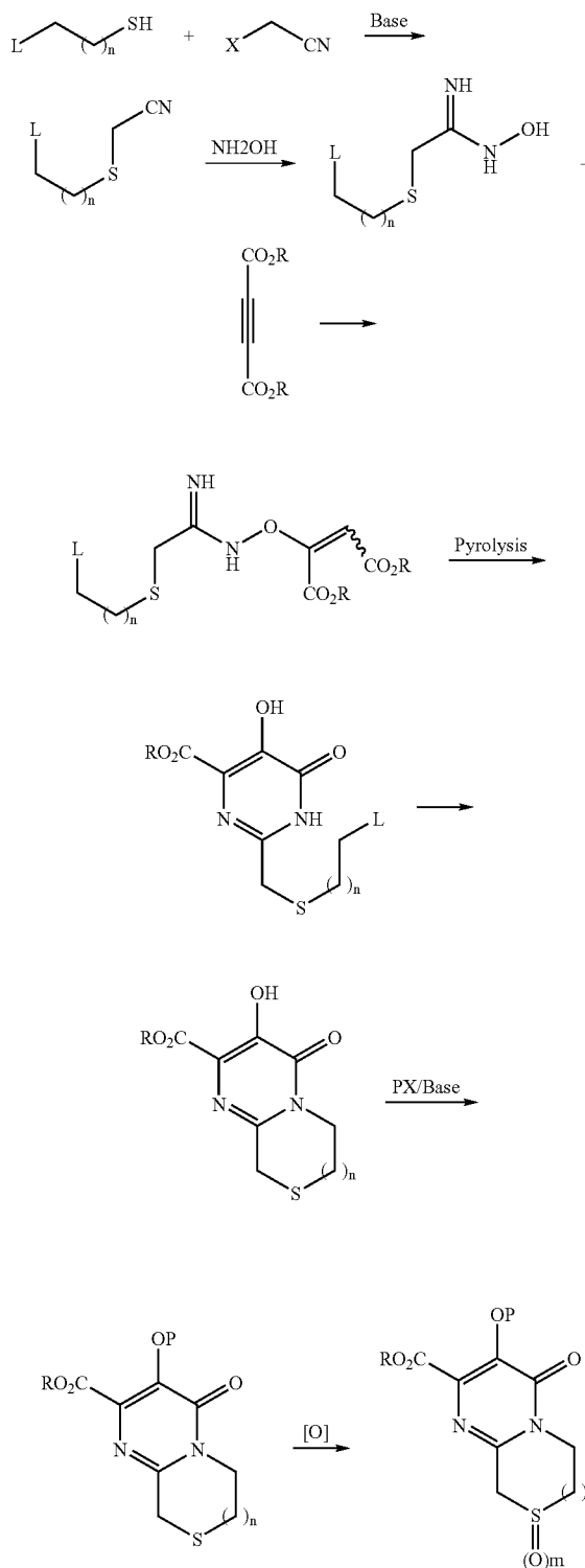
Chemical reaction scheme showing the synthesis of a pyrimidine derivative. The starting material is a pyrimidine-2,4,6-trione derivative with substituents R_c , R_d , and a sulfonamide group (O)_n . It is reacted with LiOH to form an intermediate. The intermediate is then reacted with a secondary amine R_a-NH-R_b to form the final product, which is a pyrimidine derivative with a modified side chain. Below the reaction, various structures for R_a-NH-R_b are provided, including: Morpholine N-methylamine N-methylsulfonamide Primary amine N-methylpiperazine N-methyl-2-hydroxyethylamine N-methyl-4-fluorophenylsulfonamide N-methylpiperazine N-methyl-2-aminoethylamine N-methyl-4-fluorophenylsulfonamide N-methyl-2-aminoethylamine
