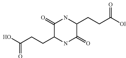
3-[5-(2-carboxy-ethyl)-3, 6-dioxo-piperazin-2-yl]-propionic acid
