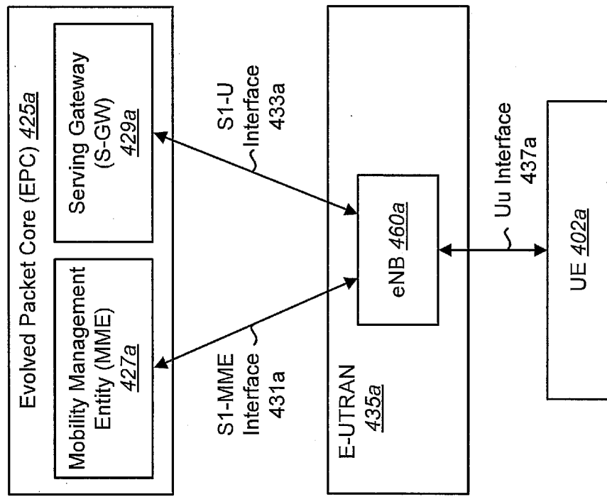
E-UTRAN Architecture 423
