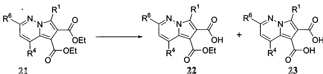
Scheme 5
