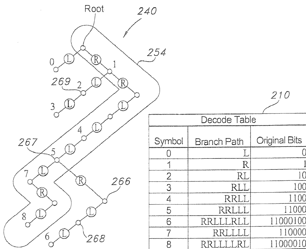
Decode Tree
