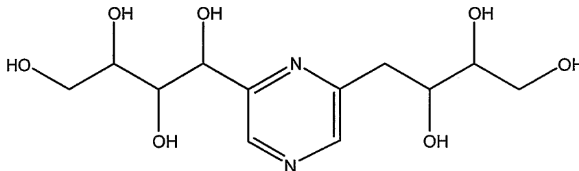
1-[6-(2,3,4-trihydroxybutyl)-pyrazin-2-yl]-butane-1,2,3,4-tetraol (2,6-deoxyfructosazine)
