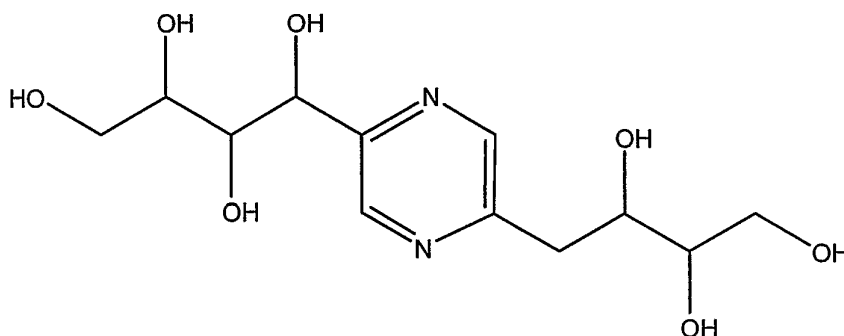
1-[5-(2,3,4-trihydroxybutyl)-pyrazin-2-yl]-butane-1,2,3,4-tetraol 15 (2,5-deoxyfructosazine)
