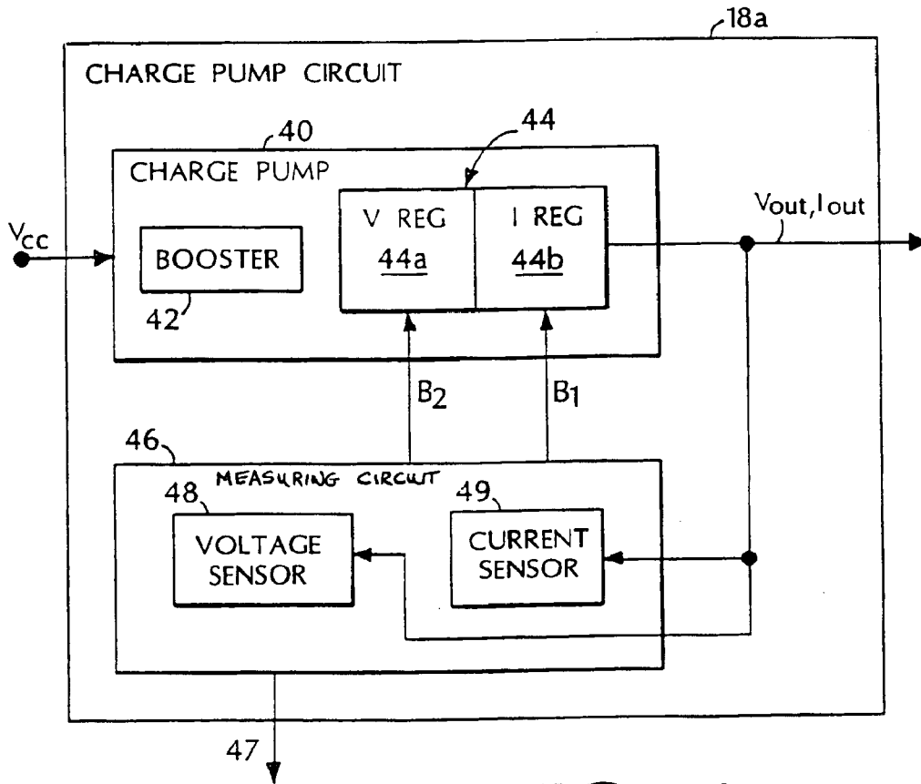
Access Line FIG. 4
