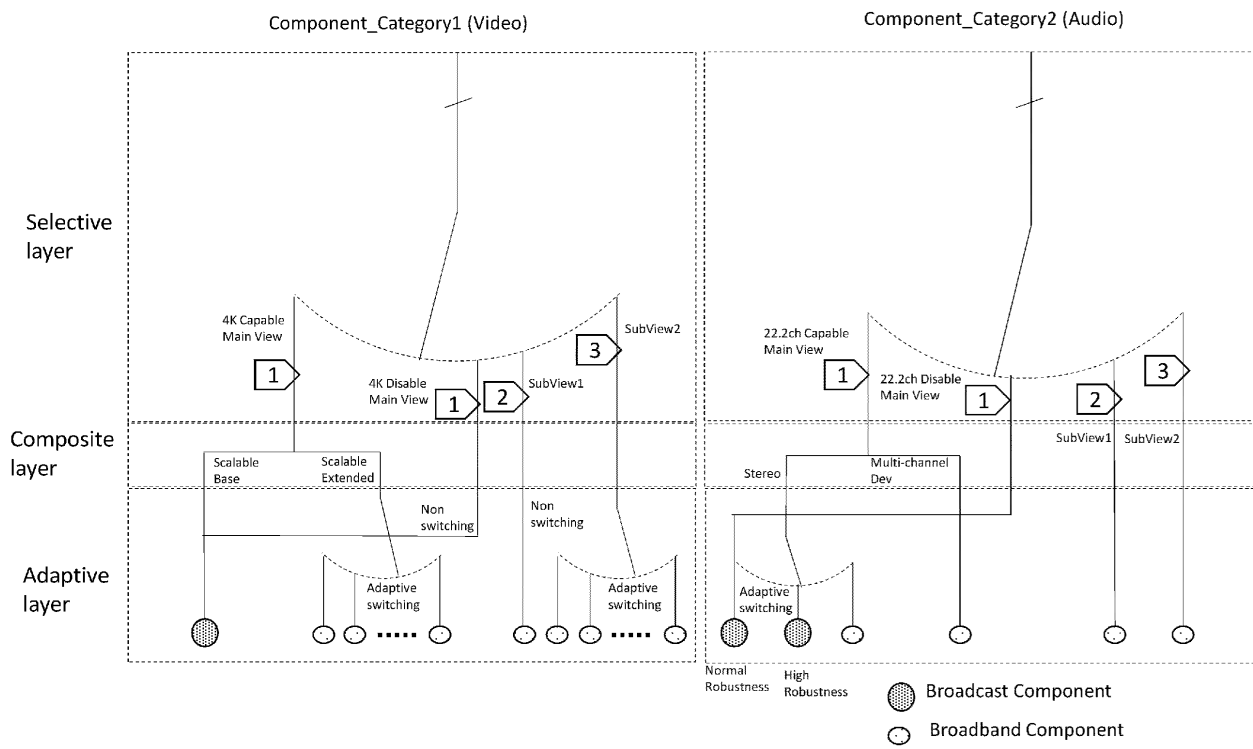
FIG. 35 MULTIVIEW COMPONENT LAYER MODEL
