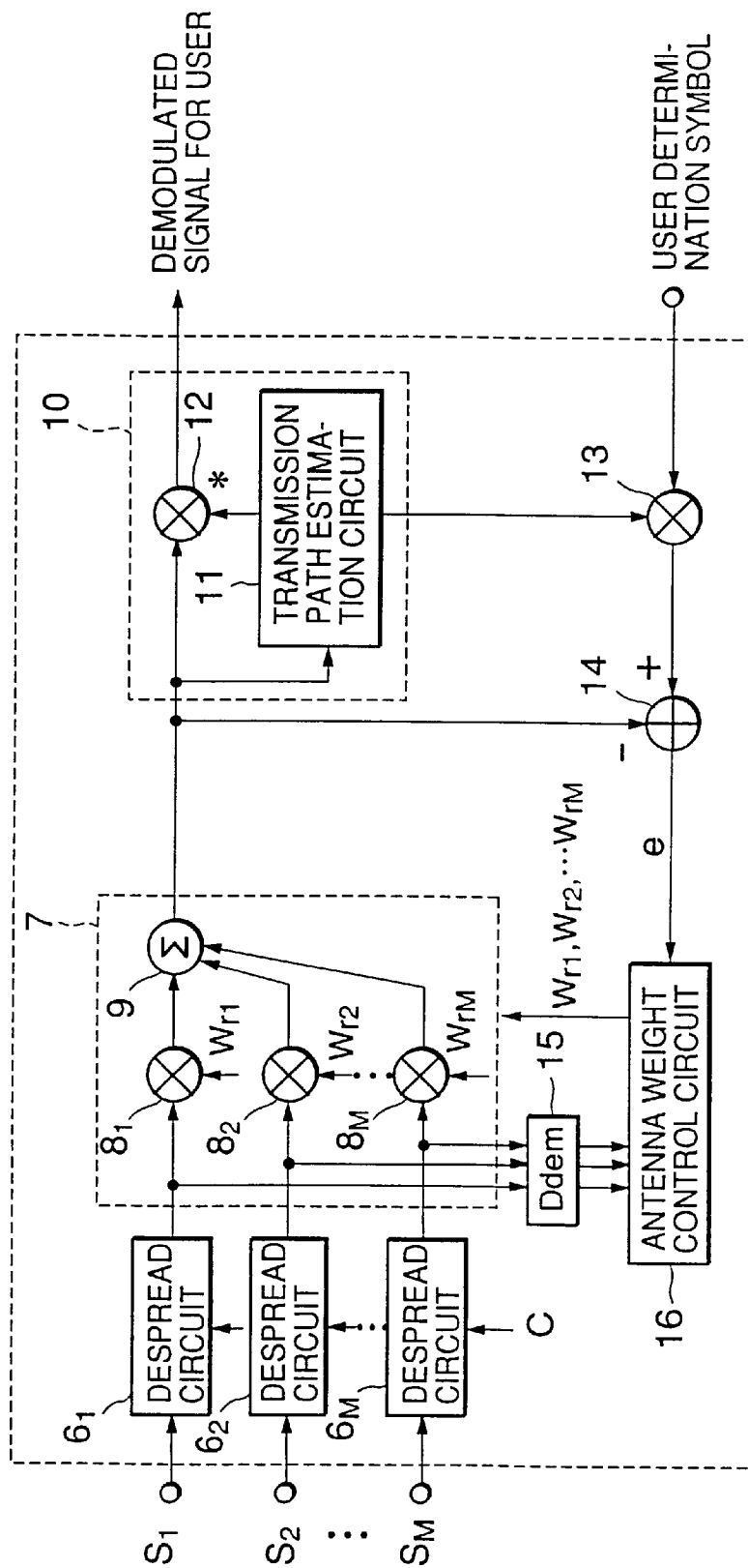
FIG.2 PRIOR ART
