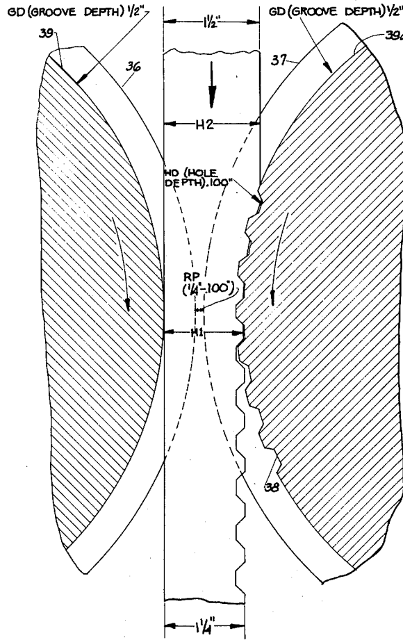
EDGING PASS - STAND 31
