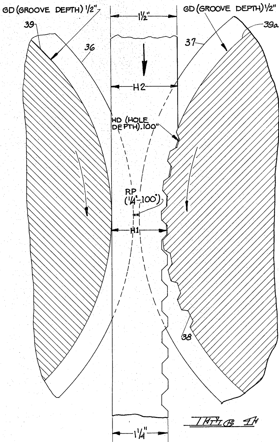
EDGING PASS - STAND 31
