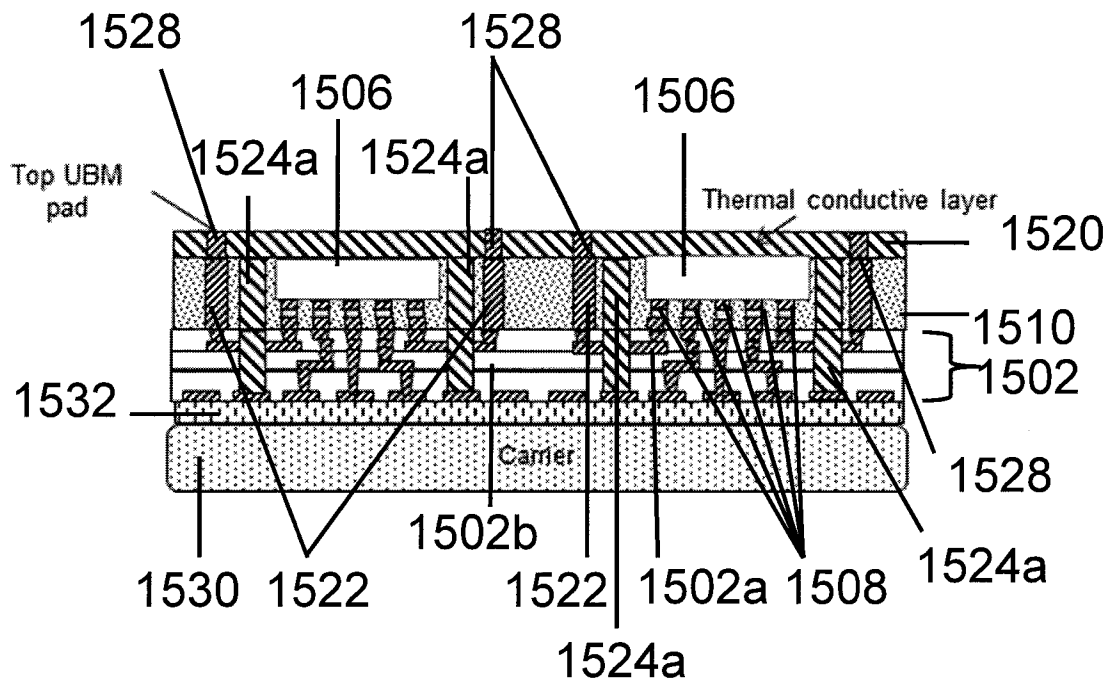
(g) Thermal conductive layer and Top UBM pad
