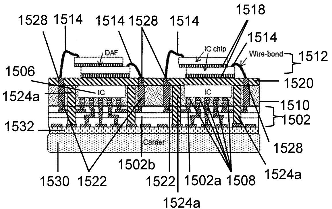
(h) Chip stacking & wire-bond
