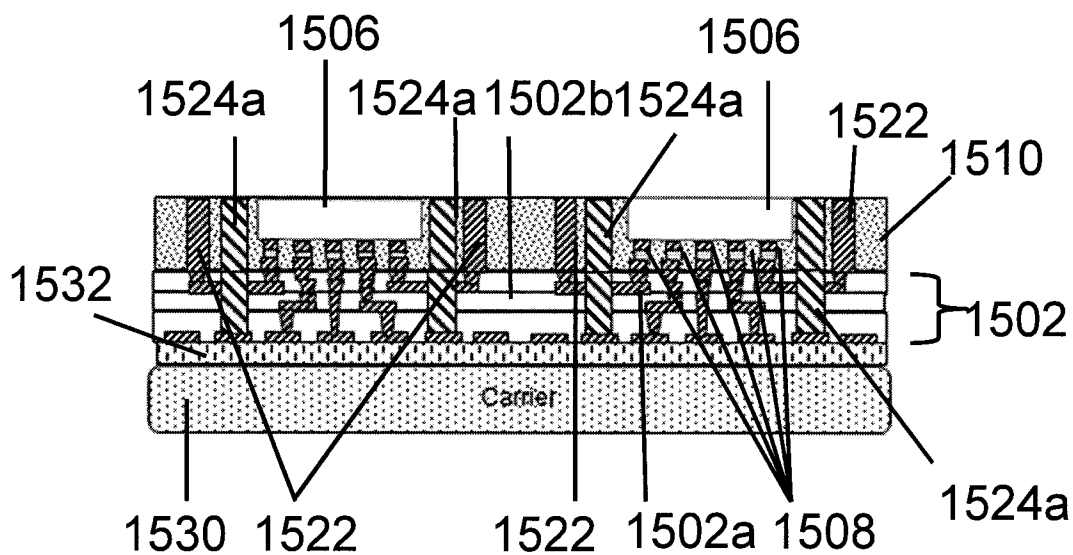
(f) Backgrind to expose TMI & thermal via
