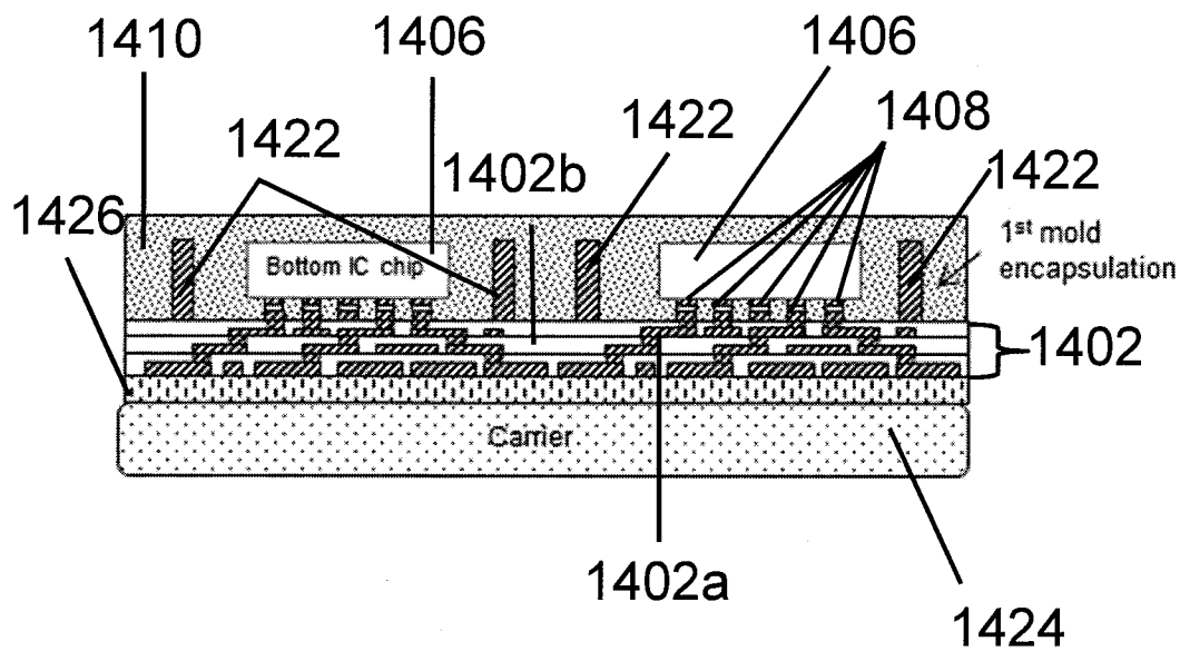
(e) Wafer level compression molding
