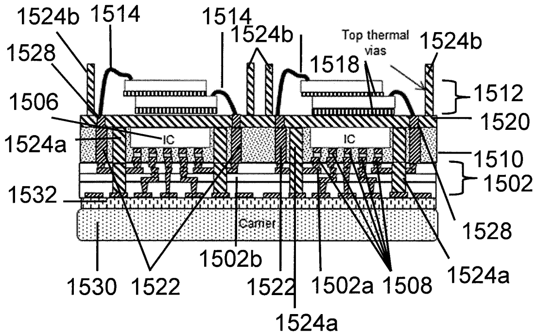
(i) Top thermal vias formation
