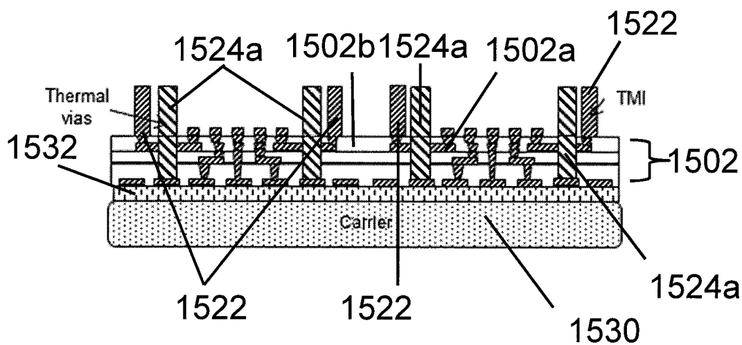
(c) Through mold interconnect (TMI) & thermal vias formation
