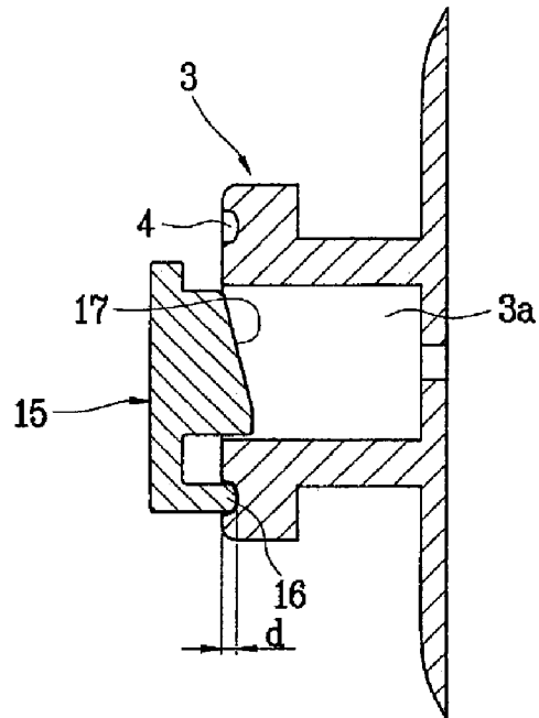
FIG. 2 Related Art
