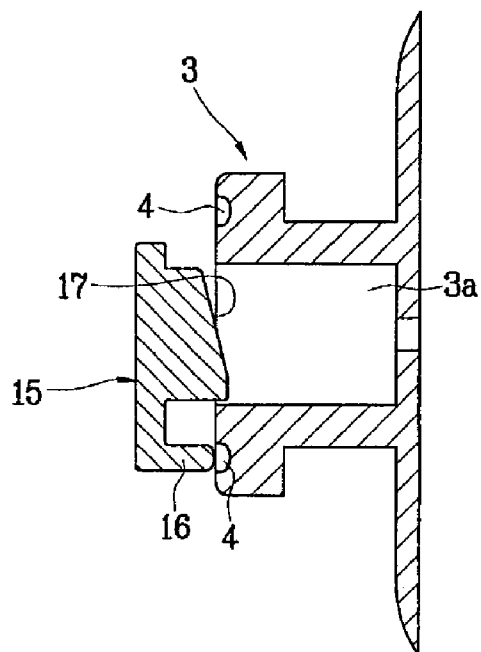
FIG. 3 Related Art
