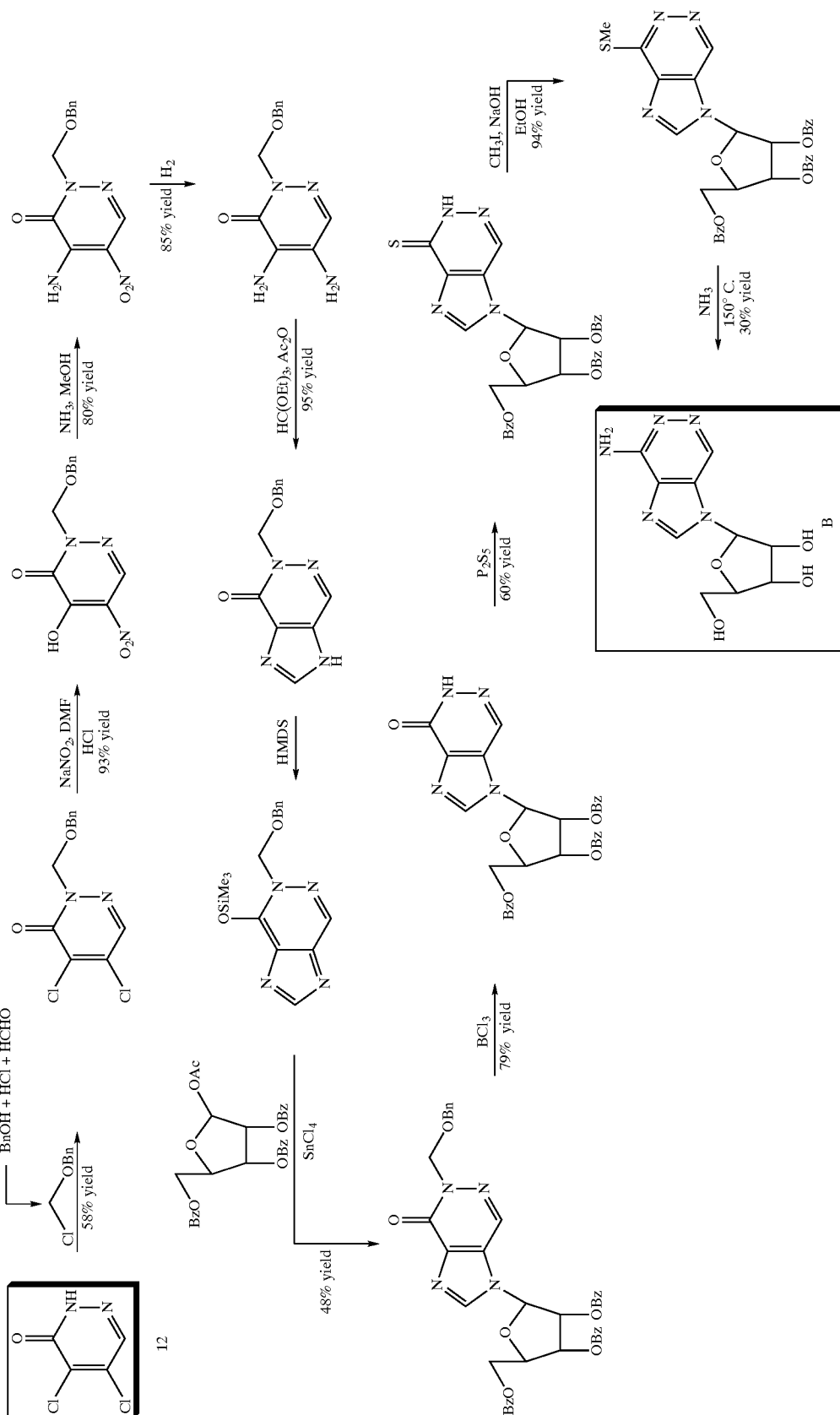
Scheme 9
