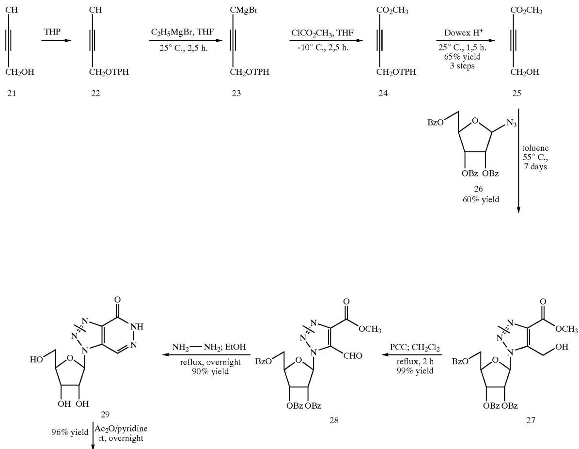
Scheme 12
