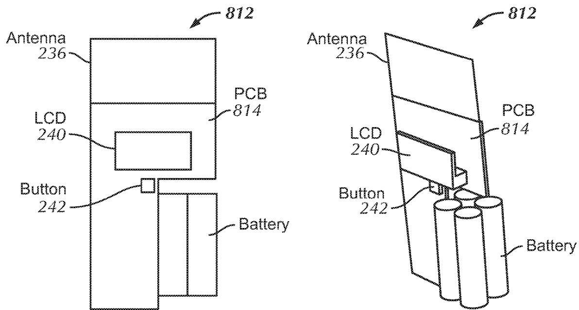
VT Board Front
