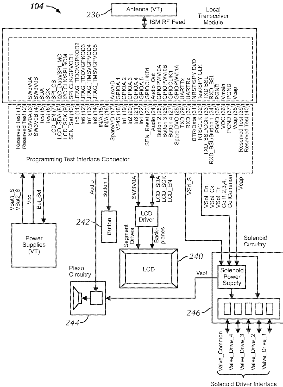
VT Top Level Block Diagram
