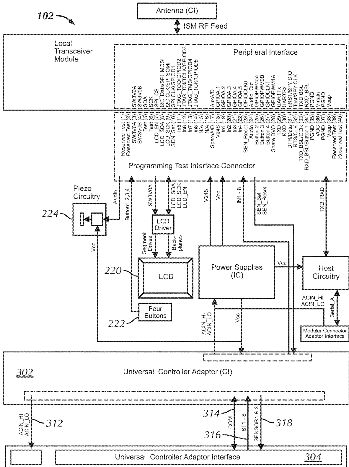
CI Top Level Block Diagram
